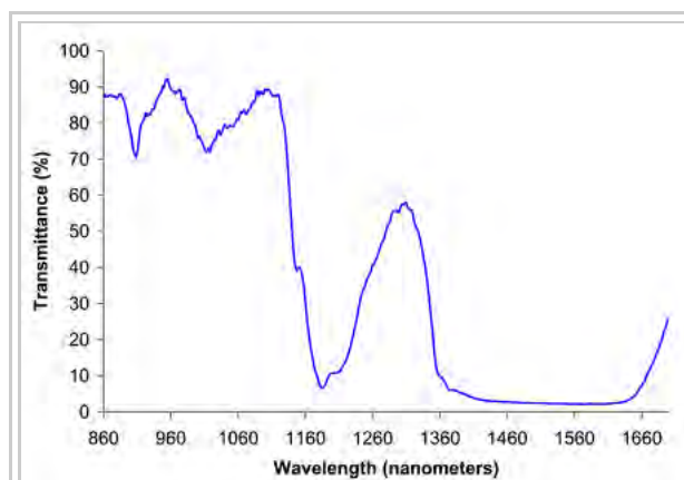
Near infrared spectrum of liquid ethanol.
