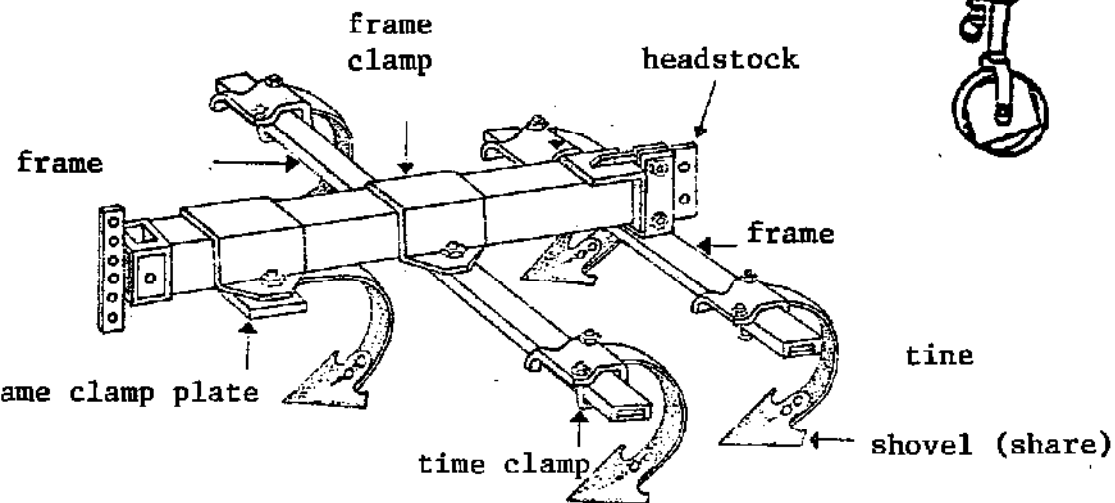
Five-Tooth Cultivator
