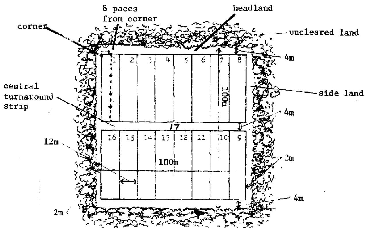
Well-planned field showing use of central turnaround strip. The turnaround strip is plowed last.
