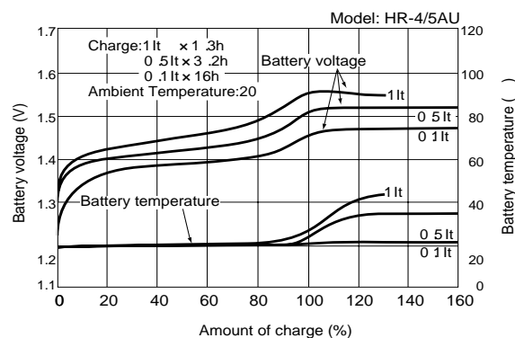
Fig.8 Charge temperature characteristics
