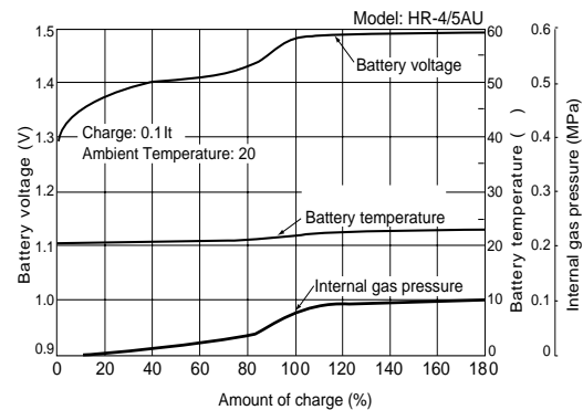
Fig.6 Charge characteristics
