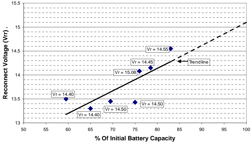
Array Reconnect Voltage (Vrr) vs. Battery Capacity Avg. of 4 and 8 Month Capacity Tests
