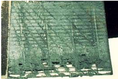
Figure 2: Electrolyte Stratification Causing Negative Plate Grid Deterioration
