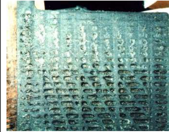
Figure 3: Gas Pocket Marks On Negative Plate
