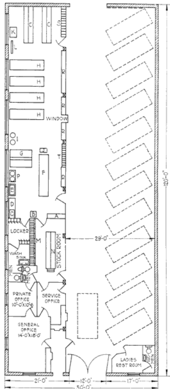
Fig. 141. Shop Layout
