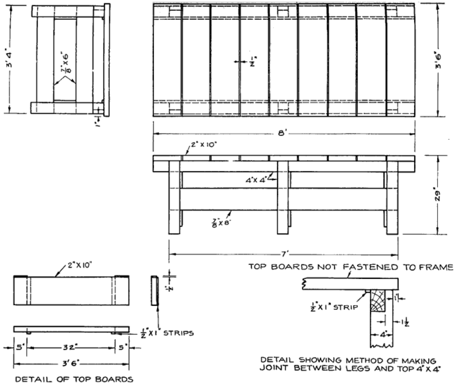
Fig. 67. Working Drawing of Eight Foot Charging Bench
