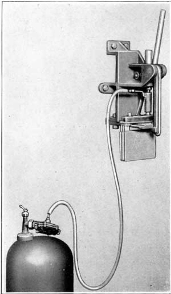
Fig. 248. Special Prest-O-Lite Peening Press
