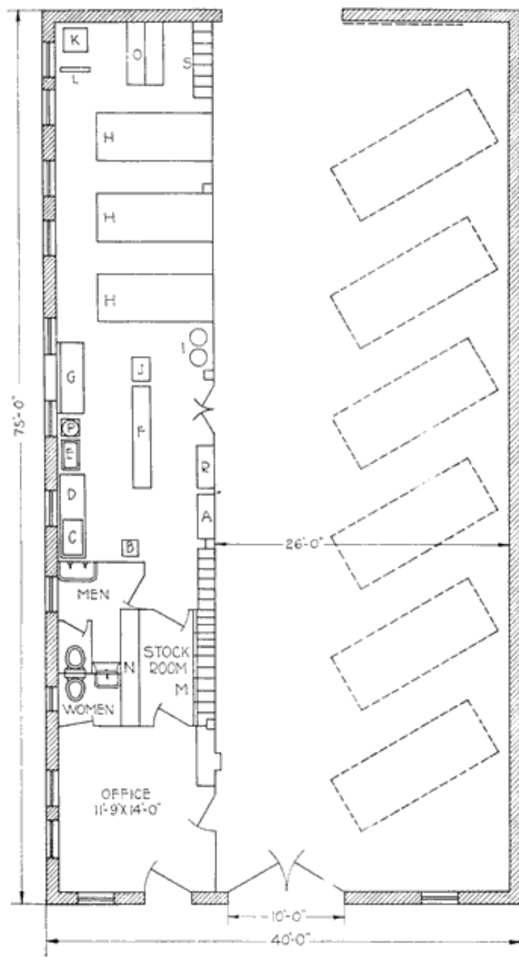
Fig. 138. Shop Layout
