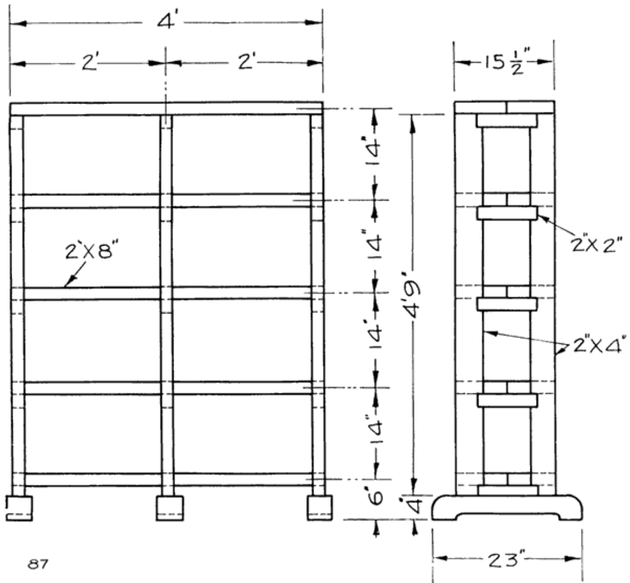
Fig. 87. Working Drawing of Rack for Repaired Batteries, New Batteries, Rental Batteries, Batteries in Dry Storage, Etc.
