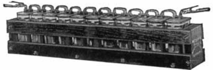
Fig. 170. Westinghouse Radio "B" Battery, Type M
