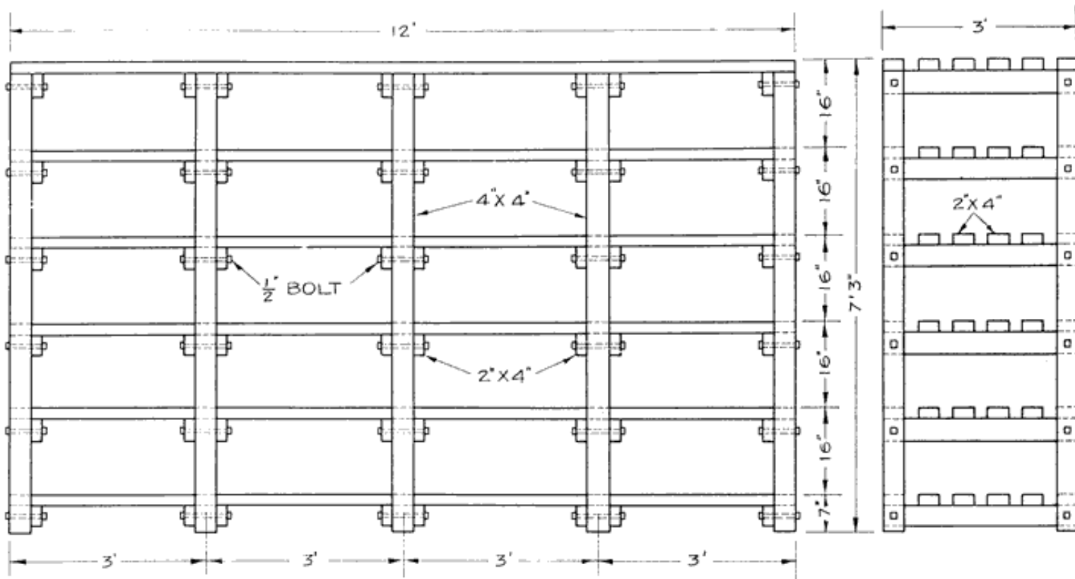
Fig. 85. Working Drawing of Receiving Rack
