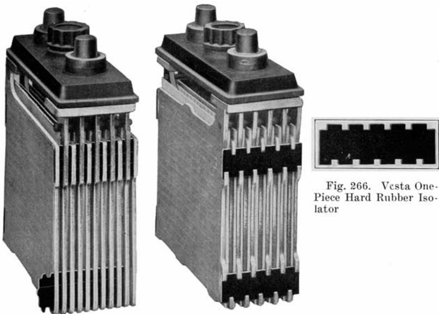
Fig. 265. Vesta Elements. Showing Old Three-Piece Celluloid Isolator and New One-Piece Hard Rubber Isolator
