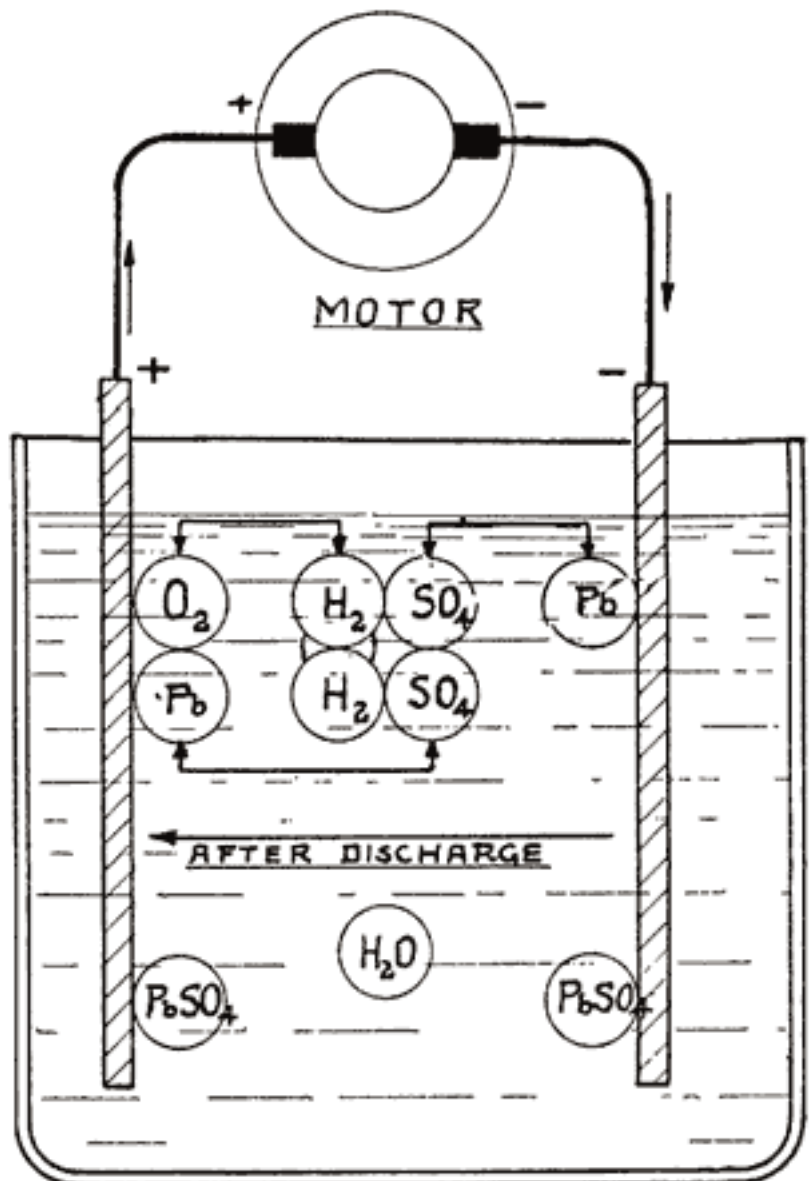
Chemical Action in a Storage Cell During
