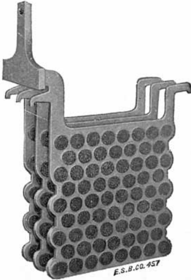
Fig. 325. Manchester Positive Plates
