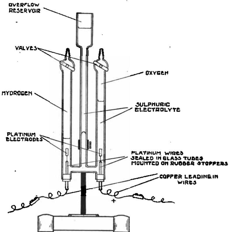
FIG. 1. GROVE'S GAS CELL, CHARGED.
