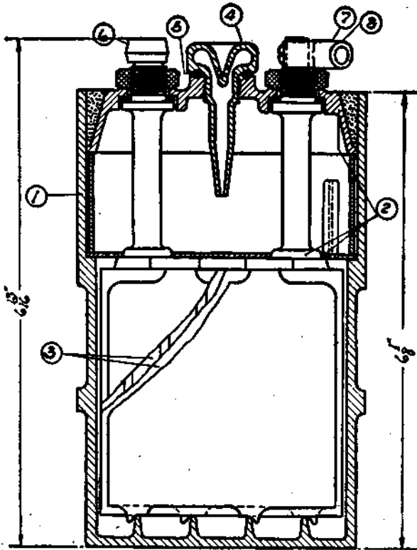
1 Rubber Jar. 2 Plate Strap. 3 Wood and Rubber Separators 4 Vent Plug. 5 Vent Gasket 6 Inter-cell connector 7 Terminal lug 8 Hole for "Sweating in" wires
