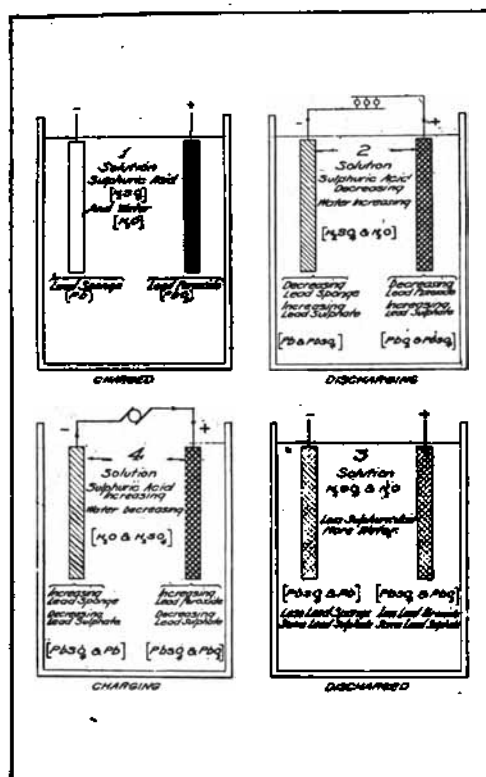
FIG. J. PICTORIAL OUTLINE OF CHEMICAL ACTION IN LEAD STORAGE BATTERY.
