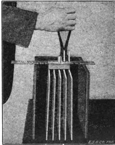
FIGURE III. DEVICE FOR PLATE GROUPING.
