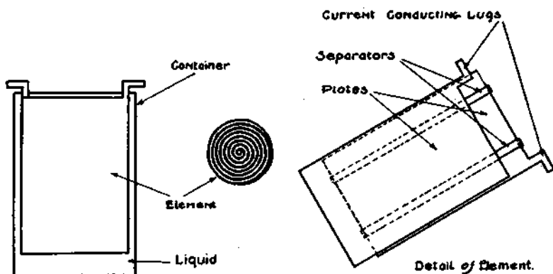
Fig. II. Planté's Cell.
