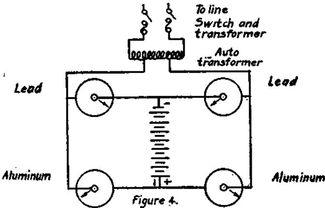
Electrolytic Rectifier Connections for using both pulsations of AC.
