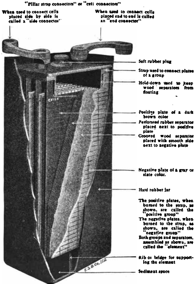
One 9-MV "Exide" Cell, Showing Parts Used and Method of Assembly
