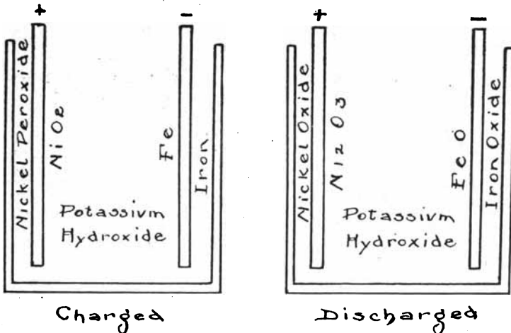
PICTORIAL EXPLANATION OF CHEMISTRY OF NICKEL-IRON CELL.
