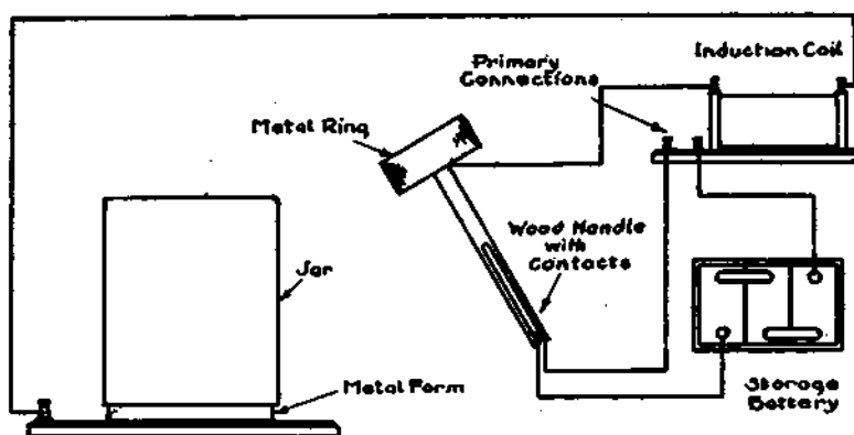
Connections for Jar Tester
