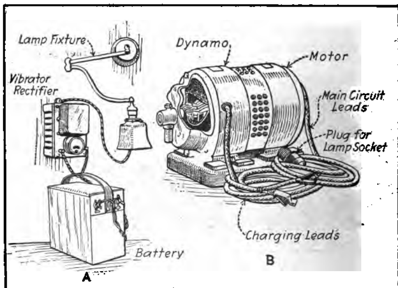
Fig. 41.—Devices for Rectifying Alternating Current. A—Vibrator Type Rectifier. B—Small Rotary Converter Set.
