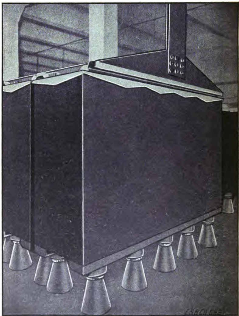
Fig. 8.—Type of Electric Storage Battery Company Cell for Stand-by and Booster Service.
