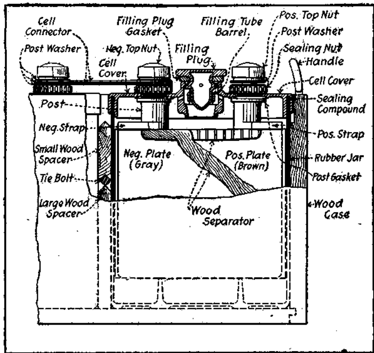
Fig. 25.—Exide Double Seal Bolted Connector Type Battery.
