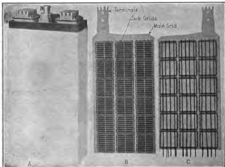
Fig. 80.—The Edison Submarine Boat Battery and Two of the Plates Showing Use of Sub-Grids.
