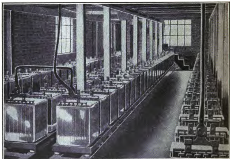
Fig. 68.—Typical Isolated Lighting Battery for Medium-Capacity Plant.
