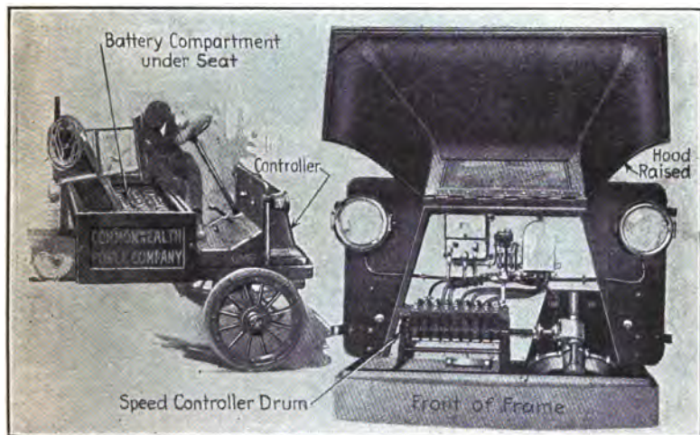
Fig. 66.—View at Left Shows Battery Location; at Right the Controller Compartment is Opened to Show Accessibility of Wiring.
