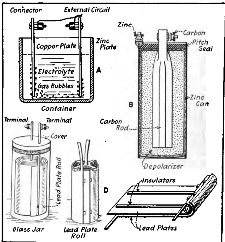
Fig. 1.—Types of Chemical Producers. A—Elementary Primary Cell. B—Construction of Dry Cell. C—Simple Form of Secondary Battery. D—The Lead Plate Roll and How It is Made.
