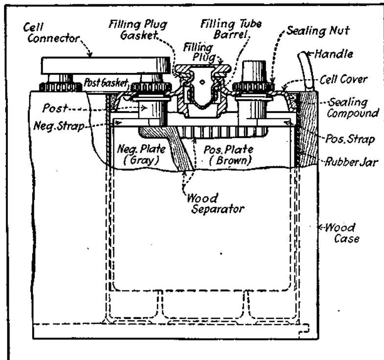
Fig. 26.—Exide Single Seal Burned Connector Type Battery.
