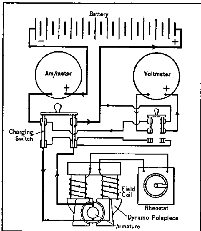
Fig. 37.—Battery-Charging Outfit, Having Field-Coil Rheostat.
