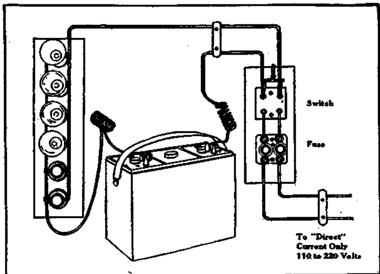
Fig. 48.—Charging Storage Battery From Direct Current With the Lamp-Bank Regulation.
