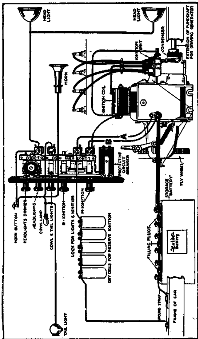
Fig. 55.—The Delco Ignition, Motor-Starting and Car-Lighting System.
