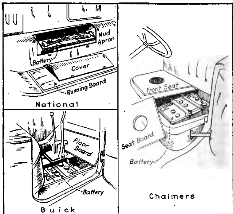
Fig. 57.—How Storage Batteries are Installed in an Automobile When Used for Starting and Lighting Current.
