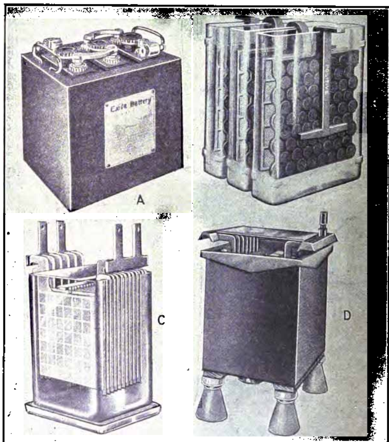
Fig. 5.—How Storage Batteries Differ in Construction. A—Automobile Type. B—Couple Type. C—Glass Jar, Open Type. D—Large Wooden Tank Type for Heavy Duty Service.
