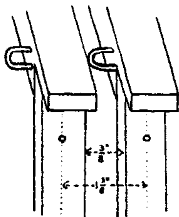
Figure 6. Staple-spaced frame
