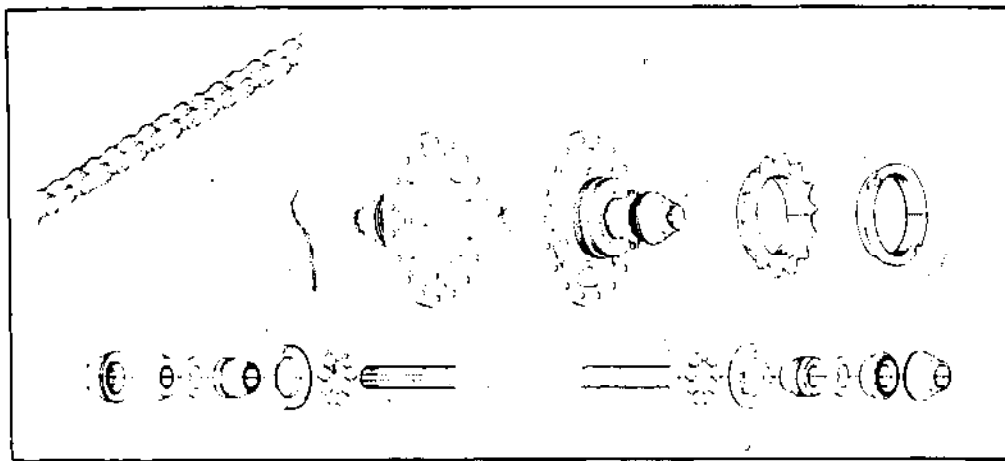
Fig. 2-26 Shimano Dura-Ace 10 chain and track model hub.
