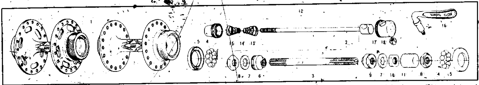
Fig. 5-4. Shimano 600 rear hub for freewheel with quick release. Parts are: (1) hub shell—large and small flange models shown, (2) complete axle set, (3) axle, (4) steel ball, (5) dust cap, (6) cone, (7) key washer, (8) lock nut, (9) cone, (10) lock nut, (11) spacer, (12) complete quick release unit, (13) skewer, (14) volute spring, (15) nut for skewer, (16) cam lever, (17) body cam lever and (18) cap nut.
