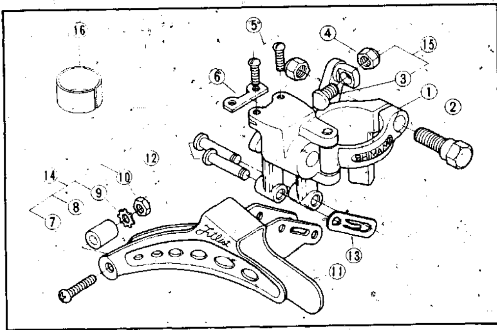
Fig. 5-52. Shimano Tittist front derailleur. Parts are: (1) mechanism unit lower inlet type, (2) clamp bolt, (3) cable fixing bolt, (4) cable fixing nut, (5) adjusting bolt, (6) adjusting plate, (7) chain guide spacer bolt, (8) chain guide spacer, (9) toothed lock washer, (10) nut, (11) chain guide, (12) pin A, (13) clip A, (14) chain guide spacer and bolt set, (15) cable fixing bolt and nut set and (16) 1-inch bushing.
