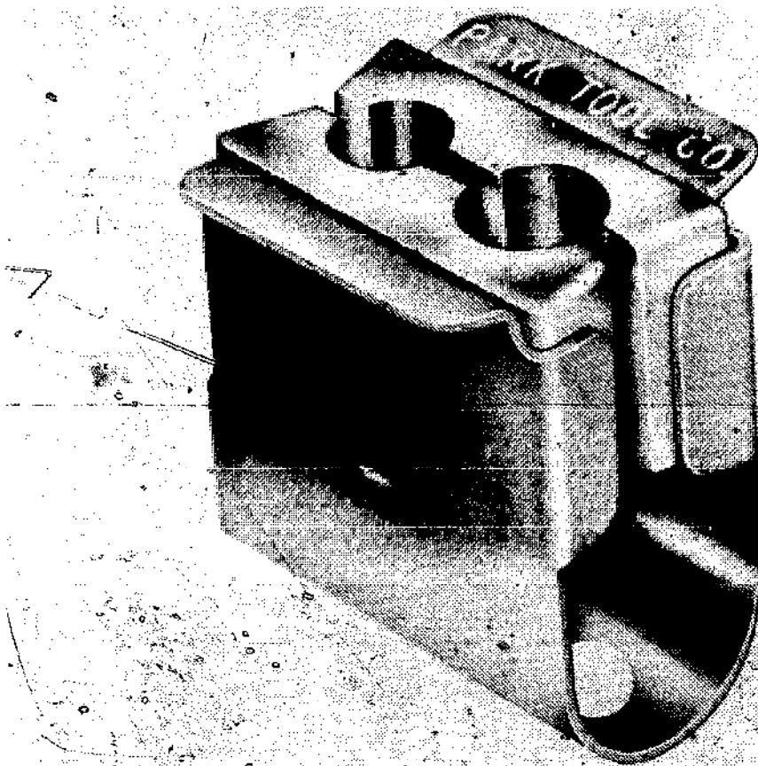
Fig 5-7 Park axle vise
