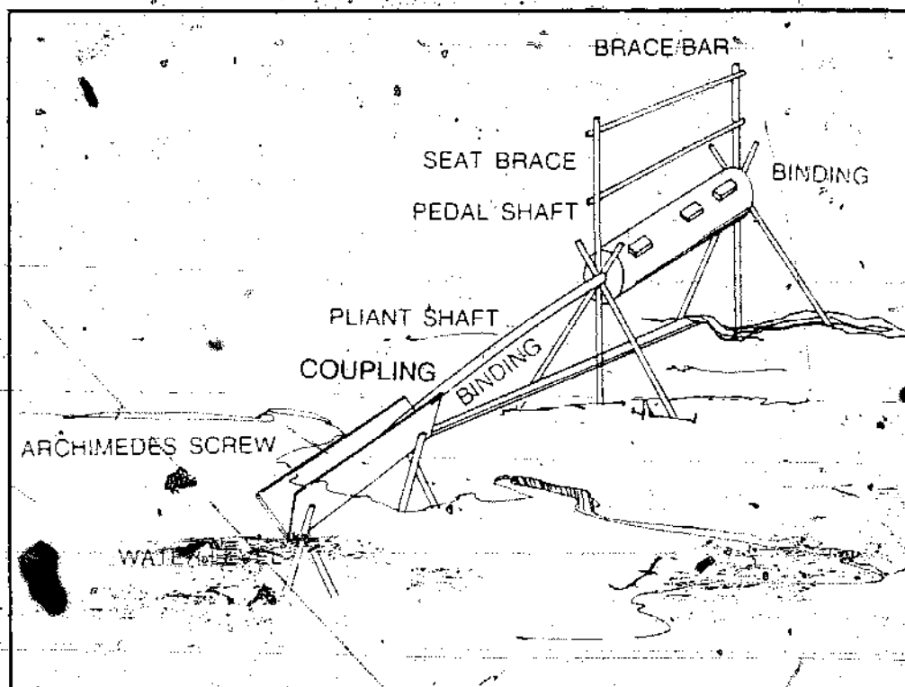
Fig. 17-9 A pedal-driven Archimedes screw that is designed with a slope of 30 degrees and a length of 20 feet.
