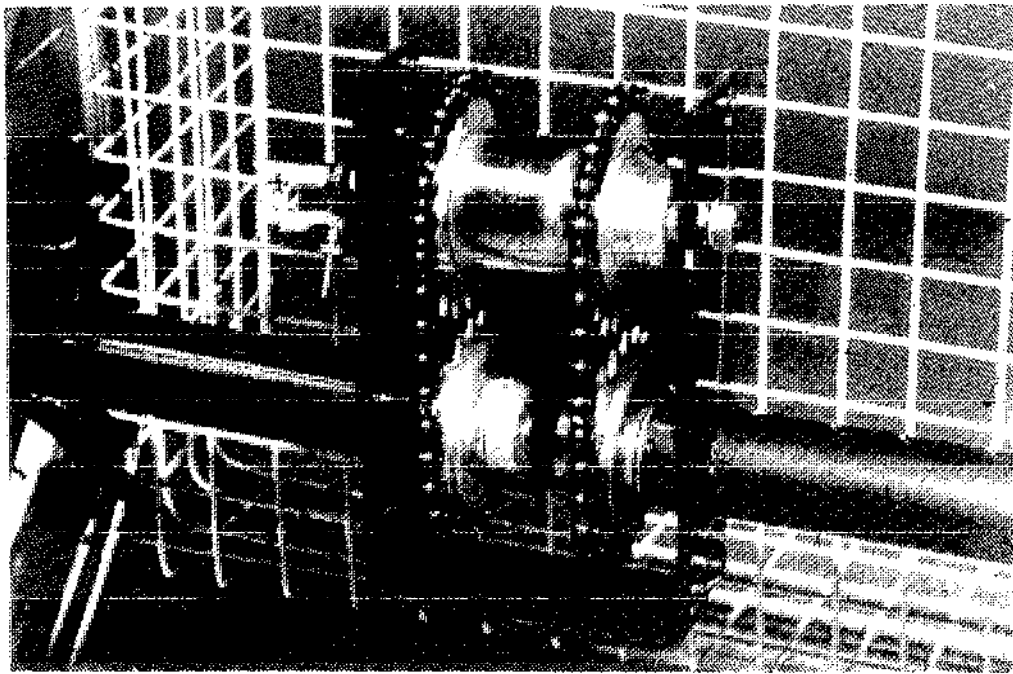
Fig. 11-10. Gobby dual-drive unit with three-speed hub.
