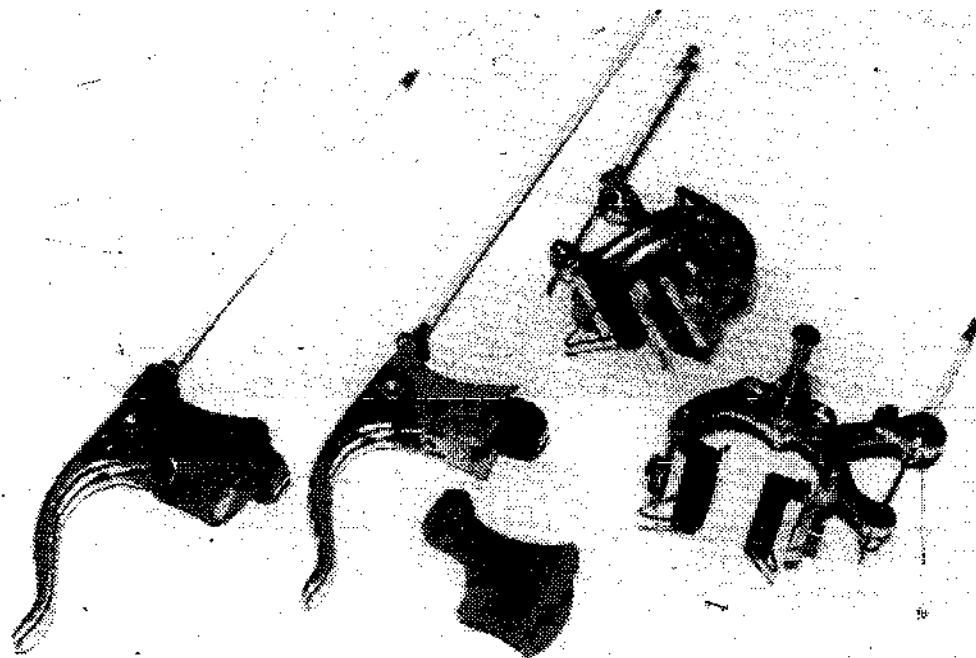
Fig. 2-21. Zeus high quality side-pull caliper brakes.
