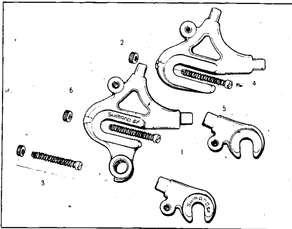
Fig. 2-14 Shimano Dura-Ace Model NB-100 drop-outs: (1) front fork end set, (2) rear fork end set with adjusting set, (3) adjusting bolt, nut and spring, (4) adjusting bolt, (5) adjusting spring and (6) adjusting nut.
