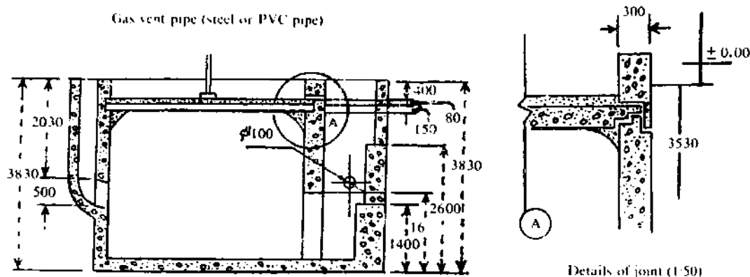
Fig. 51. Sectional view.
