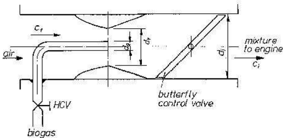
Fig. 6.3: Venturi mixer with a single gas inlet nozzle.
