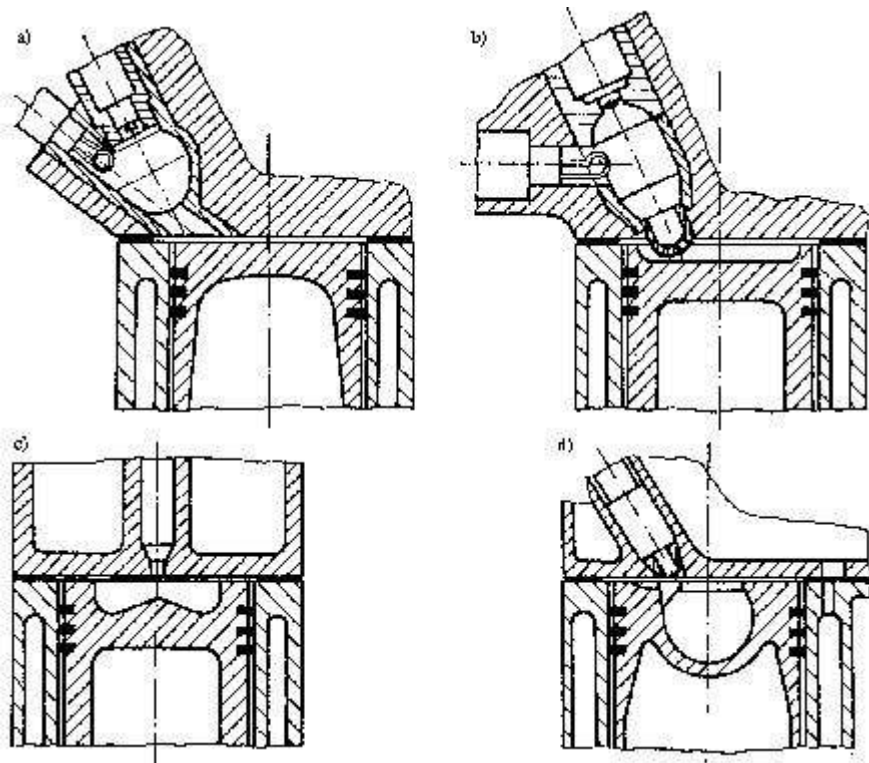
Fig. 3.12: Different combustion chamber forms and methods of fuel injection.
