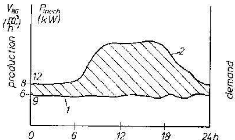
Fig 7.3: Daily profiles: 1 biogas and potential power production, 2 power demand, \\\shortage in biogas/// power production. Power shortage to be compensated by other fuels/energies in isolated operation or by purchase of electric power from grid in parallel operation.
