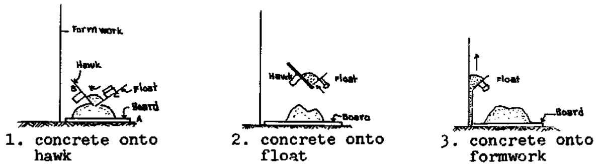
Fig. 17 Trowelling the Concrete onto the Formwork
