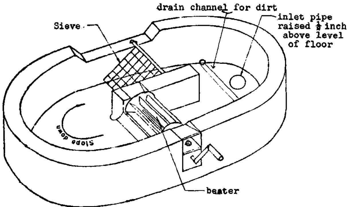
Slurry-mixing machine
