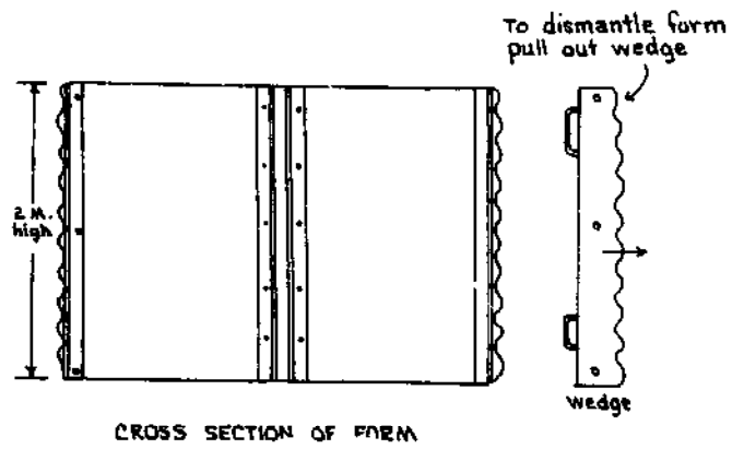
Fig. 18 Standard Formwork for 10 cubic meter tank
