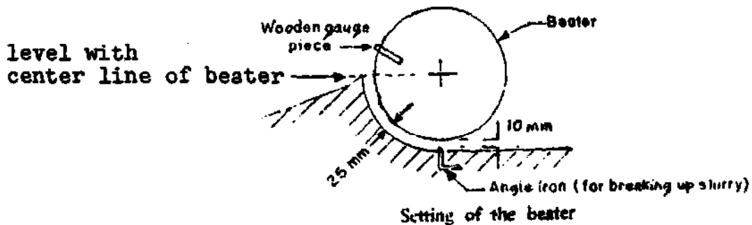
Slurry-mixing machine
