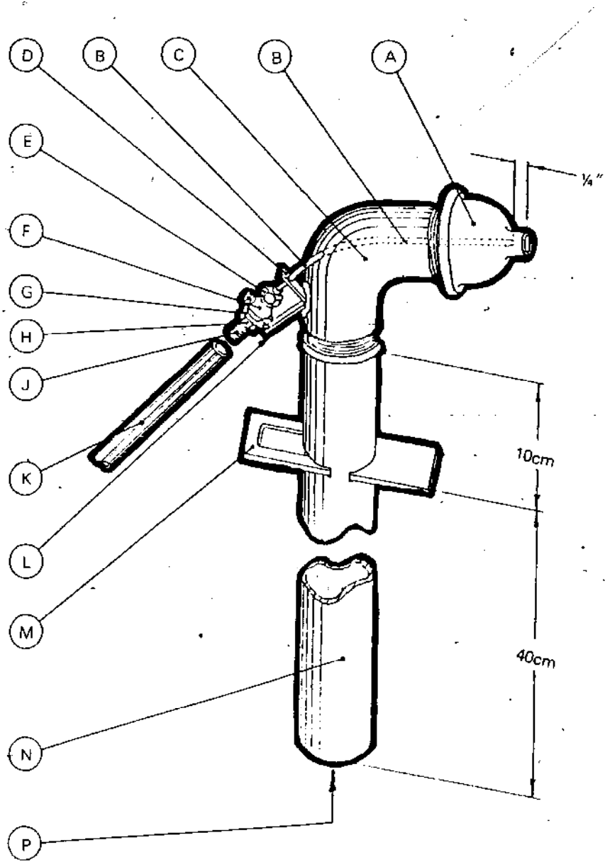
Fig. 67 Oil burner construction.
