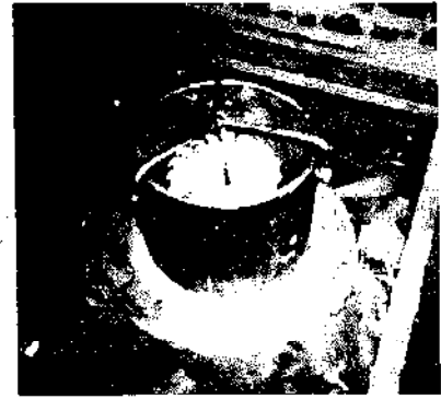
Wax pattern being held in place before pouring refractory slurry, Colombia.
