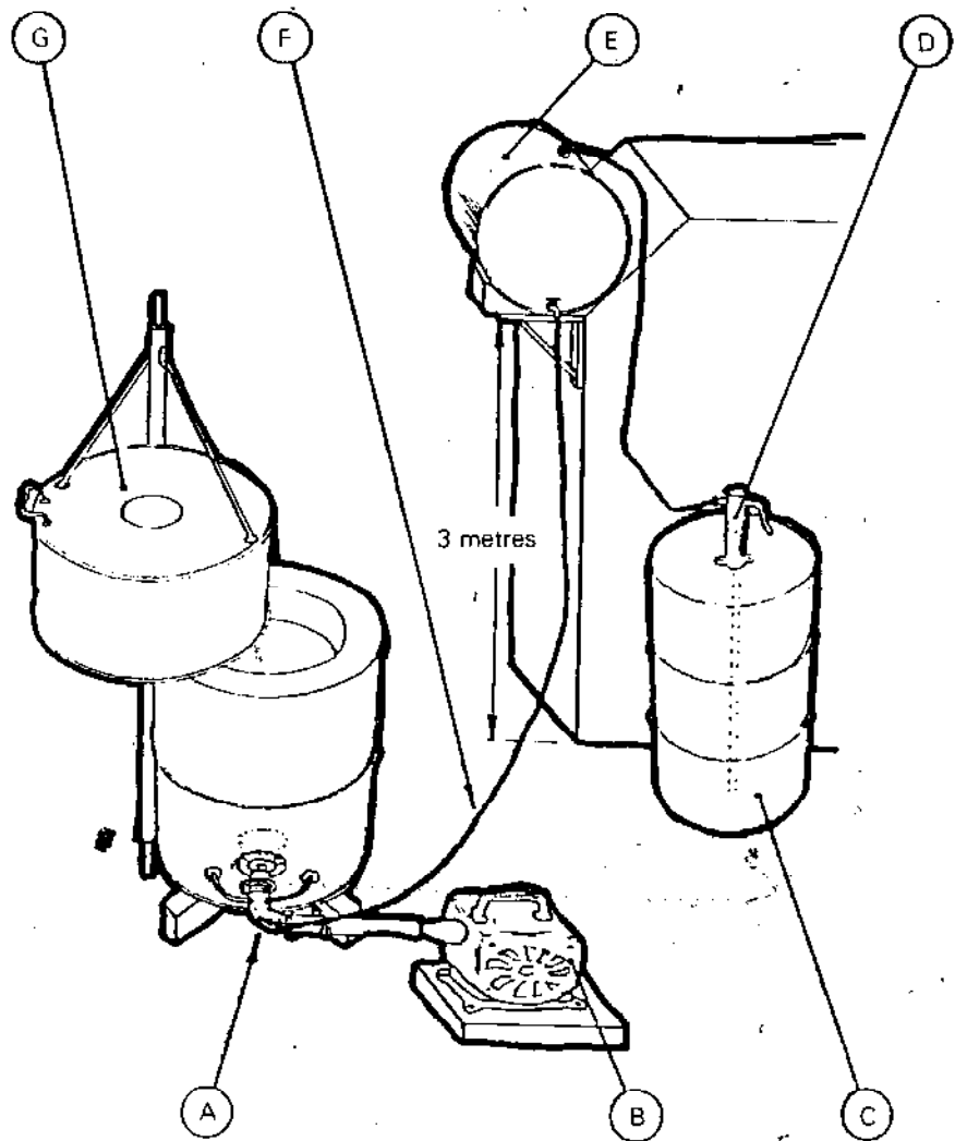
Fig. 66 Oil-fired furnace system.
