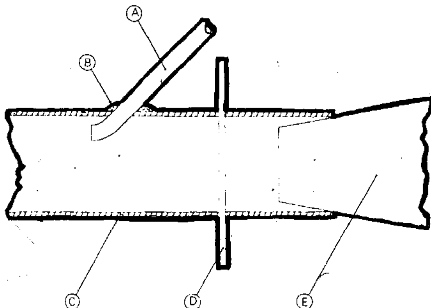
Fig. 65 Gas pipe entry detail.
