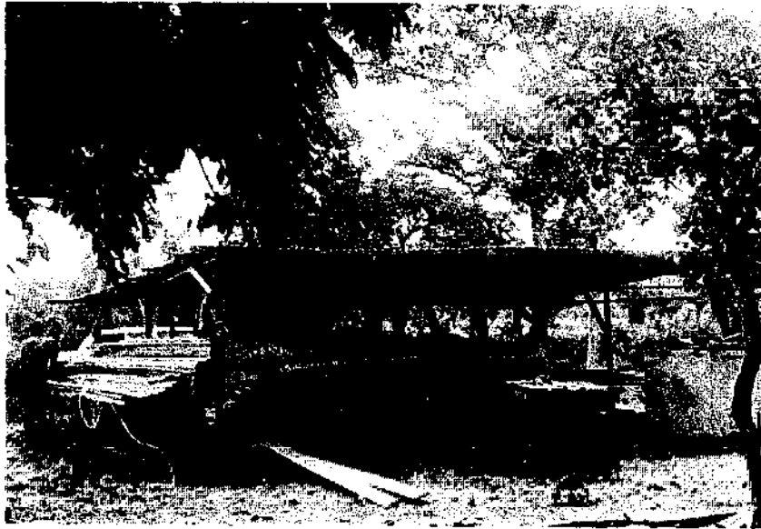
Fig.19 Chantier artisanal Fig.19 Artisanal boatyard
