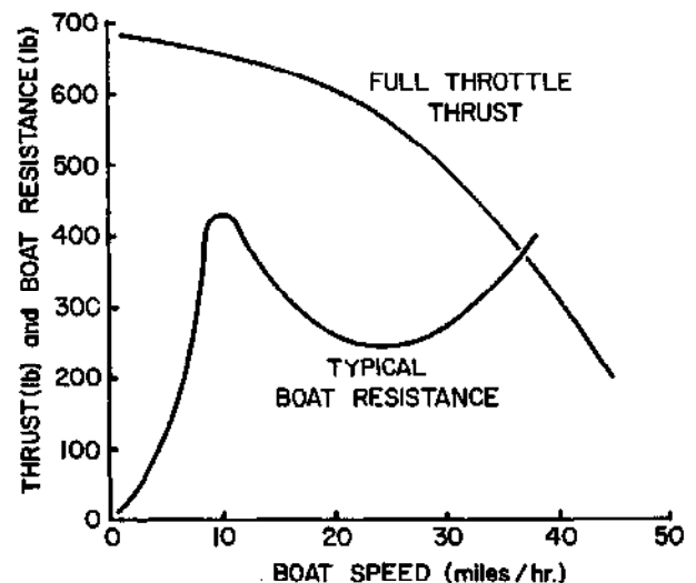
Fig. 4. Resistance of typical 17-ft boat with load of four passengers. Full throttle thrust curve is net driving thrust of an 80-hp engine using 10-in diameter x 10-in pitch propeller.
