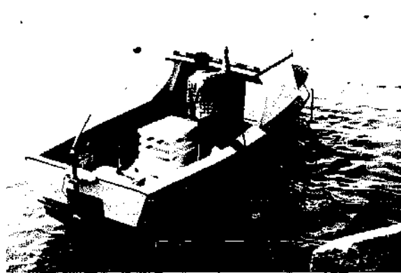
Fig. 1. Type A boat: a 28-ft, single-hull, diesel boat with removable propeller for shallow draft.
