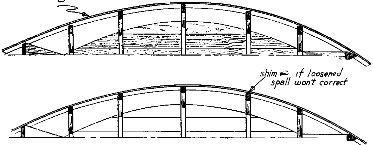
fairing batten
