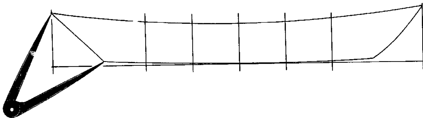
11(b). Take the length of the transom from the profile drawing. The transom is foreshortened in the other two views.
