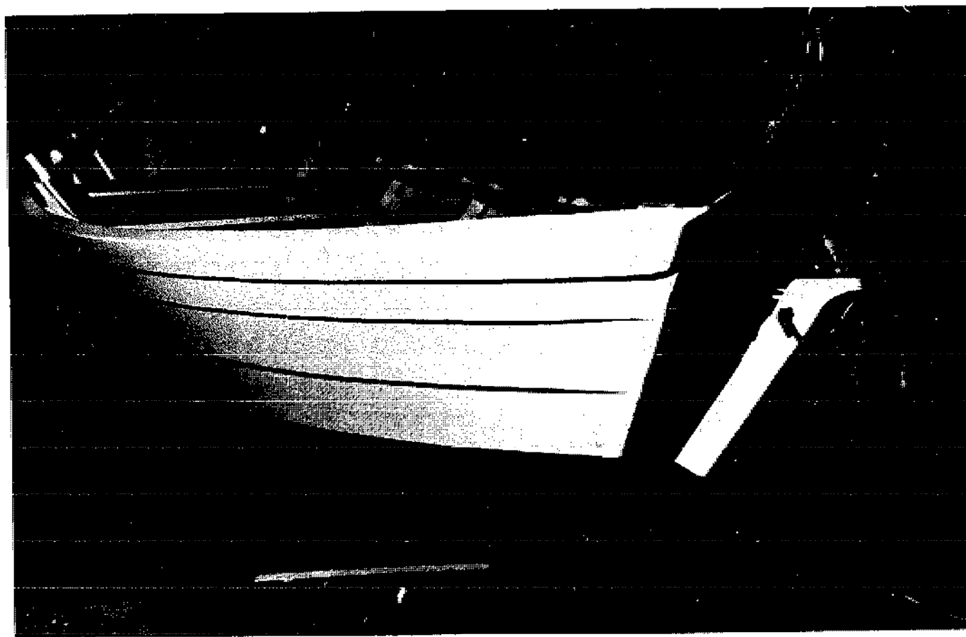
A Lowell-Coast Guard 15-foot fisherman's dory ready for delivery.
