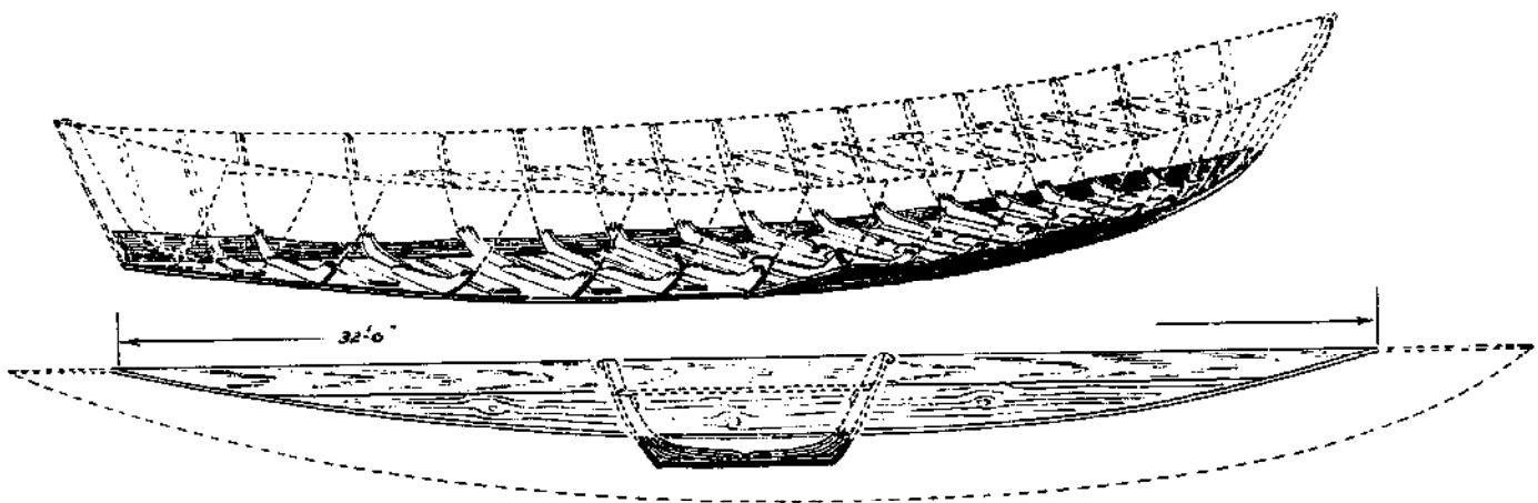
An ancient batteau bottom raised from Lake George in 1960. The boat's overall length was possibly 36 feet. The reconstruction (dotted lines) is based on the draft of the 1776 colonial batteau shown in Howard I. Chapelle's American Small Sailing Craft .
