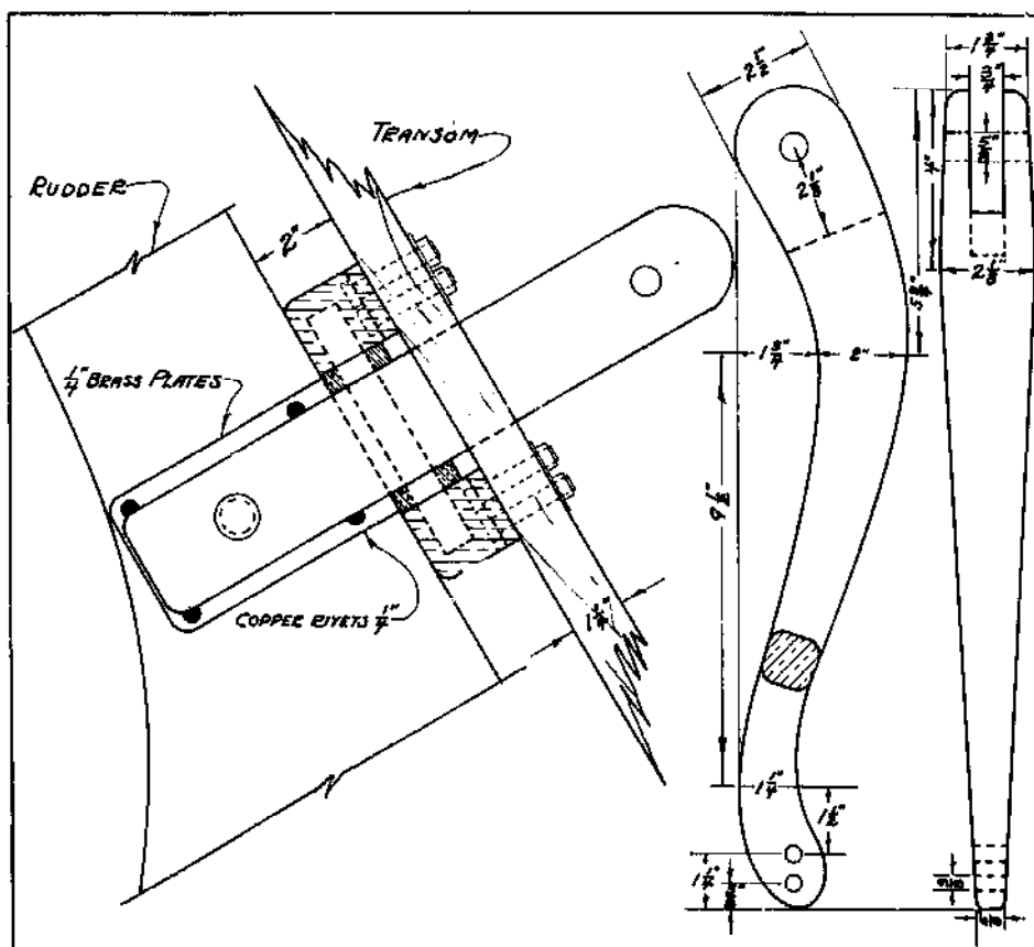
The tiller bearing assembly in place.
