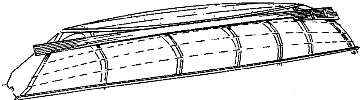
28(a). To spile a dory garboard. Clamp or tack a suitable spiling batten through the plank space to be filled. If the adjusted compass won't reach the batten in some places, tack on some cardboard to increase the batten's width locally.
