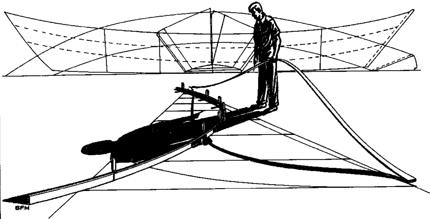
1. Lines and the laydown.
