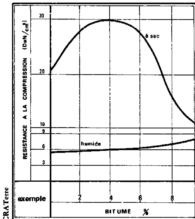
FIGURE 289 : RESISTANCE A SEC, RESISTANCE HUMIDE
