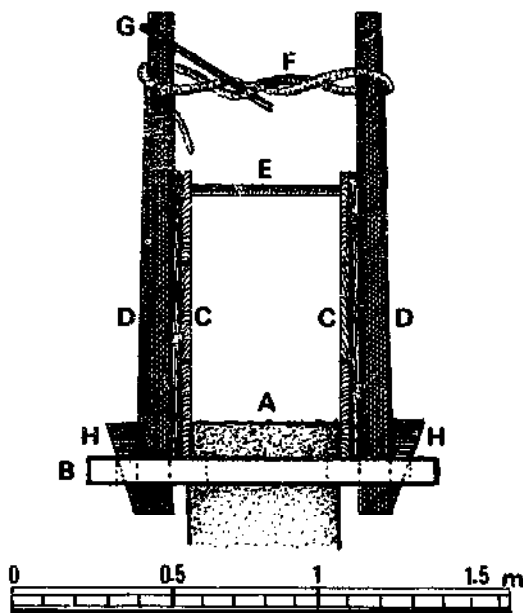
FIGURE 8 : BANCHE LYONNAISE
