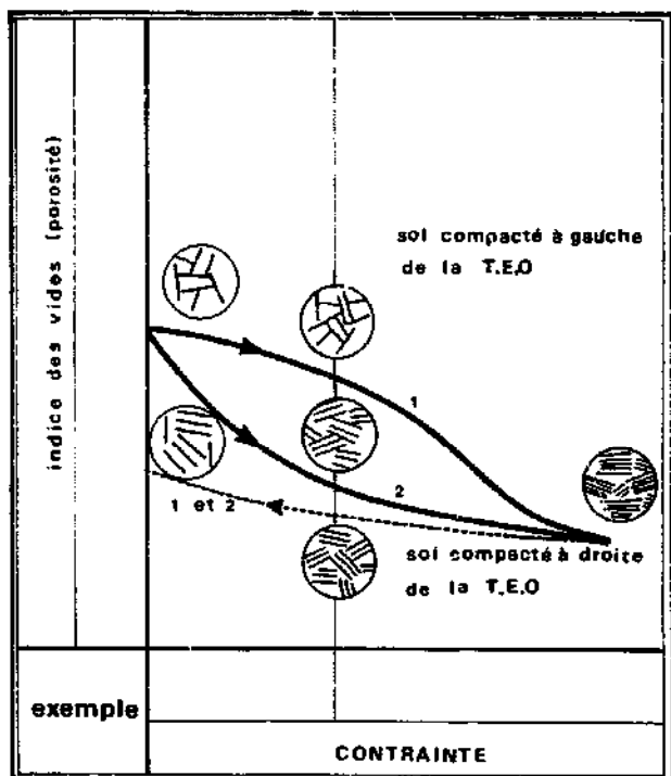
FIGURE 277 : COMPRESSION - DECOMPRESSION
