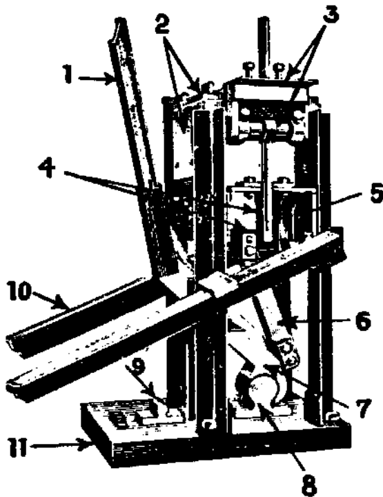
FIGURE 225 : LA PRESSE ELLSON BLOCKMASTER
