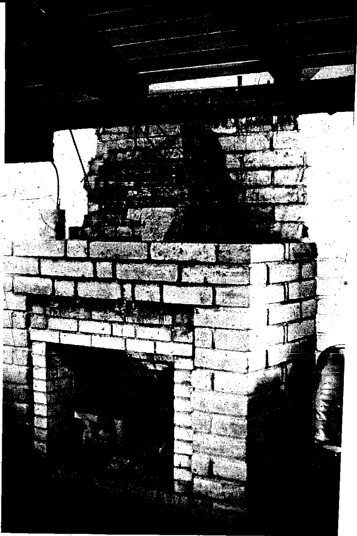
Fireplace going up, but not yet cut through the roof. The rebar's are bent into place as you go. Note firebrick around the hearth beneath the adobes. Hearth will be faced with homemade ceramic brick.
