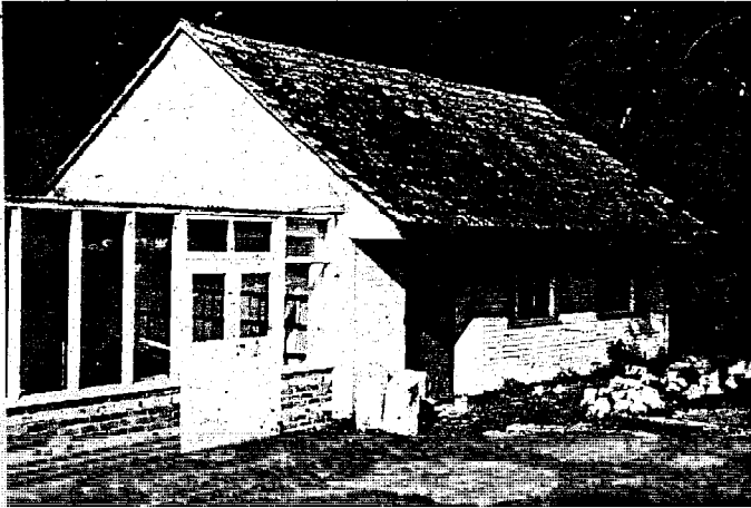
The experimental building which was constructed in 1950. The photograph was taken in October 1985.
