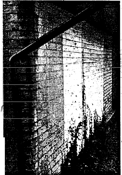
Detail view of the experimental soil-cement building, showing different surface treatments. The front corner was left untreated, but soil is in relatively good condition after 35 years of exposure.
