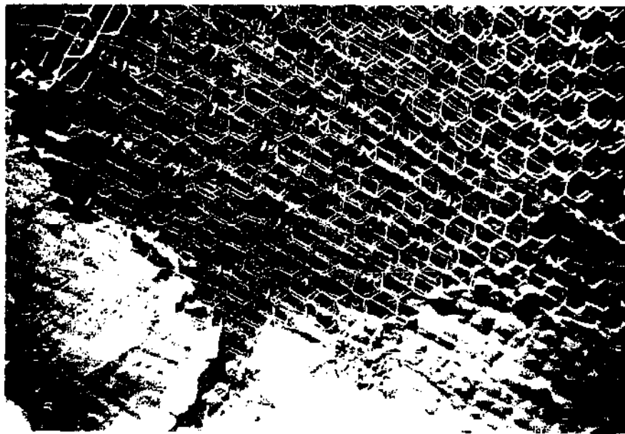
FIGURE 19 Fresh mortar applied to multiple layers of chicken-wire mesh on a 45-foot boat—showing the low-moisture mix that produces a watertight structure. (Noel D. Vietmeyer)
