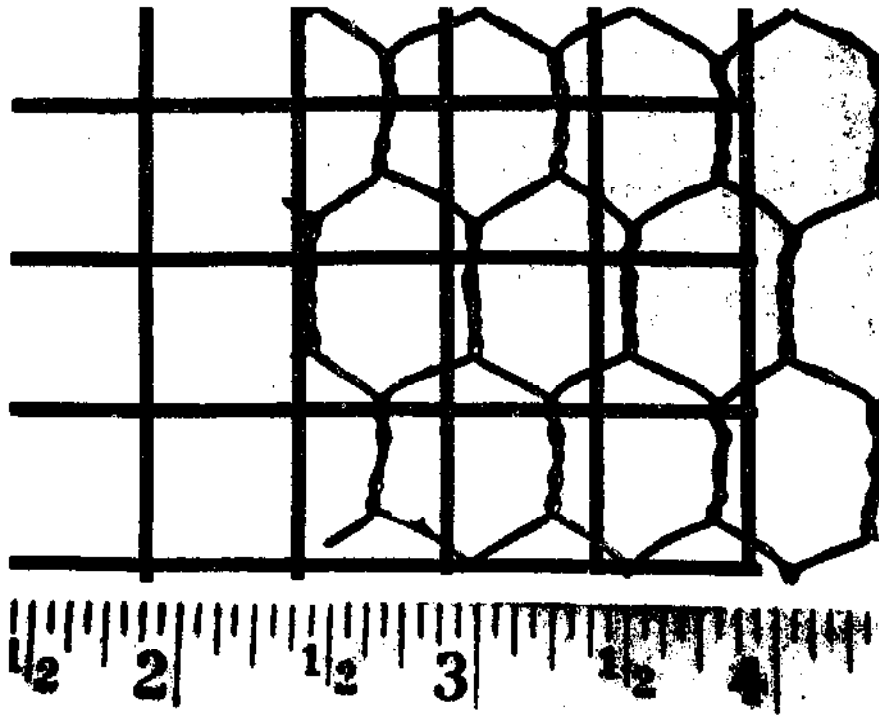
FIGURE 17 Types of reinforcing mesh commonly used for ferroceement. (R. B. Williamson, University of California, Berkeley)
