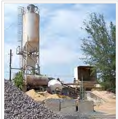
Small batching plant for local small deliveries
