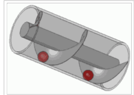
The inside of a transit mixer uses a simple Archimedes' screw to mix (clockwise) and to lift the concrete to the delivery chute (counter-clockwise).
