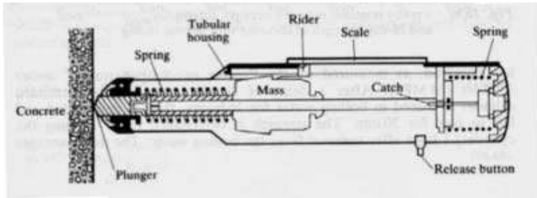
Figure 4.4: Schmidt Hammer
