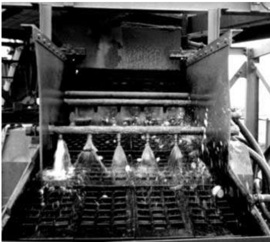
Figure 1.1: Wet screening at Gill Mill Quarry, Oxfordshire
