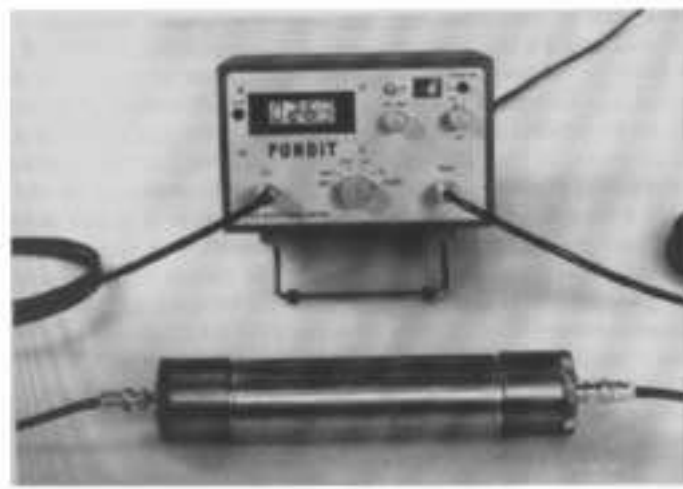
Figure 5.3: PUNDIT in laboratory
