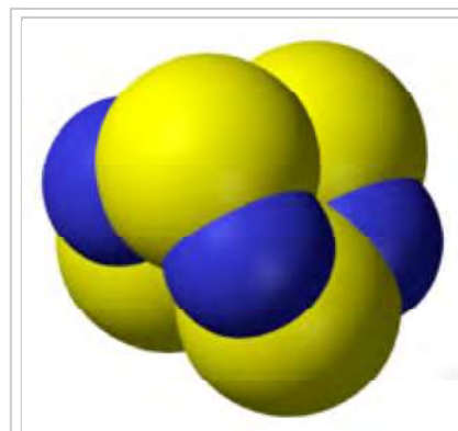
Tetrasulfur tetranitride, \text{S}_4\text{N}_4 , is a main group compound that continues to intrigue chemists
