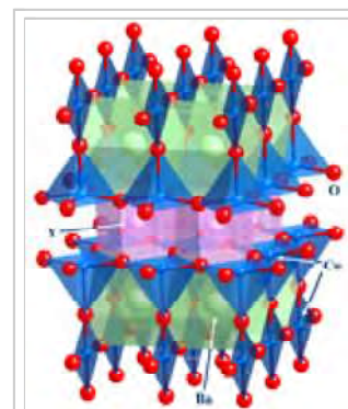
\text{YBa}_2\text{Cu}_3\text{O}_7 , or YBCO, is a high temperature superconductor able to levitate above a magnet when colder than its critical temperature of about 90 K (−183 °C)
