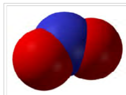
Nitrogen dioxide, \text{NO}_2 , exhibits C_{2v} symmetry
