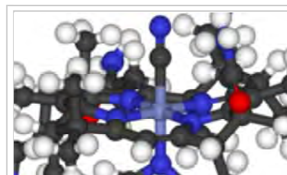
The octahedral cobalt centre of Vitamin B 12
