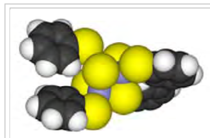
Iron-sulfur clusters are central components of iron-sulfur proteins, essential for human metabolism
