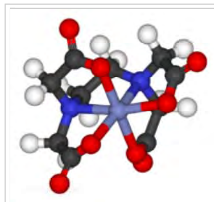
EDTA chelates an octahedrally coordinated \text{Co}^{3+} ion in [\text{Co}(\text{EDTA})]^-
