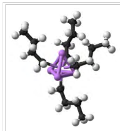
Organolithium reagents are most often found in polymeric form, such as n -butyllithium shown here
