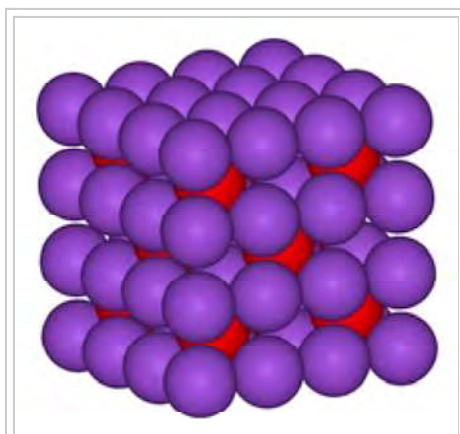
The structure of the ionic framework in potassium oxide, K_2O
