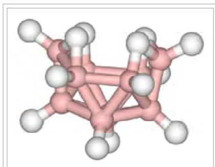
Decaborane is a powerfully toxic cluster compound of boron
