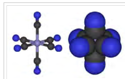
Crystal field theory explains why [\text{Fe}^{\text{III}}(\text{CN})_6]^{3-} has only one unpaired electron
