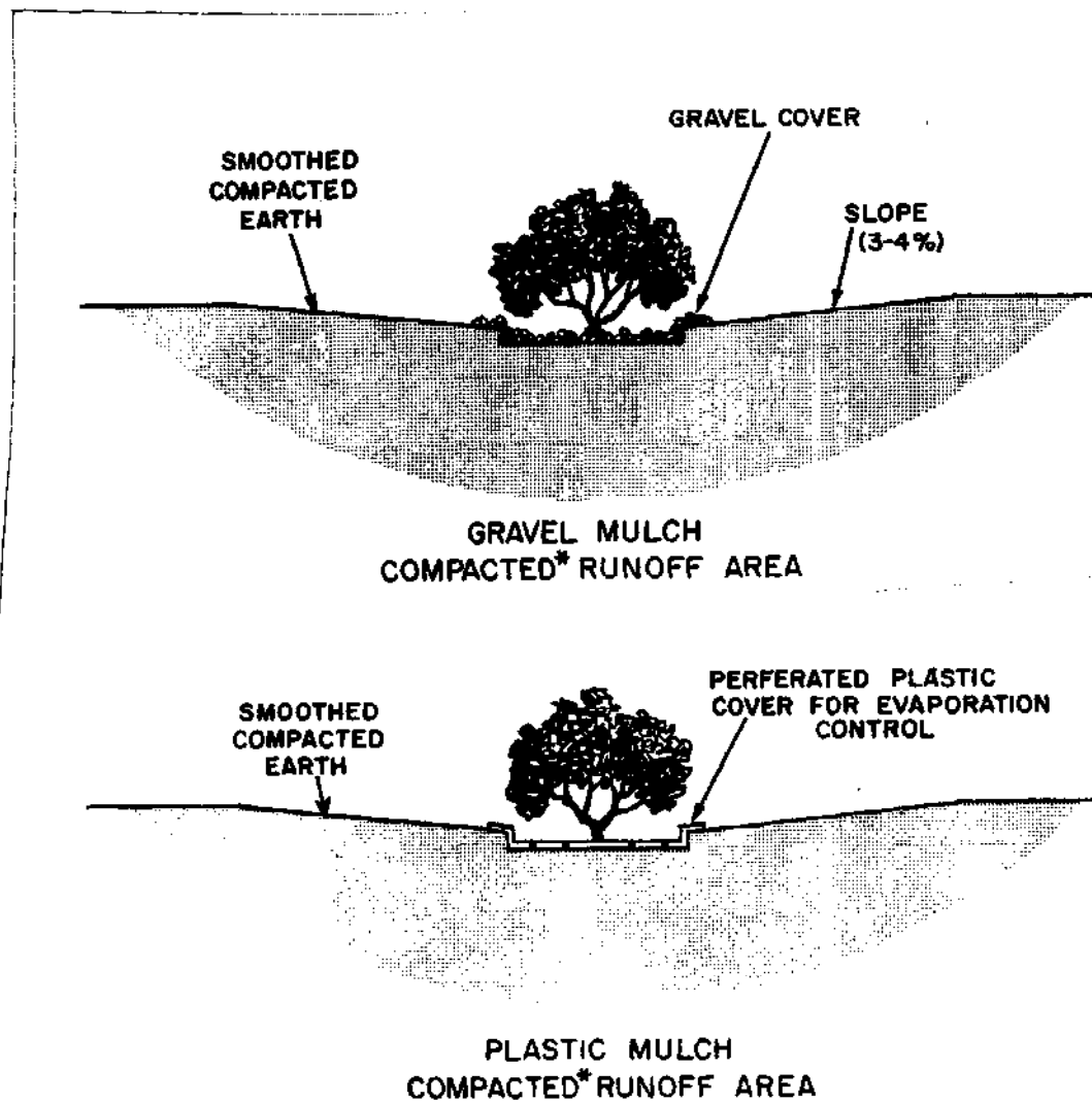
FIGURE 2 - PROPOSED RUNOFF FARMING TECHNIQUES
