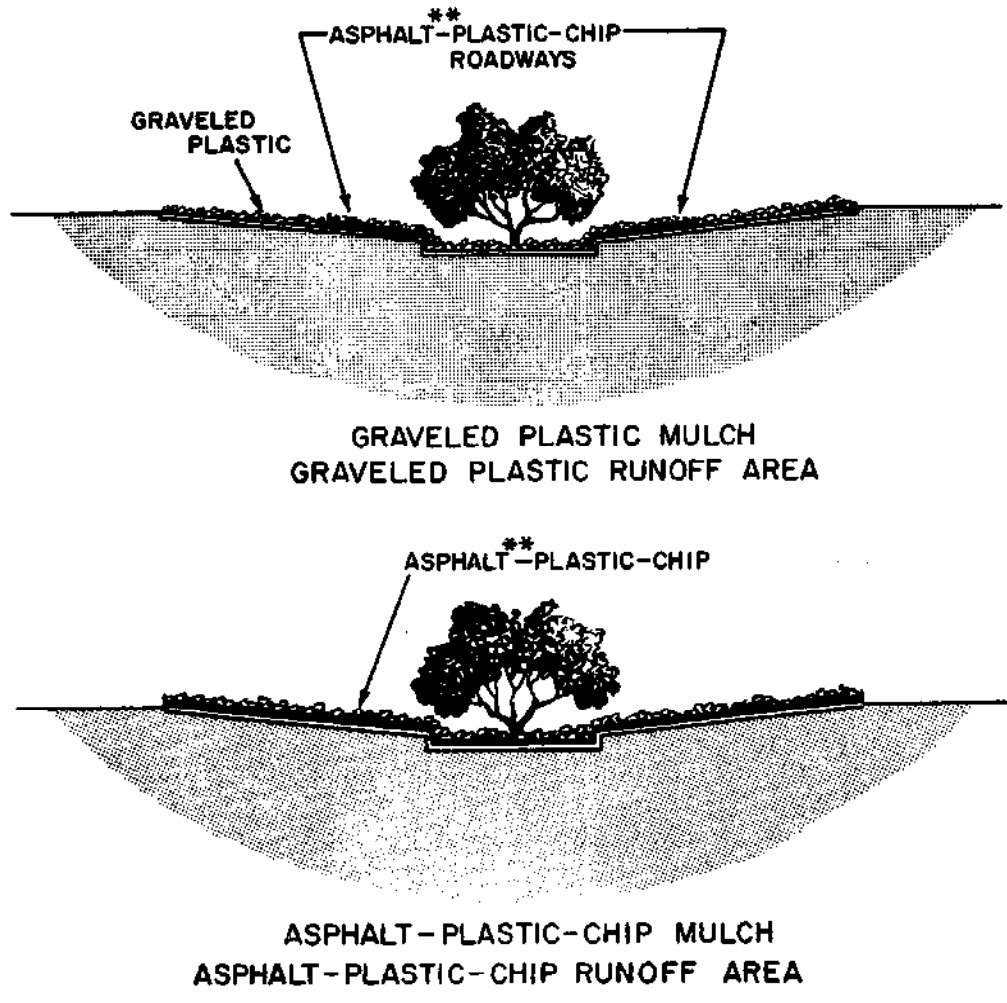
FIGURE 3 - PROPOSED RUNOFF FARMING TECHNIQUES
