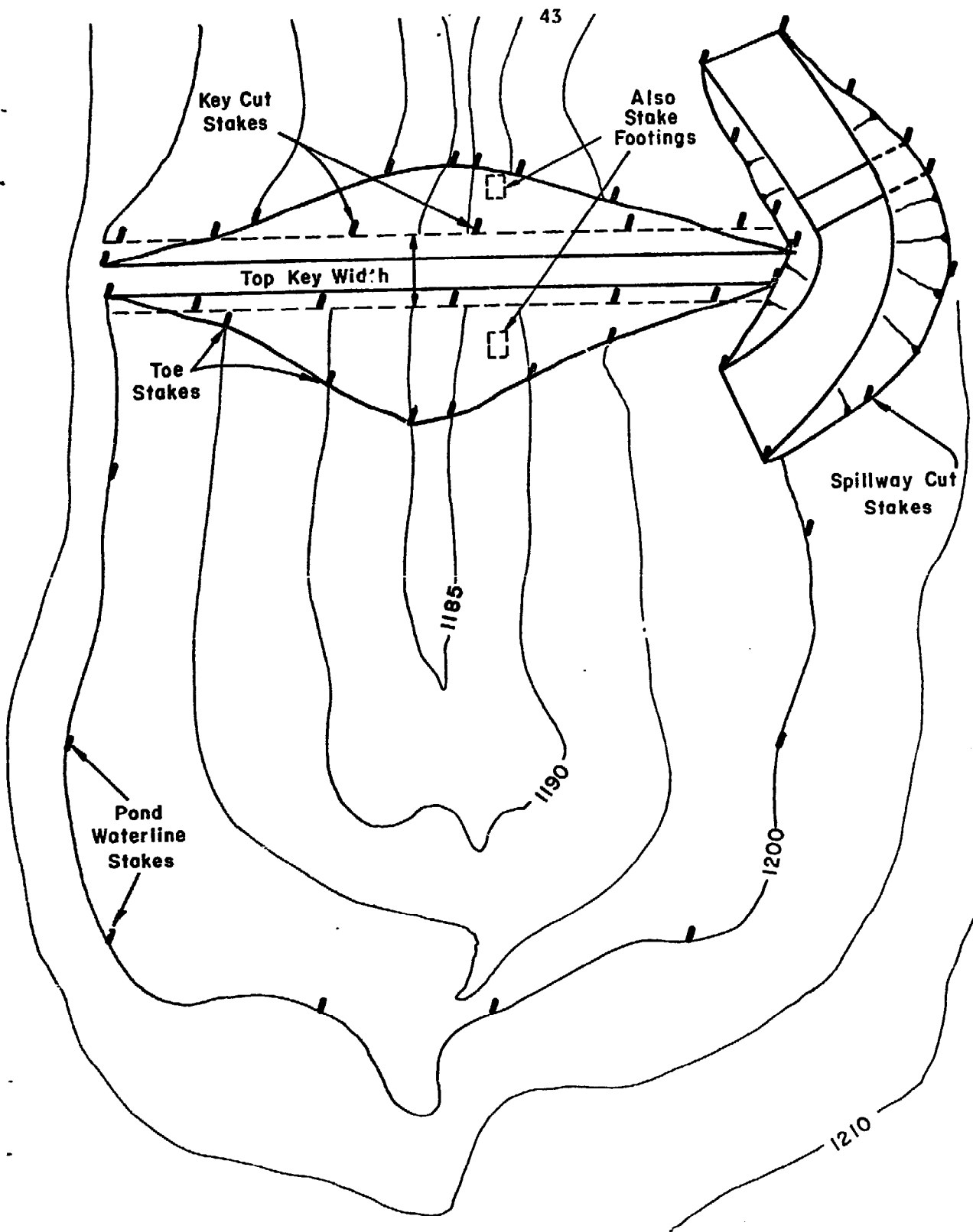
FIGURE 27 - STAKING LAYOUT
