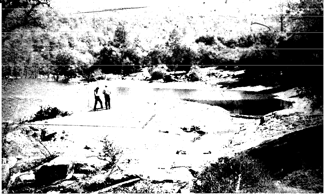
Here earth-filled sacks are used in the spillway to store additional water from late spring runoffs. Such barriers are inexpensive and easy to remove.
