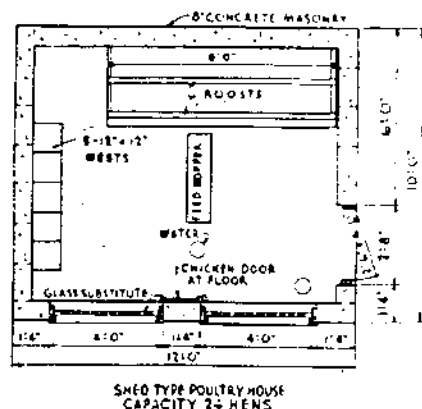
Diagram of interior of a laying house. Feed and water are placed prominently in the middle of pen to get hens to eat often — "the handier the mash . . . the more eggs."
