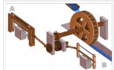
Roman Hierapolis sawmill from the 3rd century AD, the earliest known machine to combine a crank with a connecting rod. [8]
