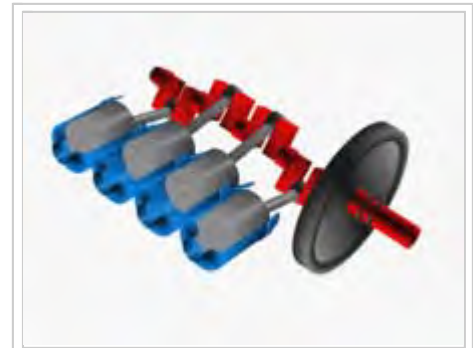
Animation showing piston and crankshaft motion in an internal combustion engine such as an automobile engine
