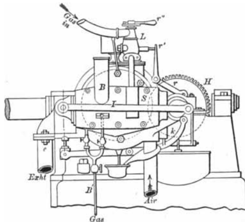
Fig. 36.—Otto Engine—End View. 1876.
