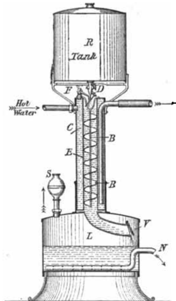
Fig. 145.—Simplex Carburator.
