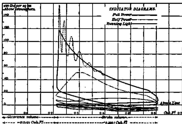
Fig. 135.—Priestman Oil Engine—Indicator Diagram.
