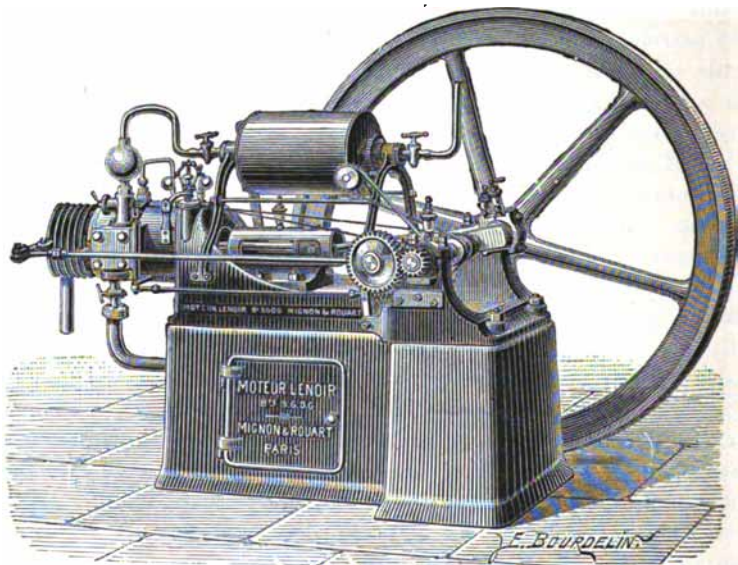
Fig. 143.—Lenoir Petroleum Engine.
