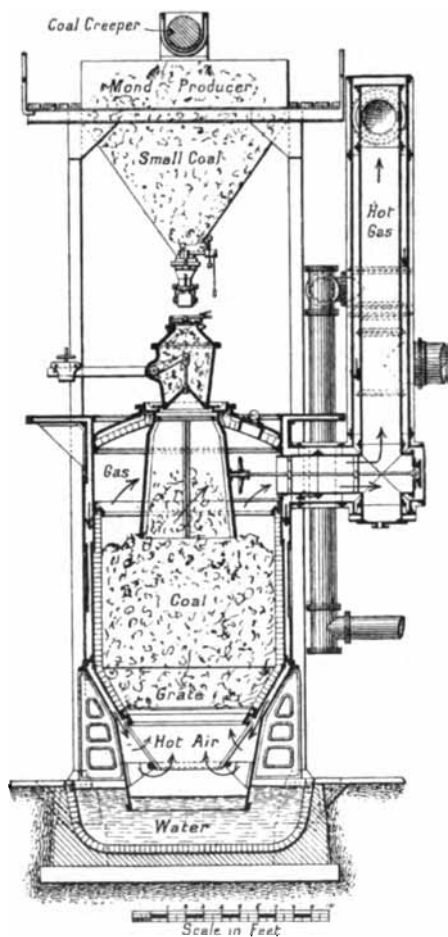
Fig. 100.—Mond Gas Producer.
