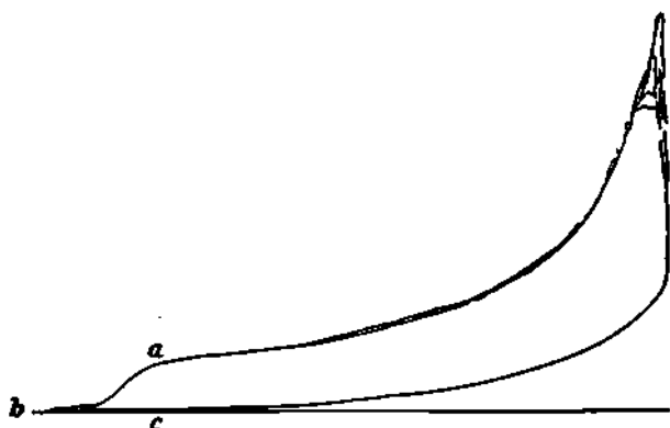
Fig. 89.—Oechelhaueser Engine—Indicator Diagram.
