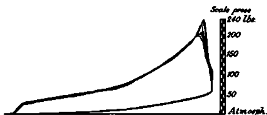
Fig. 22.—Clerk 12 H.P. Indicator Diagram.
