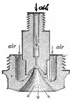
Fig. 133.—Priestman Oil Engine—Spray Maker.
