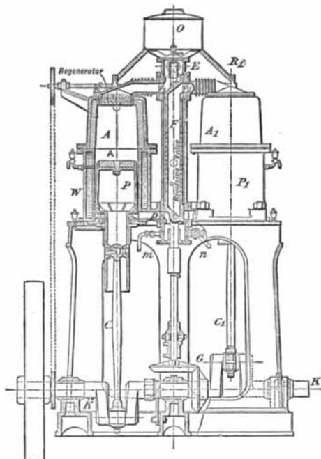
Fig. 130.—Siemens' Regenerative Engine. 1881.
