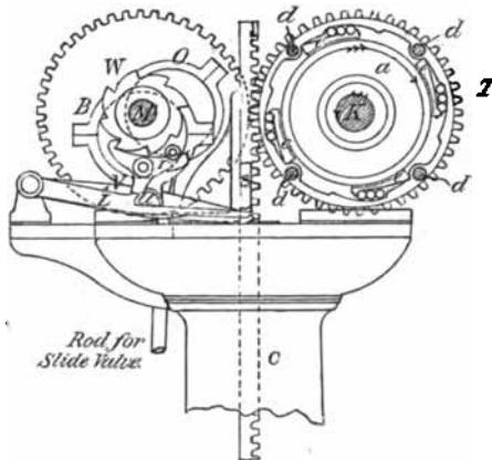
Fig. 12.—Otto and Langen Engine. 1866.
