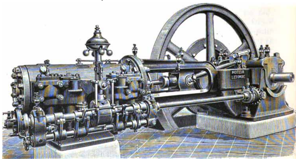
Fig. 80.—Letombe Gas Engine—Double-acting.
