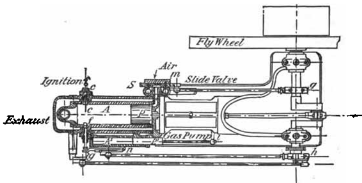
Fig. 93.—Benz Gas Engine—Plan.
