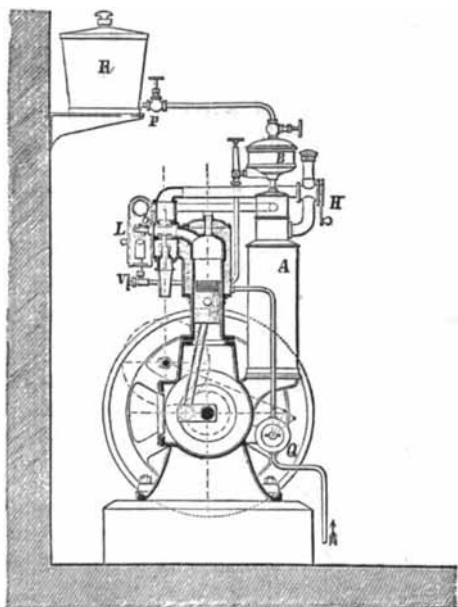
Fig. 147.—Daimler Oil Engine. 1890.
