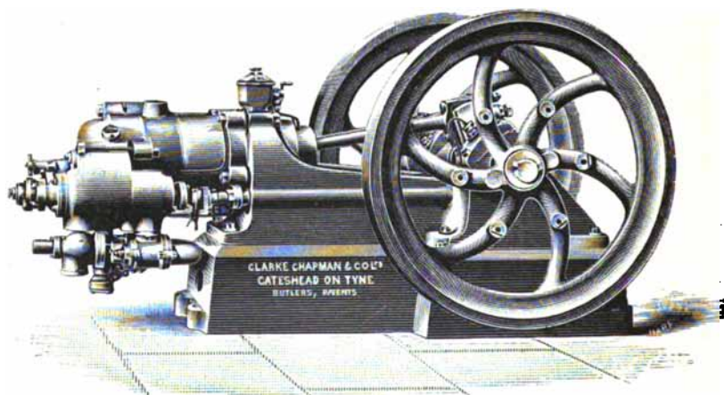
Fig. 65.—Clarke-Chapman Gas Engine—Single Cylinder. 1894-1899.
