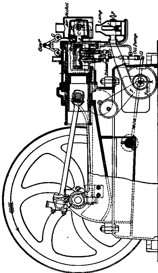
Fig. 136. ---Hornsby-Alroyd Engine—Sectional Elevation.
