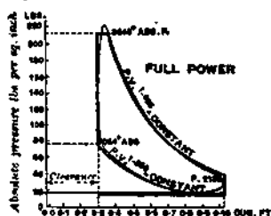
Fig. 53.—Otto—Indicator Diagram. 1888. Soc. Arts.
