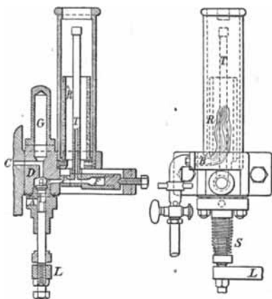
Fig. 46.—Otto Engine—Ignition Tube. 1838.
