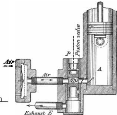
Fig. 15. — Bisschop Engine— Section of Piston Valve.
