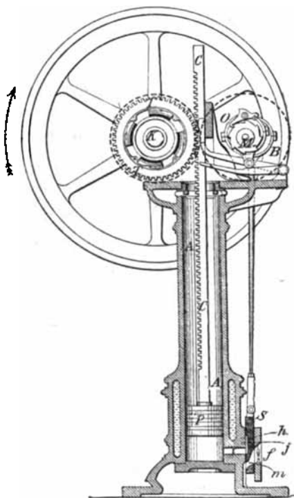
Fig. 9.—Otto and Langen Vertical Engine— Transverse Section. 1866.
