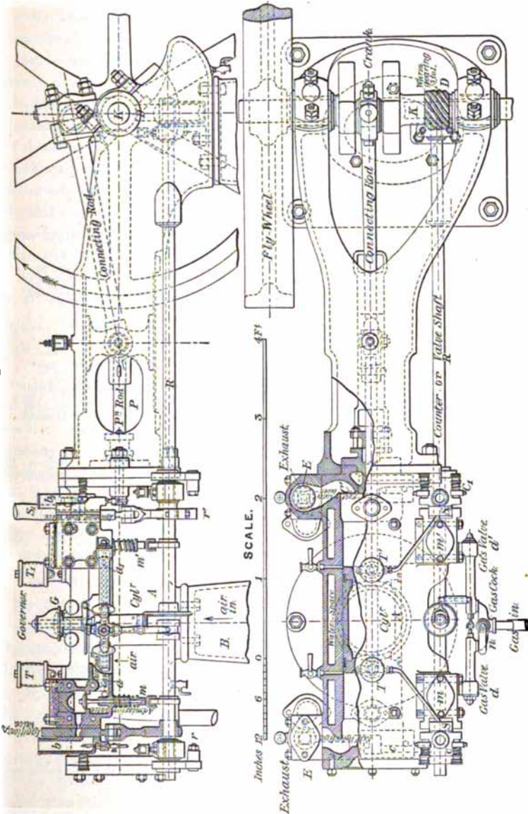
Fig. 30.—Griffin Six-Cycle Engine—Side Elevation.
