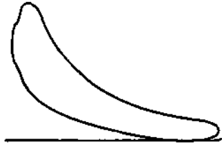
Fig. 144.—Lenoir Petroleum Engine— Indicator Diagram.
