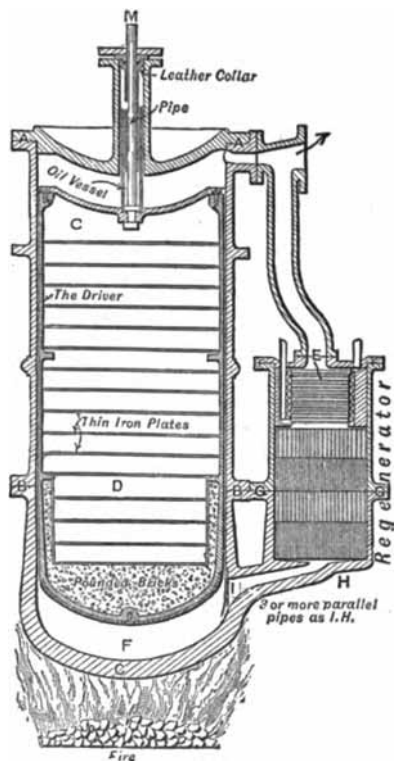
Fig. 160.—Second Stirling Engine. 1840.
