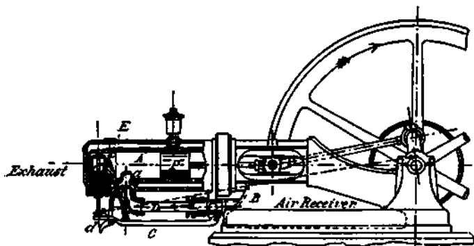
Fig. 92.—Benz Gas Engine—Elevation.
