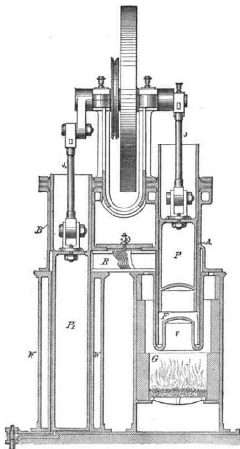
Fig. 164.—Rider Air Engine.
