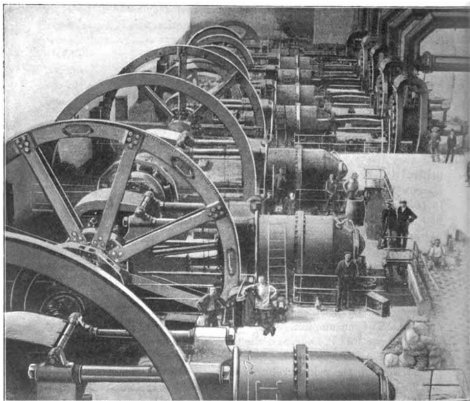
Fig. 111.—Gas Engines at Differdingen (Delamare-Deboutteville and Cockerill System).
