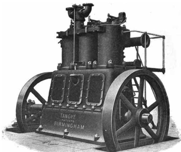
Fig. 55.—Tangye Three-cylinder Vertical Engine.
