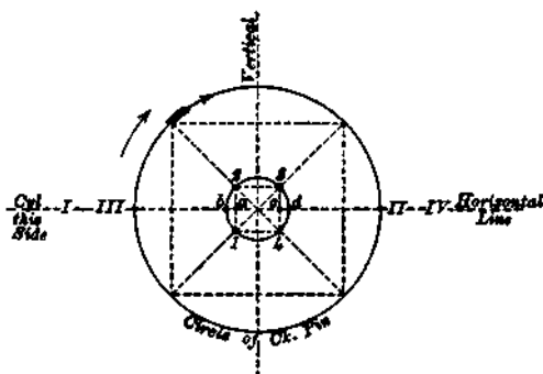
Fig. 42.—Otto Engine—Positions of Crank, Counter Shaft, and Slide Valve.
