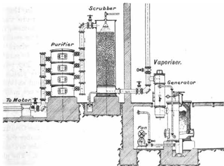
Fig. 108.—Nuremberg Suction Gas Producer.
