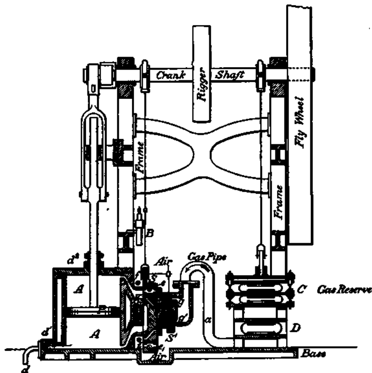
Fig. 6.—Hugon Gas Engine—Vertical. 1862.
