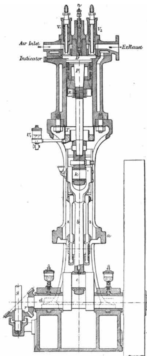
Fig. 156.—20 Horse-power Diesel Oil Motor.
