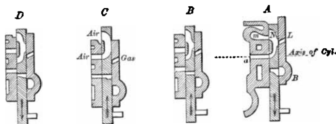
Fig. 43.—Otto Engine—Positions of Ports and Passages. 1876.
