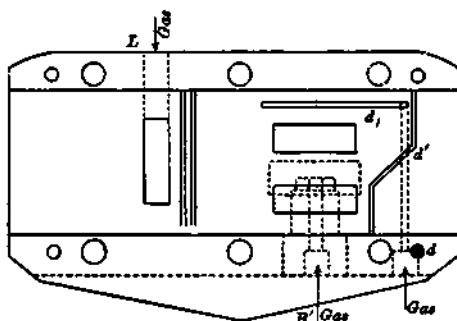
Fig. 39.—Otto Engine—Vertical View of Slide Cover. 1876.
