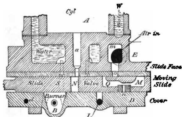
Fig. 37.—Otto Engine, 1876—Sectional Plan of Slide Valve.
