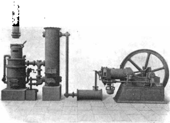
Fig. 107.—Deutz Suction Gas Producer.
