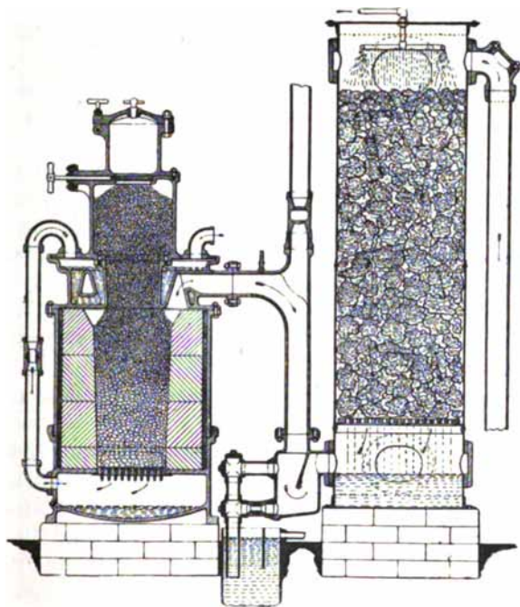
Fig. 98.—Tangye Suction Gas Producer.
