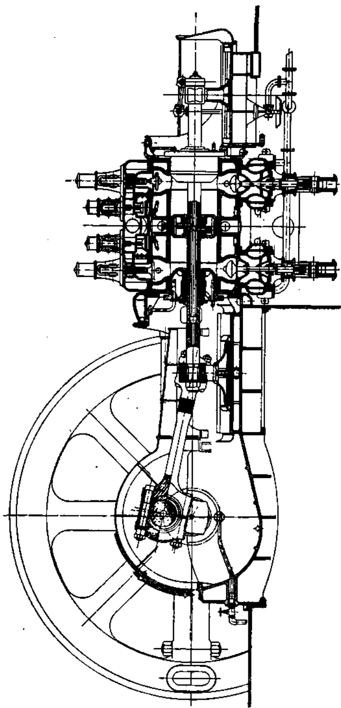
Fig. 86.—Nuremberg Double-acting Engine—Longitudinal Section.
