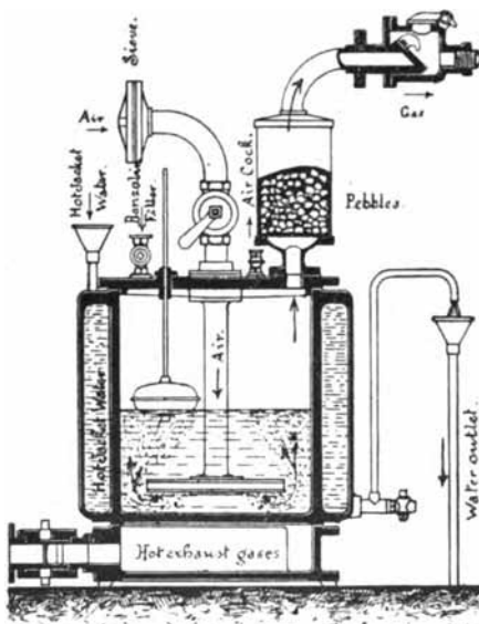
Fig. 150.—Benzine Carburetor—Otto Engine.
