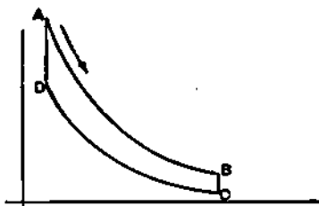
Fig. 115.—Stirling Cycle—Constant Volume.
