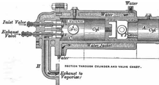
Fig. 132.—Priestman Oil Engine.
