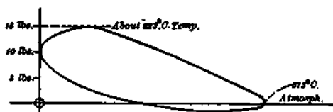
Fig. 163.—Bailey Air Engine—Indicator Diagram.
