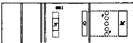
Fig. 38.—Otto Engine—Vertical View of Slide Valve.
