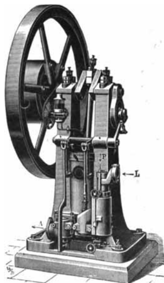
Fig. 149.—Koerting Oil Engine.
