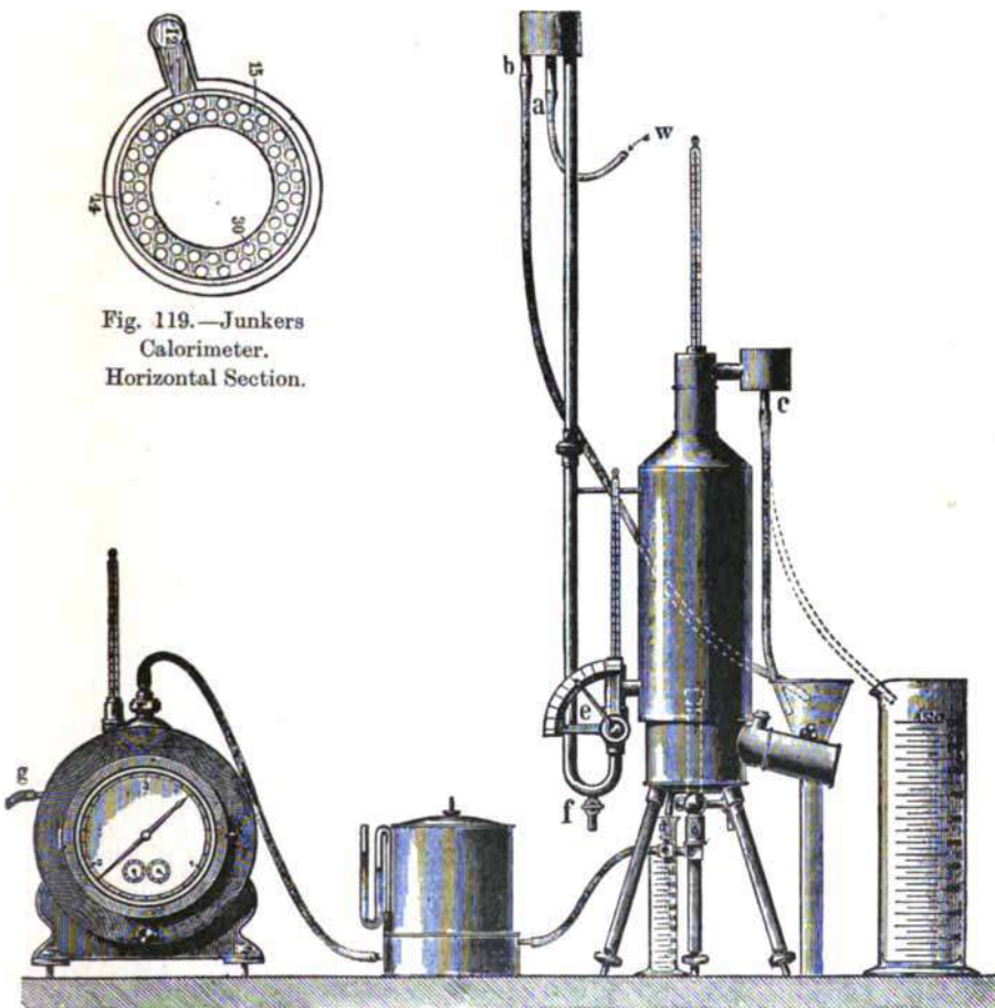
Fig. 120.—Junkers Gas Calorimeter, with Gas Meter, &c.
