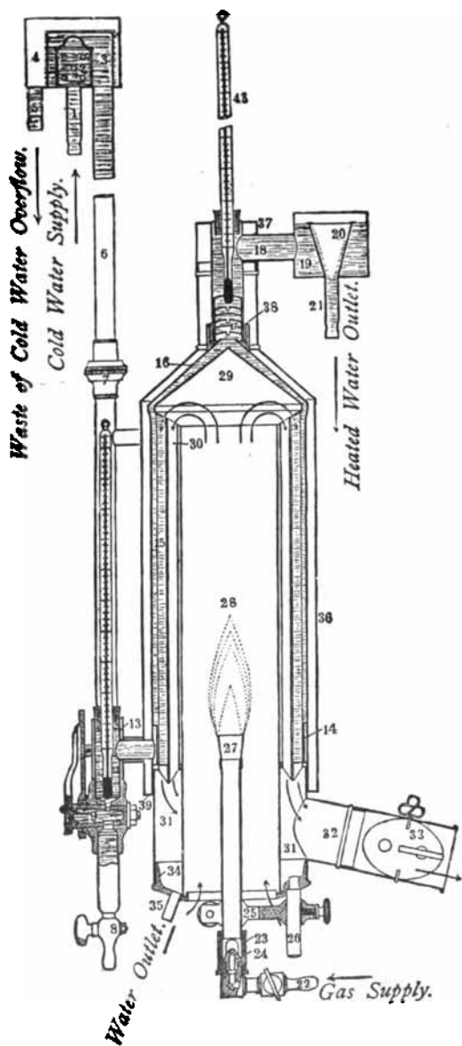
Fig. 118.—Junkers Gas Calorimeter. Sectional Elevation. 1899.
