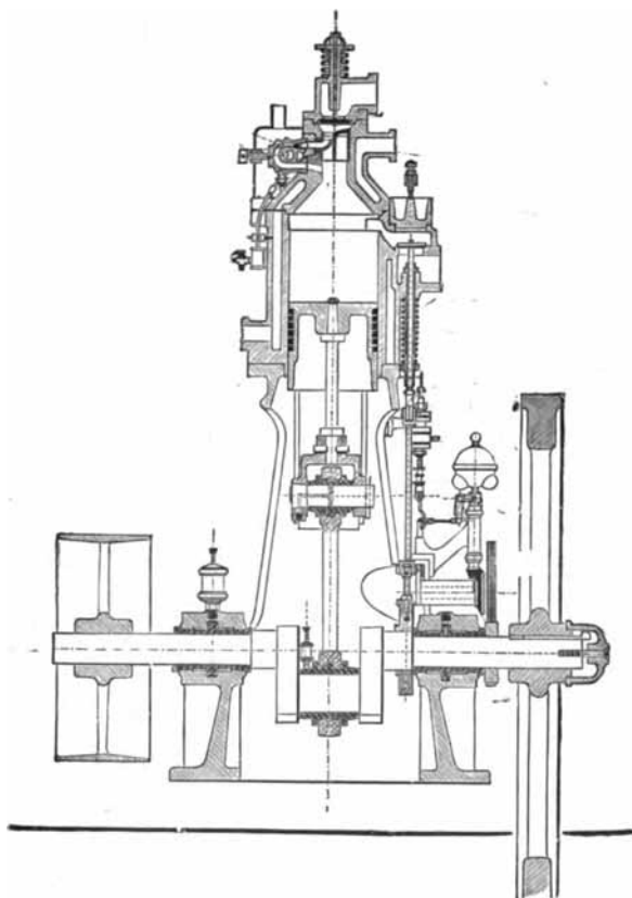
Fig. 162.—Capitaine Oil Engine.
