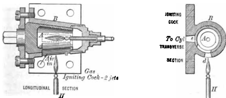
Fig. 1.—Barnett's Engine Gas Ignition Cock—Longitudinal and Transverse Sections. 1838.
