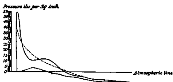
Fig. 13.—Otto and Langen Engine—Indicator Diagram (Clerk). 1866.
