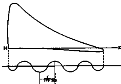
Fig. 123.—Witz Time Diagram.
