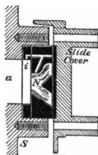
Fig. 41.—Ignition Flame and Slide Cover.
