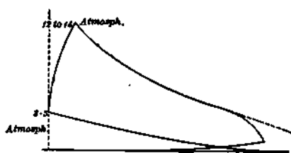
Fig. 79.—Niel Engine—Indicator Diagram. 1891.
