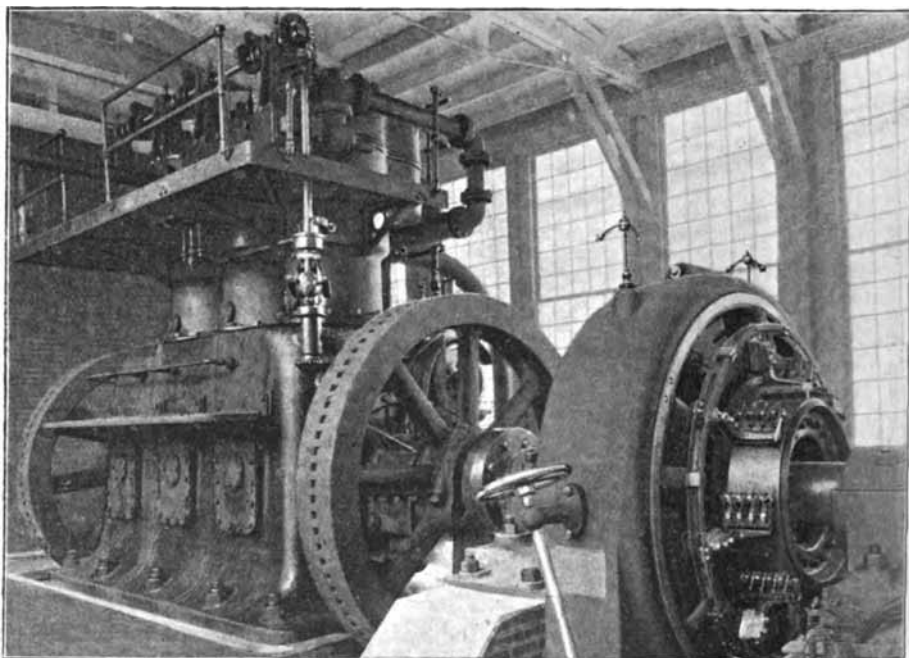
Fig. 60.—Westinghouse Vertical 650 B.H.P. Three-Cylinder Gas Engine, with Direct-Driven Dynamo.
