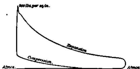
Fig. 151.—Otto-Petroleum Engine. Indicator Diagram.
