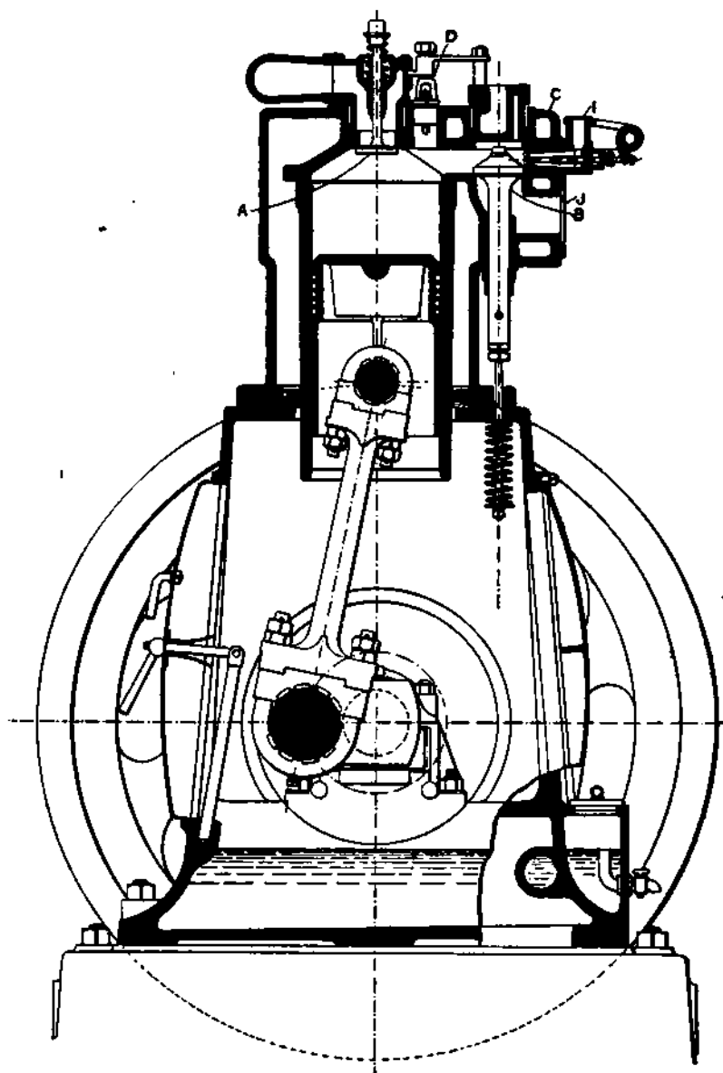
Fig 57.—150-H.P. Four-cylinder Fielding & Platt Engine—Sectional Elevation.
