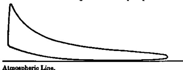
Fig. 106.—Indicator Diagram of 29 H.P. Engine worked with Pierson Suction Producer.
