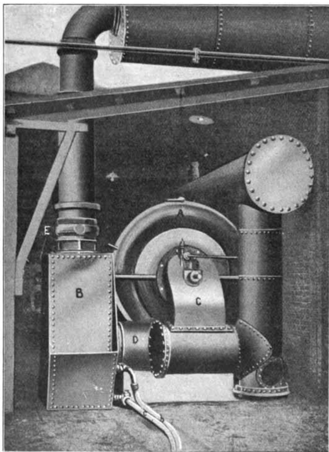
Fig. 110.—Centrifugal Fan for Cleaning Blast-furnace Gases.
