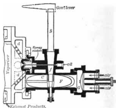
Fig. 134.—Priestman Oil Engine—Vaporiser.
