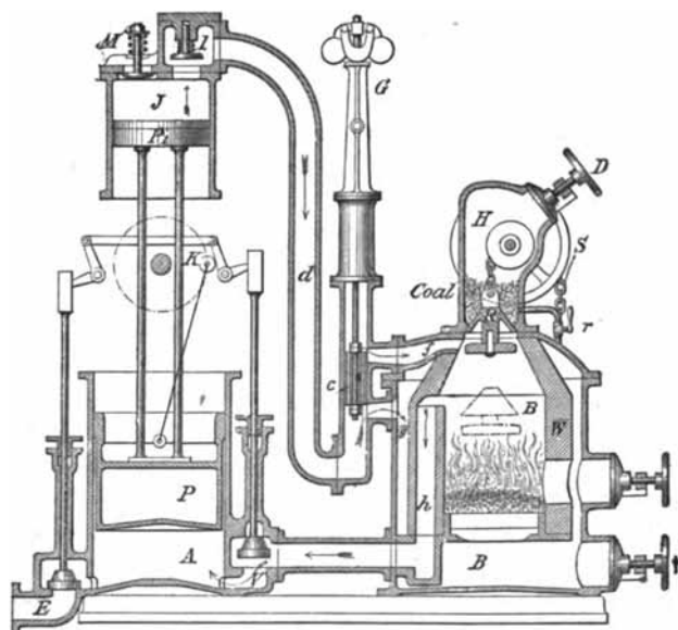
Fig. 157.—Buckett Air Engine—Single Cylinder.
