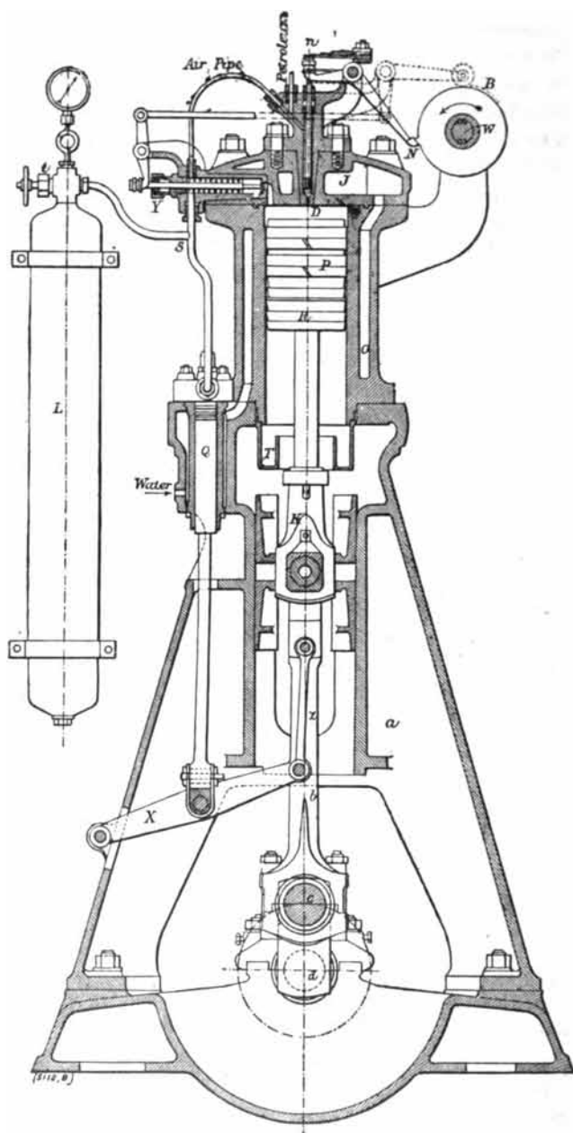
Fig. 155.—20 Horse-power Diesel Oil Motor.
