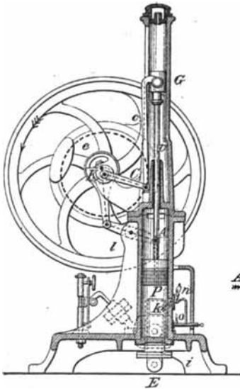
Fig. 14. — Bisschop Engine— Sectional Elevation. 1870.
