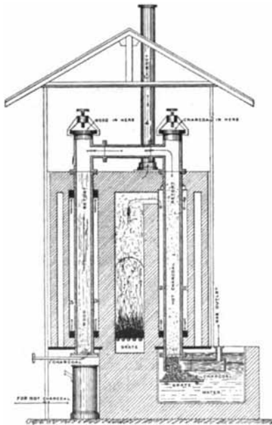
Fig. 109.—Wood Gas Producer—Section (Riché). 1899.
