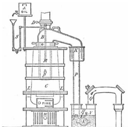
Fig. 126.—Mansfield Oil Gas Producer.
