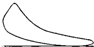
Fig. 74.—Second Lenoir Engine—Indicator Diagram.
