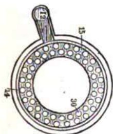
Fig. 119.—Junkers Calorimeter. Horizontal Section.
