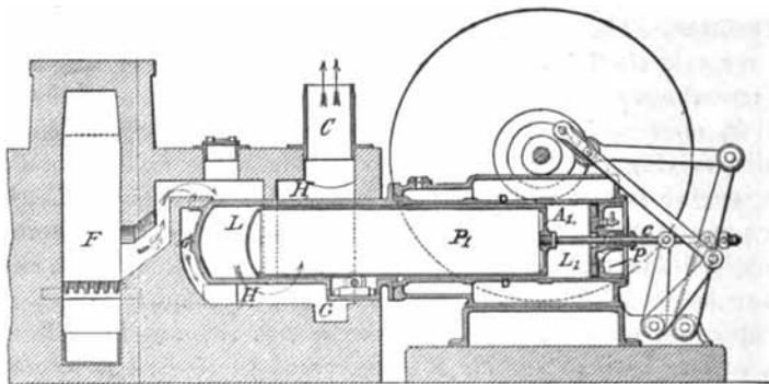
Fig. 162.—Bailey Air Engine.
