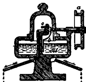
Sectional elevation.
