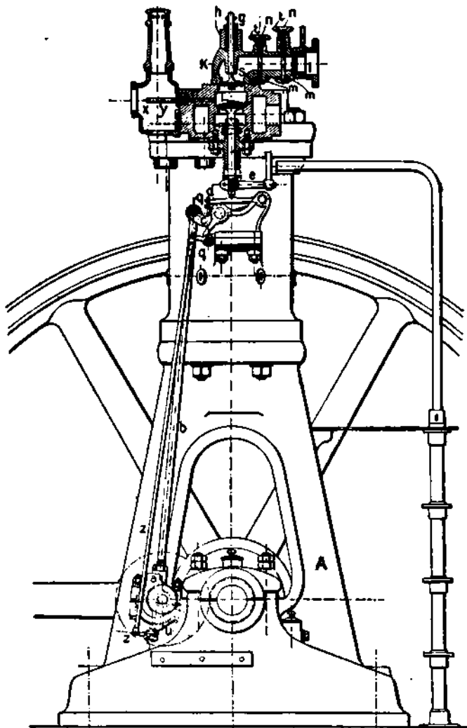
Fig. 153.—Bánki Oil Engine—Sectional Elevation.
