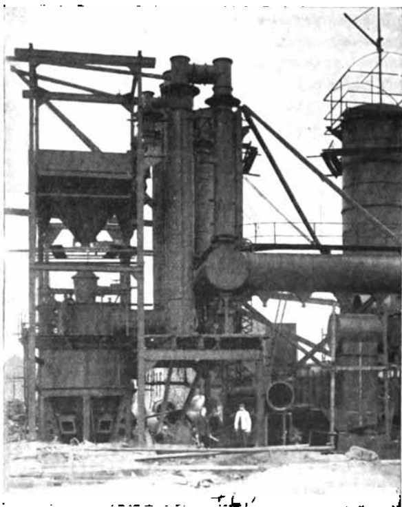
Fig. 101.—Mond Gas Plant at Warrington.
