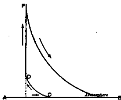
Fig. 121.—Diagram of Perfect Cycle with Compression.
