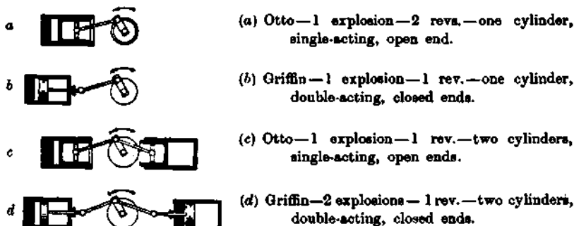
Fig. 33.—Diagram of Single- and Double-Cylinder Explosion Engines.
