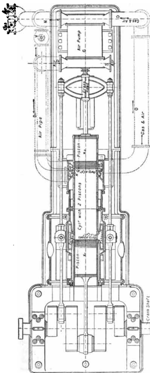
Fig. 88.—600 Horse-power Oechelhauser Two-cycle Engine.
