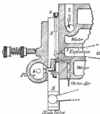
Fig. 21.—Clerk Engine—Ignition Valve. 1880.
