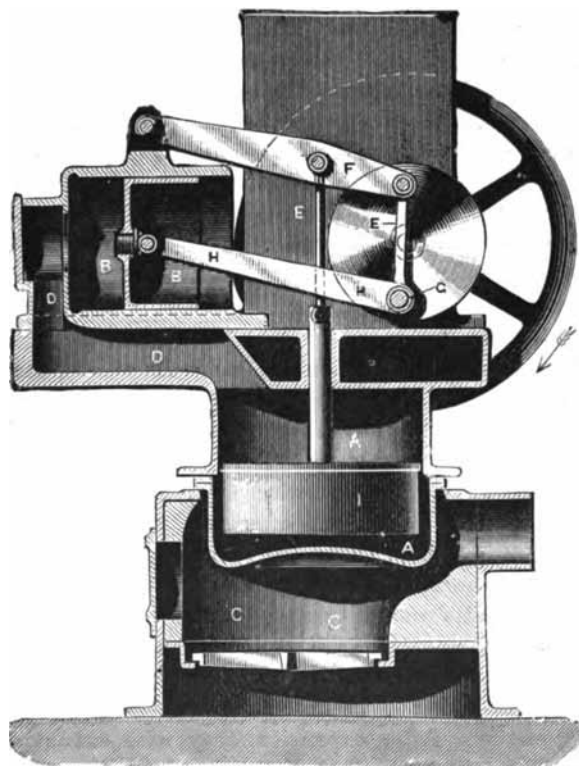
Fig. 161.—Robinson Air Engine.
