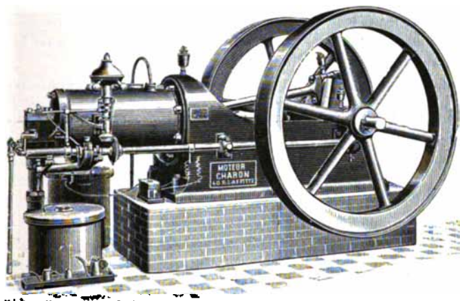
Fig. 75.—Charon Gas Engine.
