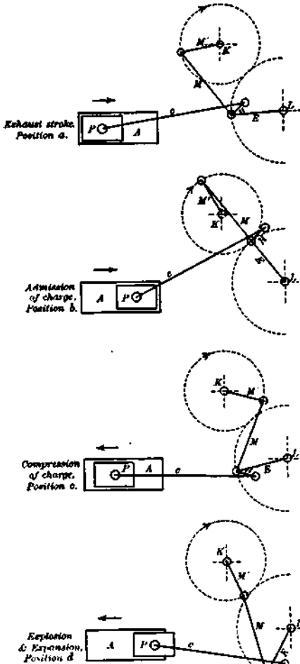
Fig. 27.—Atkinson Cycle Engine—Four positions of Link and Toggle Motion. 1836.
