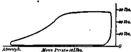
Fig. 158.—Buckett Air Engine—Indicator Diagram.
