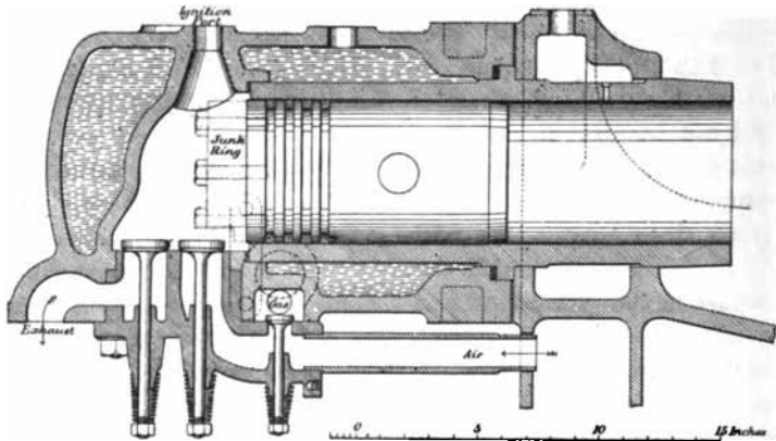
Fig. 125.—Experimental Gas Engine—Burstall's Tests. 1898, 1901.
