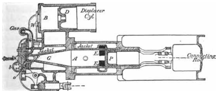
Fig. 20.—Clerk Engine—Sectional Plan. 1880.
