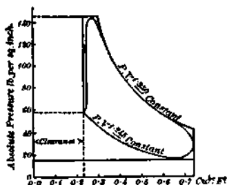
Fig. 32.—Griffin Engine—Indicator Diagram. Society Arts . 1888.
