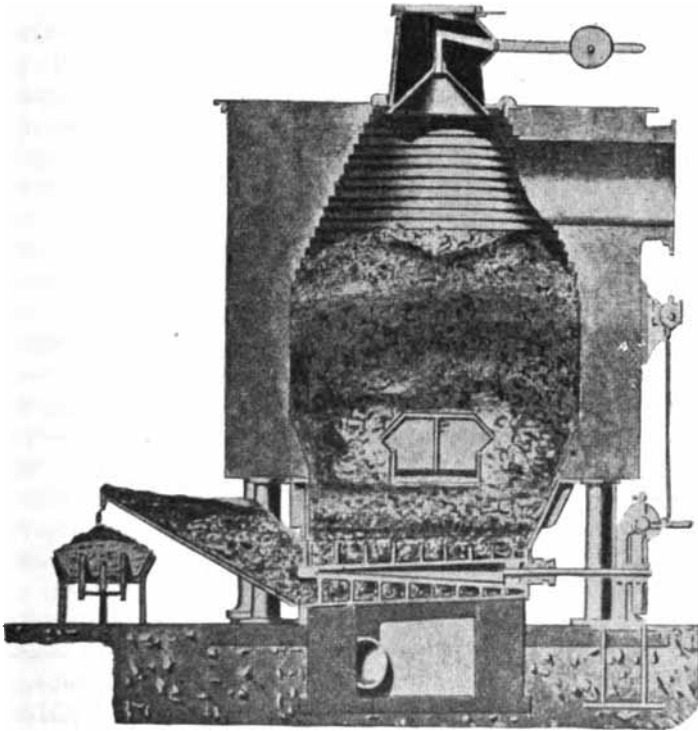
Fig. 99.—Wilson Gas Producer.
