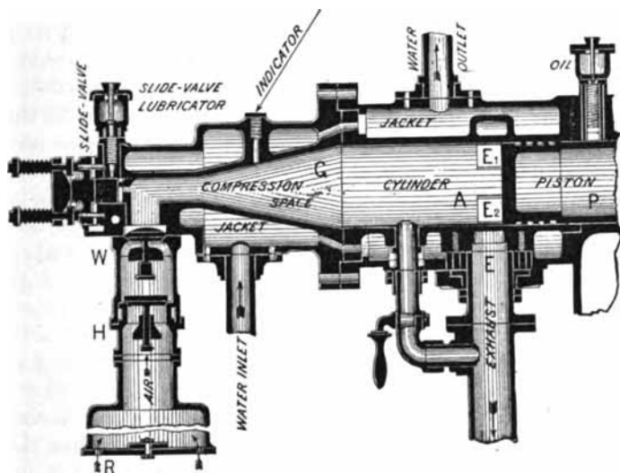
Fig. 19.—Clerk Engine—Sectional Elevation. 1880.
