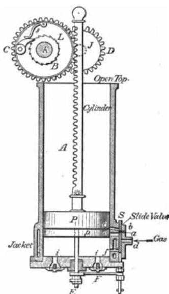
Fig. 2.—Barsanti and Matteucci's Gas Atmospheric Engine. 1854.
