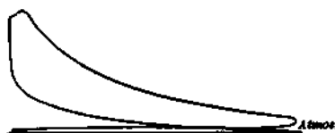
Fig. 139.—Trusty Oil Engine—Indicator Diagram.
