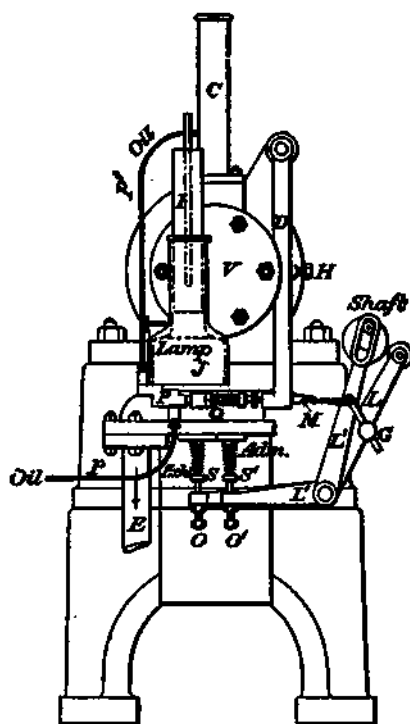
Fig. 138.—Trusty Oil Engine. 1891.
