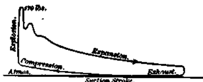
Fig. 129.—Spiel Oil Engine—Indicator Diagram.
