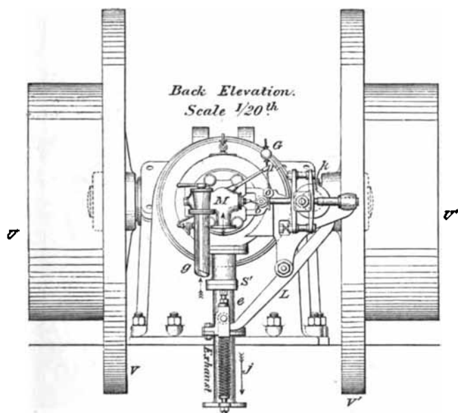
Fig. 67.—Simplex Engine.
