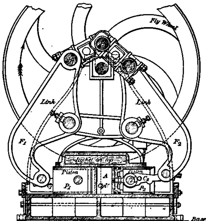
Fig. 24.—Atkinson Differential Engine. 1884.
