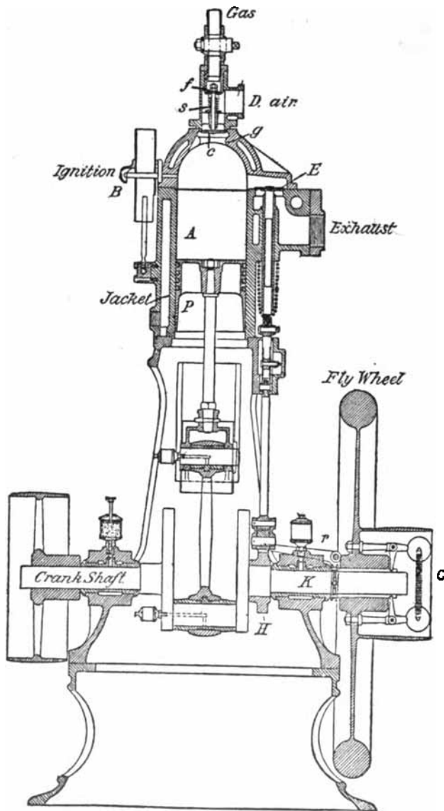
Fig. 94.—Capitaine Gas Engine—Sectional Elevation.
