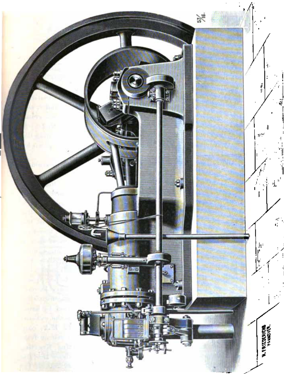
Fig. 82.—Koerting Four-cycle Horizontal Engine. 1906.
