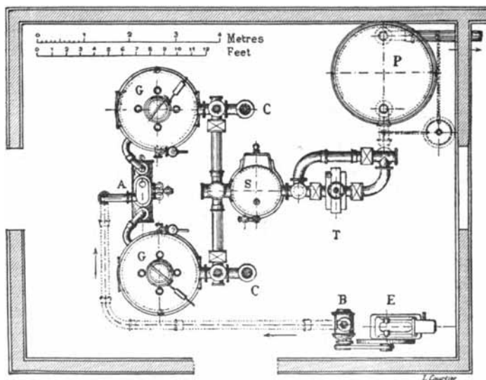
Fig. 103.—Lenoachez Gas Plant—Plan.
