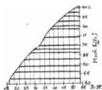
Fig. 76.—Charon Gas Engine—Varying mechanical efficiencies according to power, on same engine.
