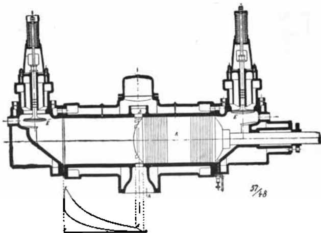
Fig. 84.—Koerting Engine—Section of Cylinder with Diagram.
