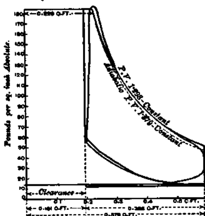
Fig. 23.—Beck Engine—Indicator Diagram. 1888.
