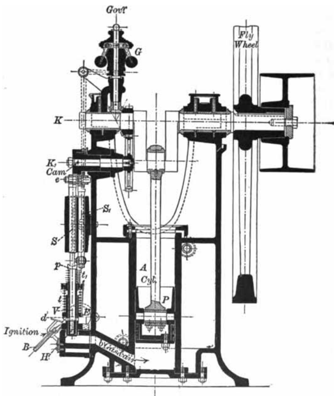
Fig. 91.—Adam Gas Engine—Sectional Elevation. 1888-1899.
