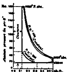
Fig. 28.—Atkinson Cycle Engine —Indicator Diagram. Society Arts . 1888.
