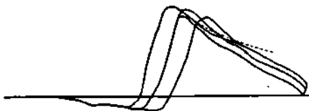
Fig. 5.—Lenoir Engine—Indicator Diagram (Slade). 1860.
