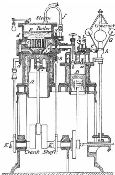
Fig. 16.—Simon Vertical Engine. 1877.
