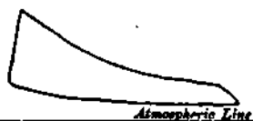
Fig. 51.—Otto—Indicator Diameter. 1881.
