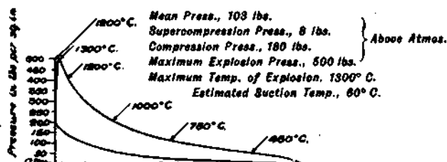
Fig. 63.—Diagram of National "Super-compression" Engine.
