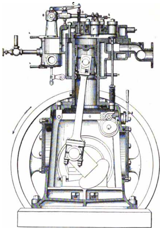
Fig. 59.—Sectional View, Westinghouse Engine.
