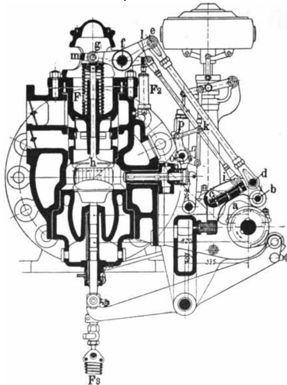
Fig. 87.—Nuremberg Engine—Valve Gear and Governor.
