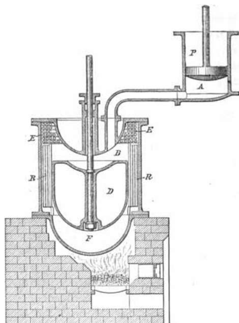
Fig. 159.—First Stirling Engine. About 1830.
