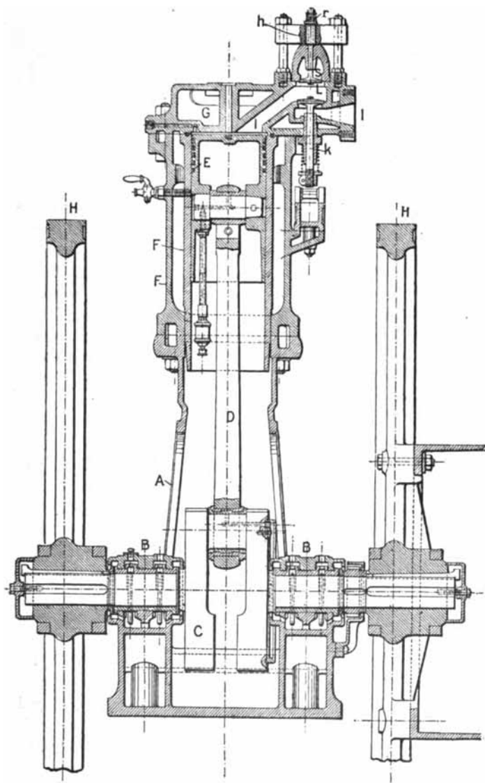
Fig. 154.—Bánki Oil Engine—Sectional Elevation.
