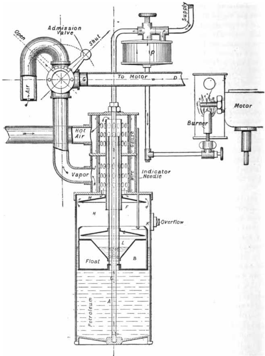
Fig. 148.—Daimler Oil Engine. Vaporiser.
