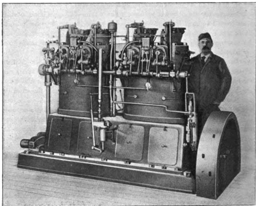
Fig. 142.—Otto Gasoline Engine for "Holland" Submarine Torpedo Vessel.
