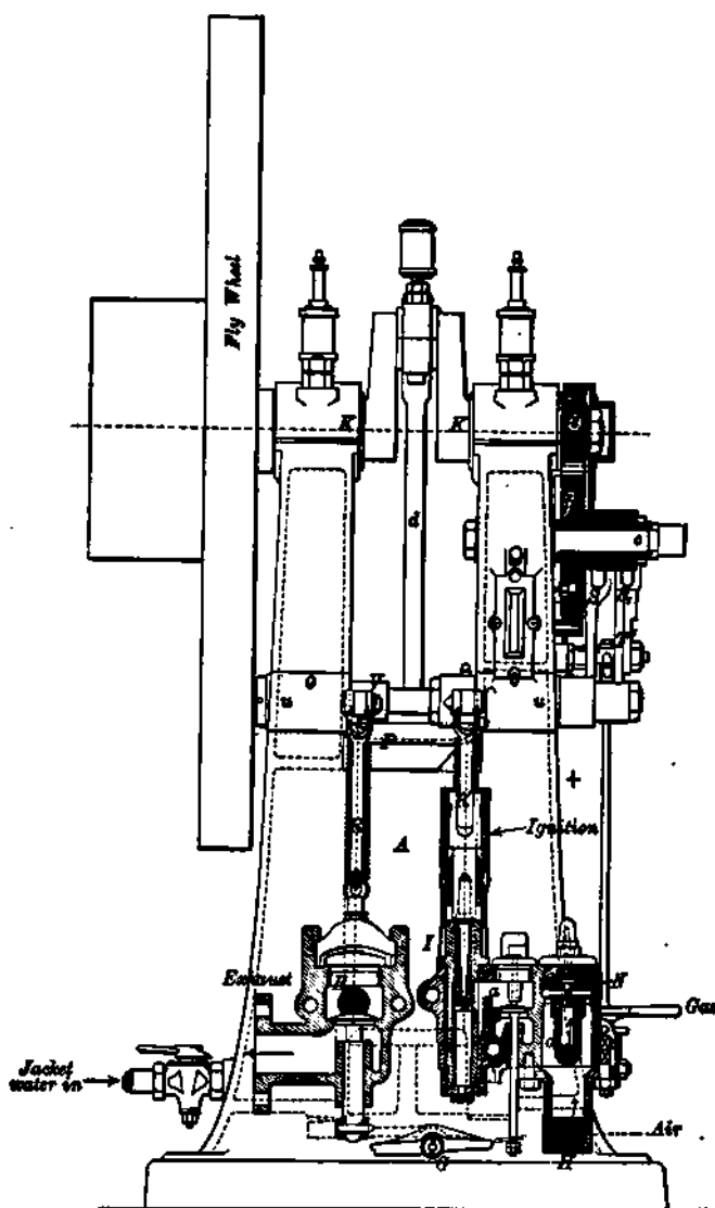
Fig. 81.—Koerting Gas Engine—Sectional Elevation. 1888-1899.
