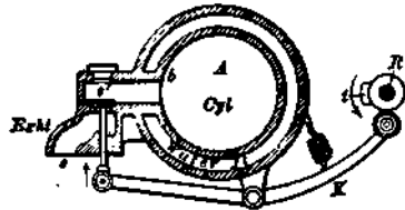
Fig. 44.—Otto Engine—Exhaust Valve. 1876.
