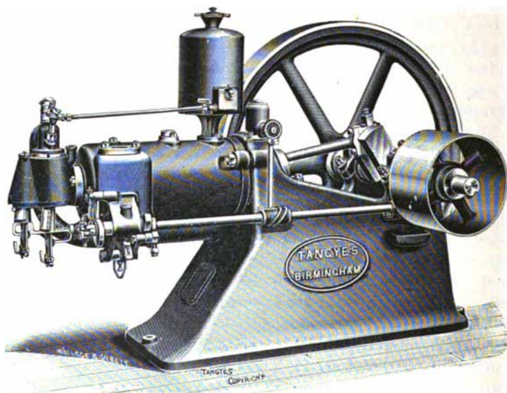
Fig. 140.—Tangye Oil Engine.
