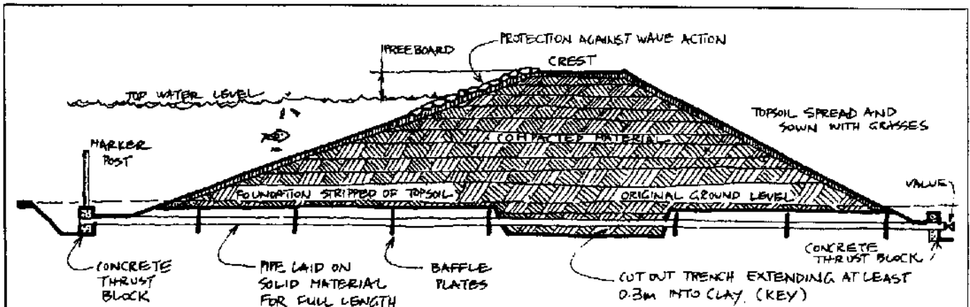
FIGURE 7.18 DAM WITH LOCK PIPES.
