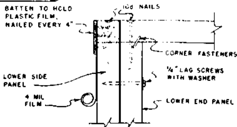
FASTENING DETAIL
