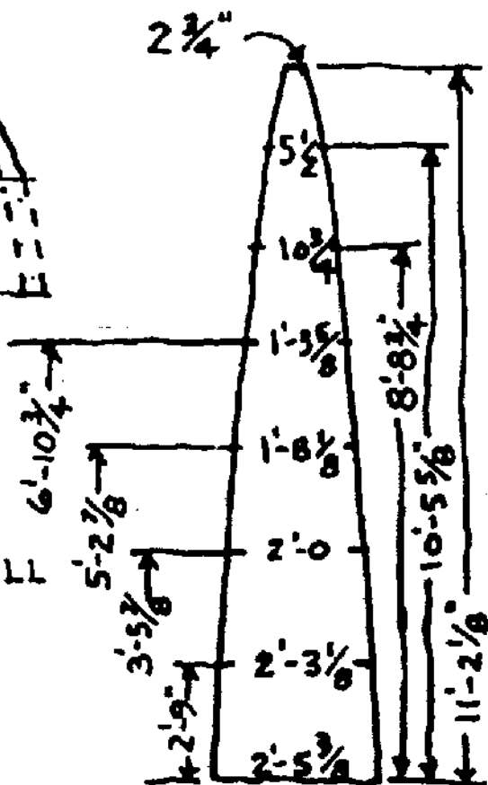
TYPICAL FIBERGLASS PANEL
