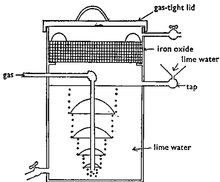
SCRUBBING UNIT
