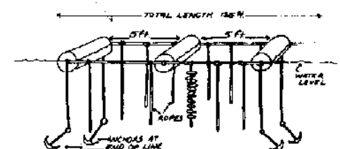
LONG LINE METHOD OF OYSTER CULTURE
