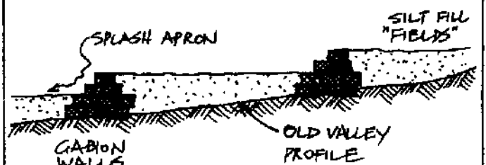
FIGURE 7.14 Eroding gullies are best stabilised using strong wire baskets to contain stones or shingle; these resist floods well.
