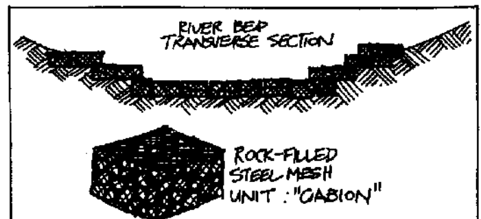
FIGURE 7.13 CHECK DAM FOR RAM PUMP OR WATER WHEEL Only 1–3 m of head enables modest energy use for mechanical power, lift pumps, or diversion to canals.
