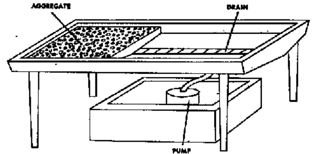
A simple mechanical subirrigation system.
