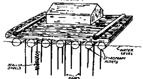
RAFT FOR OYSTER OR MUSSEL CULTURE
