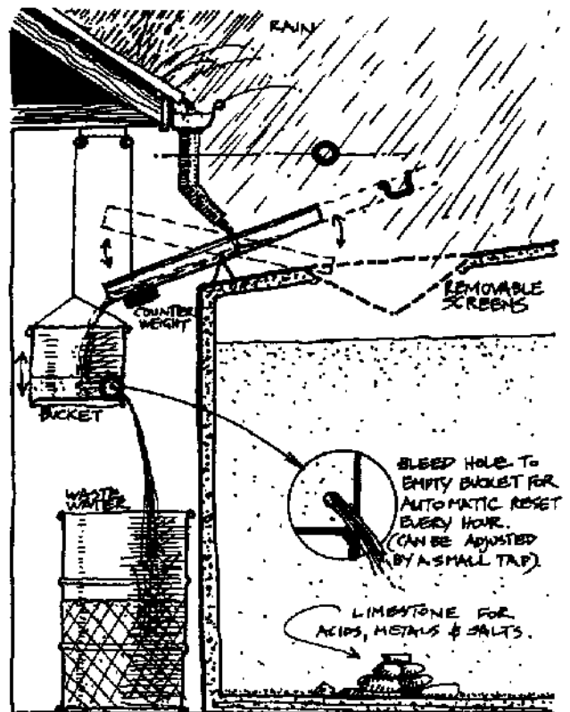
FIGURE 7.21 METHODS OF REJECTION OF FIRST WATER FLOW OFF A ROOF.
