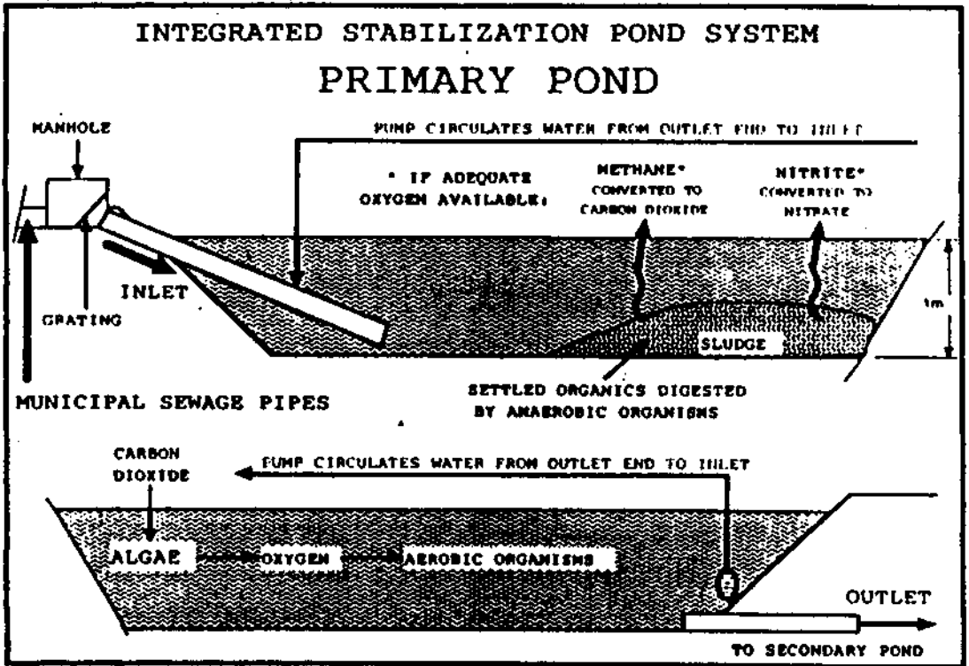
Fig.1, Primary pond
