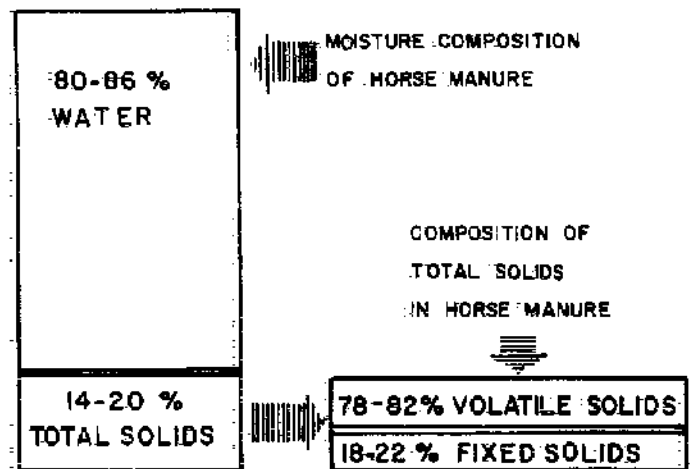
Figure 5.6 Moisture and solids content of horse manure.
