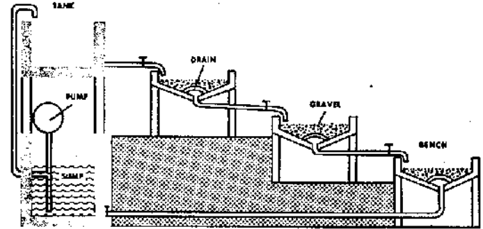
Cross-section of a mechanical gravity-feed system.
