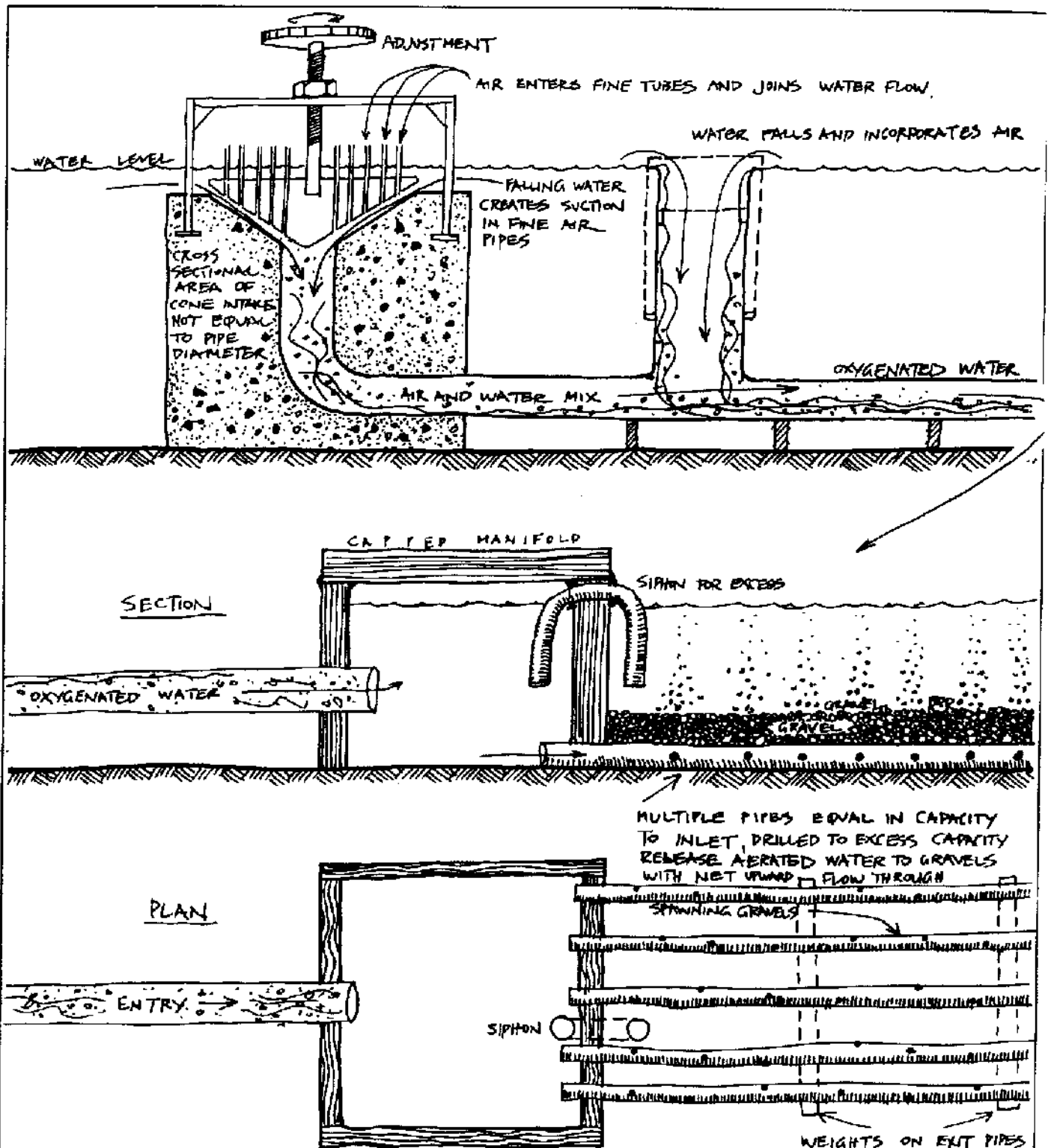
FIGURE 13.7 CONE AERATOR
