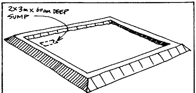
FIGURE 13.6 FISH REFUGES Deep "kettles" in a shallow pond can prevent fish dying in freezes, of excessive heat, or from accidental pond water loss; they also assist capture in draw-down conditions.
