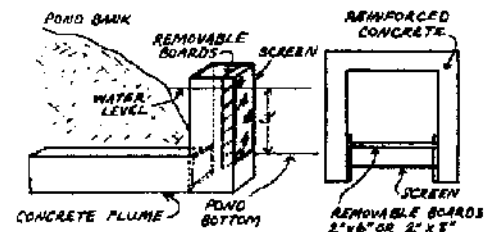
POND CONSTRUCTION
