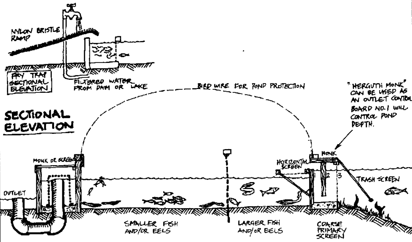
FIGURE 13.15 DOWNSTREAM AND UPSTREAM TRAPS. Both of these may be essential, e.g. in eel or mullet culture, or to harvest extensive swamps. Adults are held in a capture cage, fry
