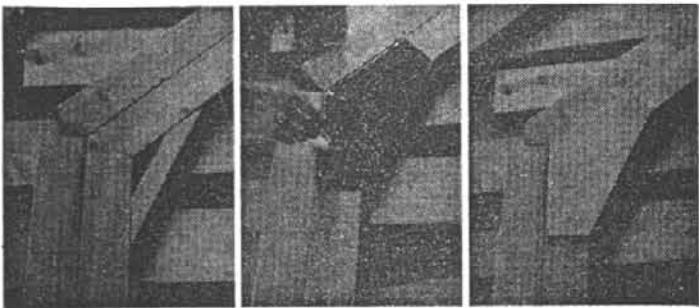
A rigid frame formed in a jig with plywood gussets being glued and nailed over the joints. Note the filler block which may be cut from a 2" x 2" (shown) or 2" x 4" member. Fourpenny nails secure the gussets until the glue dries.
