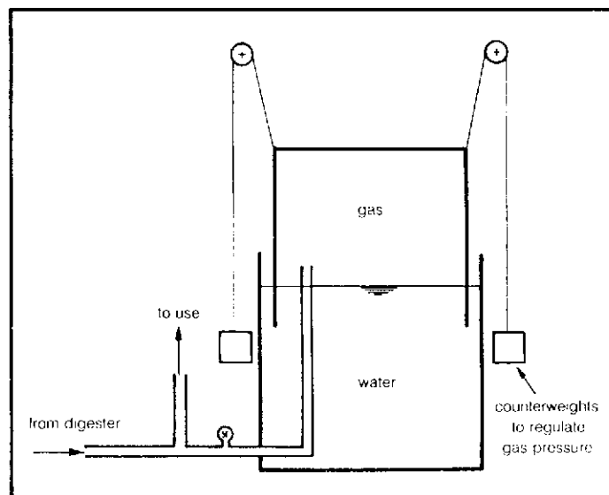
Figure 5.11 Floating-cover gas collection tank.
