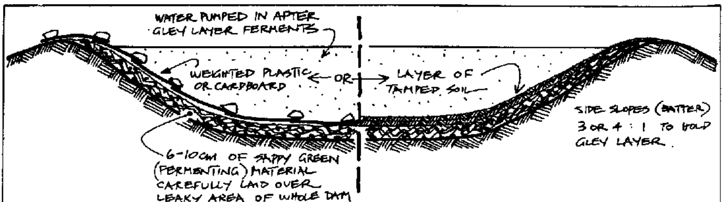
FIGURE 7.19 GLEYSING A POND
