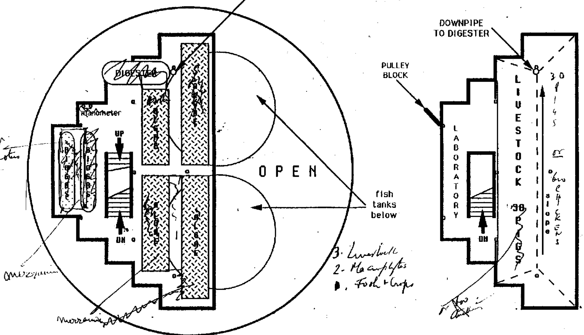
3RD LEVEL PLAN
