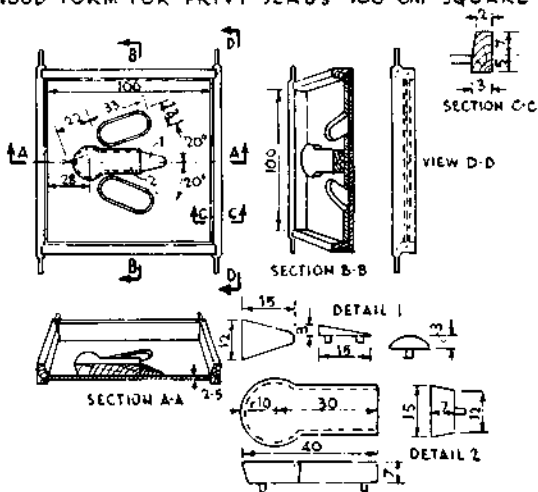
Figure 5.4 Privy floor details.
