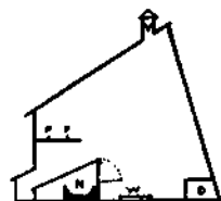
FIG. 201. House and yards for confined fowls: This house is so arranged as to be easily cleaned from the outside, the droppings falling into a trough at the rear, the floor under the roost being on an incline. C, Incline; P P, roosts; N N, nests; D, dust box; W, water trough; V, ventilator.
