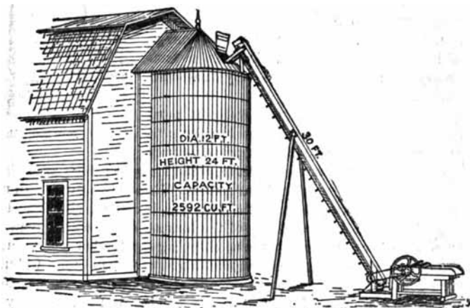
FIG. 169. Stave silo, 12 feet diameter, 24 feet high; capacity, 50 tons. (Eliass.)
