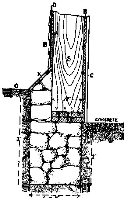
Fig. 167. Foundation of silo. Bottom of silo one foot below ground. (Cook.)
