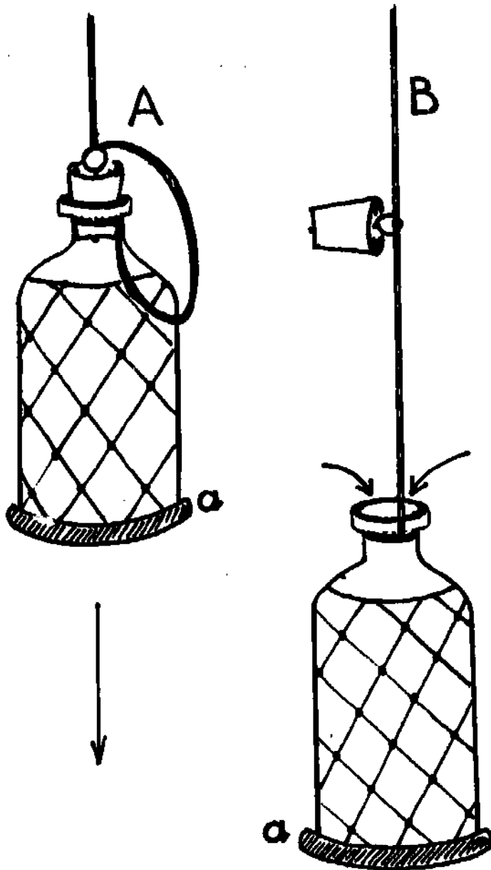
Fig. 24 Neyer's bottle for collecting water samples from different depths. A. Closed bottle B. Bottle opened under water with a jerk of the rope, a. weight fixed to the bottom of the bottle (preferably of lead).
