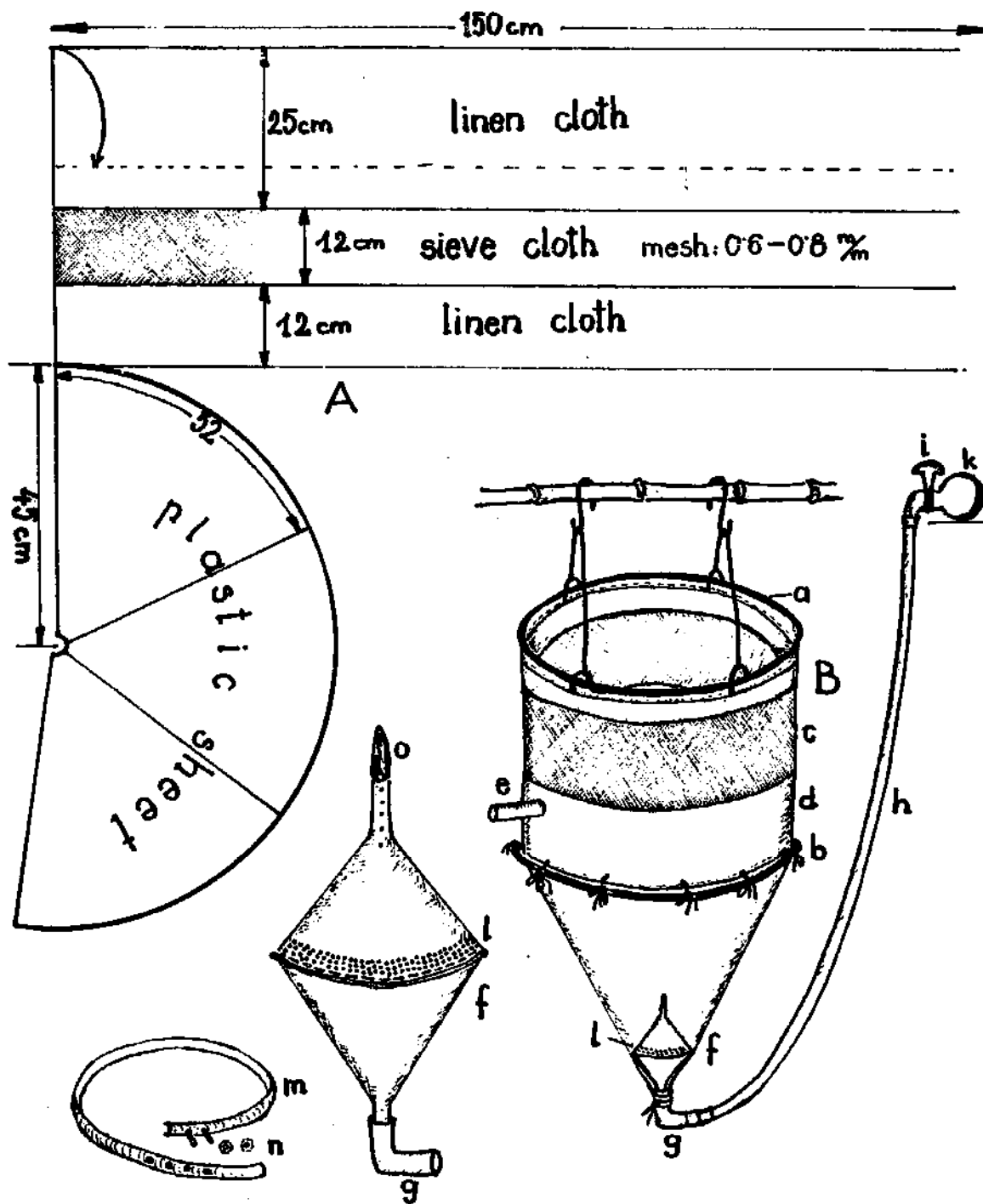
Fig. 45 Sieve-cloth plastic funnel. A. Dimensions of a medium size funnel. B. Parts of the funnel. a. cane ring, b. stretching ring, o. sieve cloth, d. linen cloth, e. nozzle, f. water distributor, g. elbow, h. water supply pipe, i. tap, k. water main, l. rows of holes on the water distributor, m. ring of split plastic pipe to keep the water distributor in position, n. screws and nuts, o. plug on the top of the water distributor.
