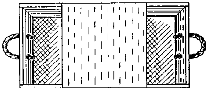
Fig. 60. Bait-Box complete, with cover in position upon which the bait is dissected.
