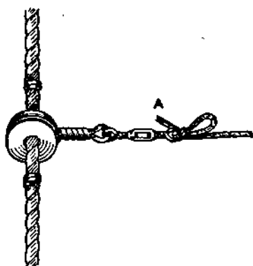
Fig. 87. Revolving Head-Link completed and placed upon the line, being kept in position by a coil or two of copper wire on either side. By pulling at the end A the snood is quickly unfastened.
