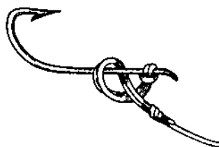
Fig. 10. Attaching a Gut Loop to a Hook, formed by a "lark's-head" knot as before, and a single half-hitch with both parts brought over the bend.
