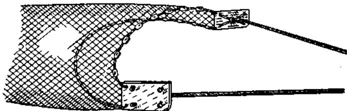
Fig. 98. Otter-Trawl, showing mouth of the net and portions of Bridle.
