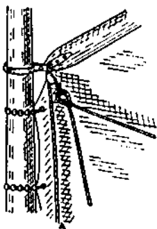
Fig. 101. Tricing-up the Mainsail for convenience in Ground-Fishing. A is the tricing-line attached to the clew of the sail and passing over small pulley-block. The Gaff is then lowered and secured, with the sail, around the mast.
