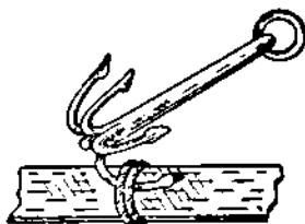
Fig. 102. Method of bending the claw of a "creeper" into its original form.
