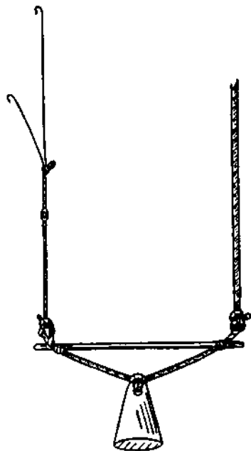
Fig. 20. Dartmouth Rig complete, showing spreader to which the sling holding the lead is lashed. The snoods descend parallel to the main line, as here shown.
