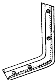
Fig. 121. Galvanised iron bracket screwed to front bar of Strand-Net.
