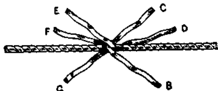
Fig. 115. Short Splice, showing the strands unlaid and placed together for working.
