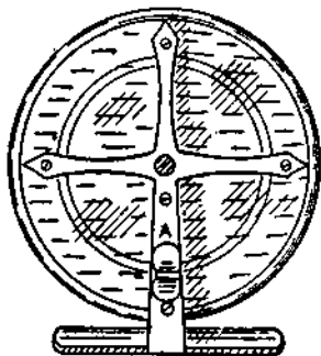
Fig. 24. Nottingham Reel, showing the back. By pushing the bolt A downwards, the check is released.
