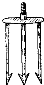
Fig. 128. Fish - Spear: the upper screw fits into a brass socket at the end of a long pole.
