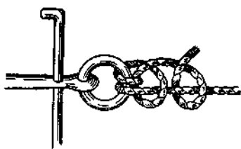
Fig. 110. Anchor Bend, showing end of rope fastened to ring, with the turns slack.
