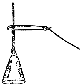
Fig. 69. Plummeting Gear, showing conical lead attached by spliced loop, and boom above it; also portion of Snooding connected to smaller extremity of boom.
