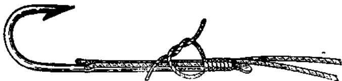
Fig. 54. "West Country Whipping" for Cod or Conger Hook, the snood being attached by tying a single overhand knot above and below, finishing off with a reef knot
