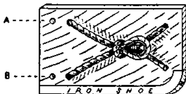
Fig. 97. Otter-Board, showing inside with method of fitting it. The Bridle is attached to the outer eye of the rope, and the head and foot ropes are passed through the holes A and B respectively.
