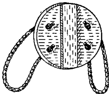
Fig. 119. Cover of Store-Pot, showing method of attaching ropes for retaining it in position.
