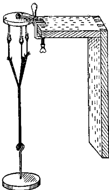
Fig. 72. Spinning-Jack, clamped on to wood, showing leaden weight depending from horsehair length being spun up. The lower portion of wood should be fixed firmly in the vice of a carpenter's bench.
