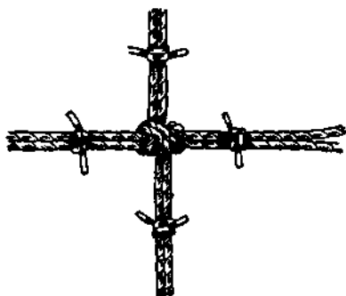
Fig. 125. Cords across the centre of Baited Prawn-Net enlarged, and showing the four pieces of twine knotted to form "sliders" for holding bait.
