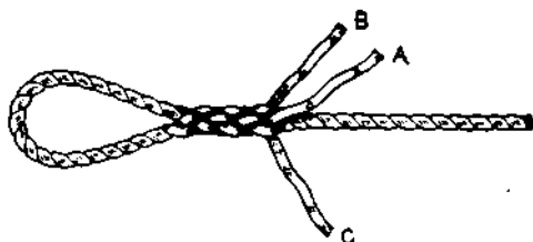
Fig. 114. Eye-Splice completed, before cutting off the ends.
