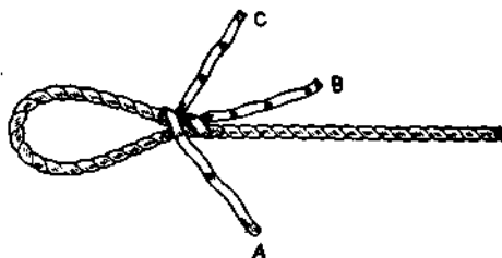
Fig. 113. Eye-Splice commenced, with middle strand B introduced.
