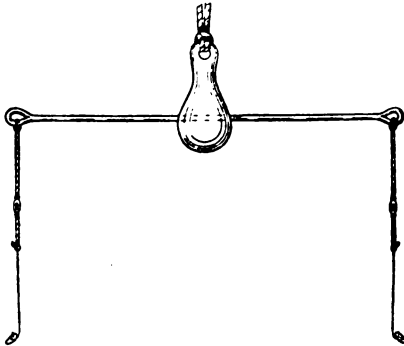
Fig. 19. Southampton Rig, consisting of a pear-shaped, or conical lead and a transverse bar of brass wire with short snoods fastened to each of the eyes.
