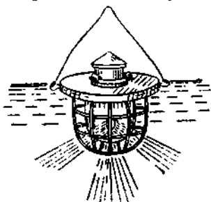
Fig. 130. Floating Lamp for attracting large Mullet or other fish at night-time.
