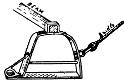
Fig. 95. Trawl-Head, or Iron runner, with portion of Beam and Bridle.
