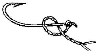
Fig. 9. Attaching Two-stranded Snooding to a Hook, performed by making a "lark's-head" knot upon the shank, and then passing a single half-hitch over the bend.
