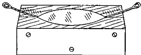
Fig. 14. Wooden Mould, screwed together, containing boat-shaped lead.
