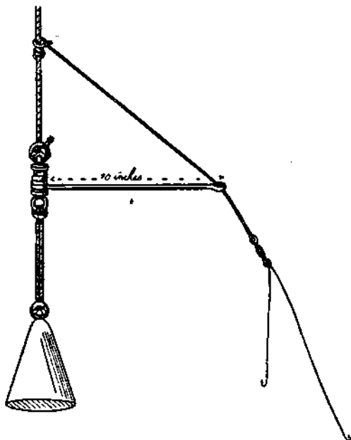
Fig. 17. Improved Rig for Deep-Sea Fishing, complete, showing boom revolving upon brass reel, and lead attached by independent piece of line.
