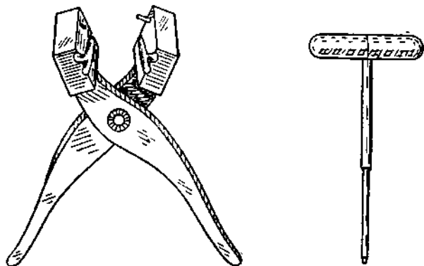
Fig. 16. Brass Mould for Casting Pipe-Leads (open); also Pin for inserting before pouring in the lead.
