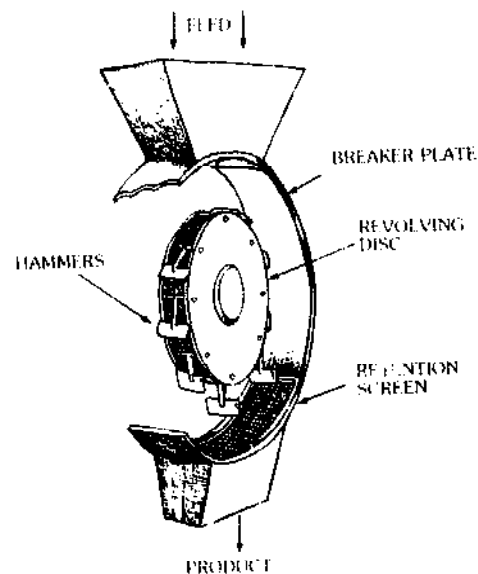
Hammer Mill
