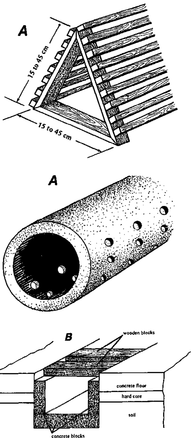
Figure 39. Lateral duct design. A -- Above ground. Slatted triangular duct (may also be square or rectangular or a round tube with numerous air holes). B -- Below ground. Sunken concrete duct. (From Control of Environment, Part 2, Potato Marketing Board, Sutton Bridge Experimental Station, Report No. 6, London ).
