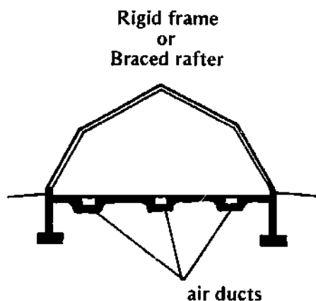
Figure 24. Above-ground large-scale stores. (From Bulk Potato Storage , Agriculture Canada Publication 1508, Canada Department of Agriculture).
