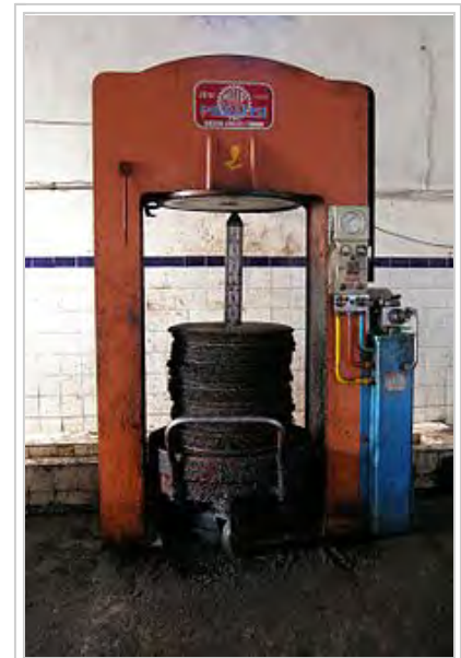
Press with stack of fiber disks
