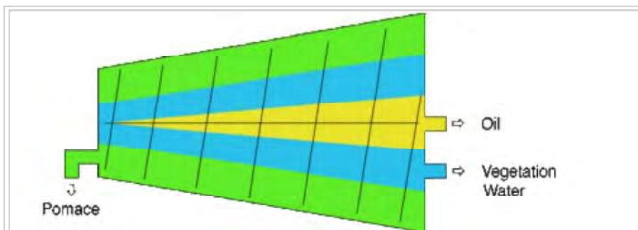
Diagram of a working decanter. The three phases are separated according to their densities.
