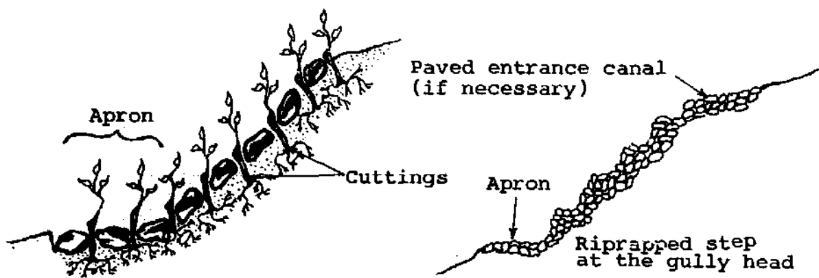
Fig. 44: Stabilization of a gully head by riprap
