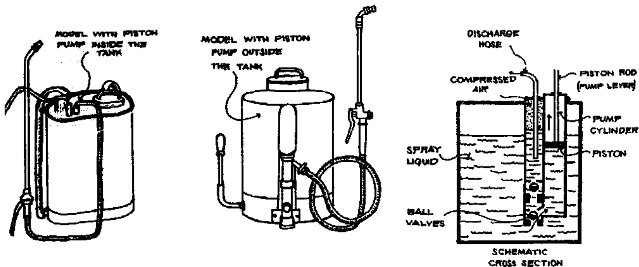
Fig. 56: Knapsack sprayers with piston pumps (Adapted from Lambrecht, 1967)
