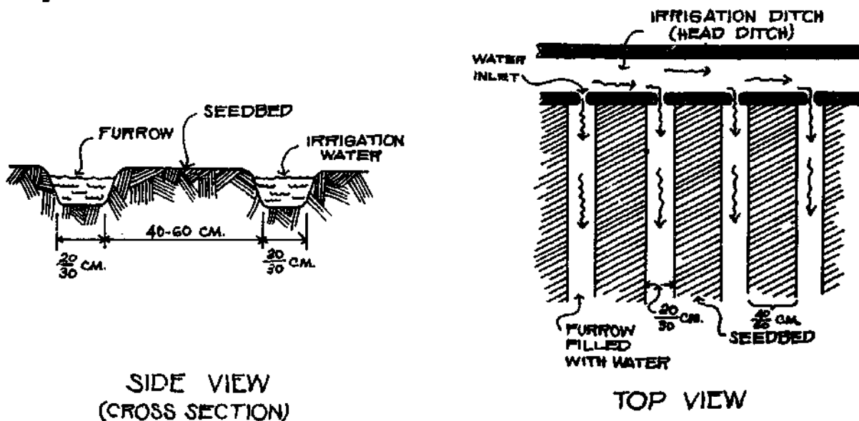
Fig. 7: Furrow irrigation
