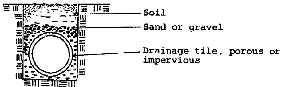
Fig. 14: Tile drainage
