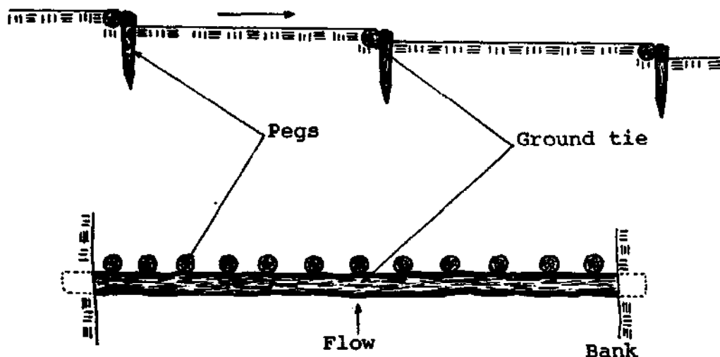
Fig. 73: Construction of a ground tie
