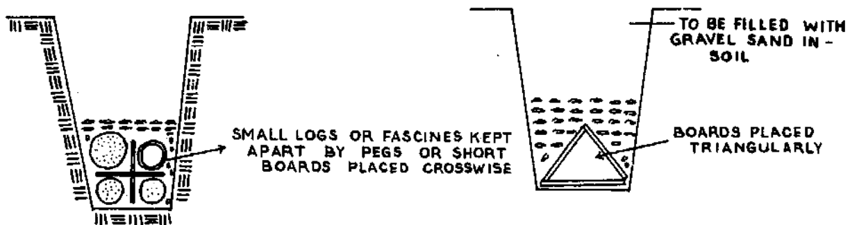
Fig. 16: Temporary drainage
