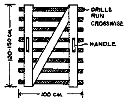
Fig. 13: Marking board
