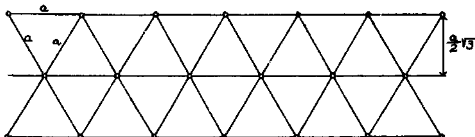
Fig. 7: Equilateral spacing
