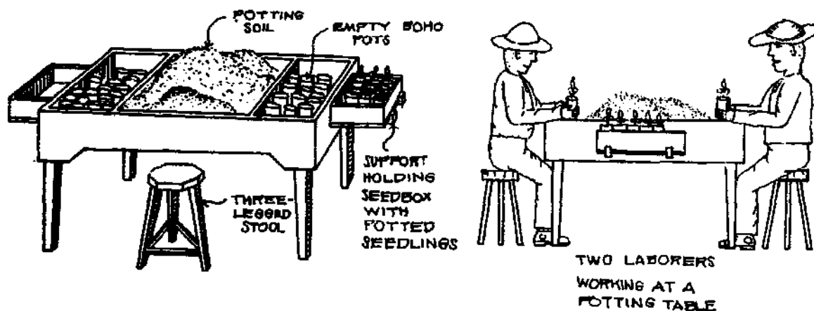
Fig. 27: Potting table
