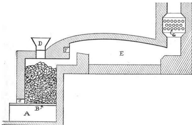
FIG. 12. — EBELMEN GAS-PRODUCER.
