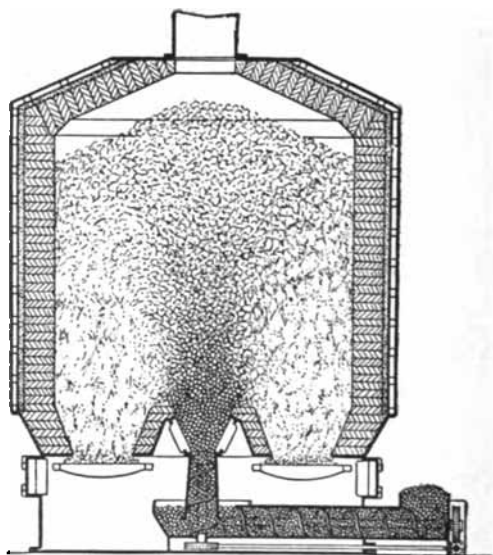
FIG. 106. — SECTION OF CAPITAINÉ SOFT-COAL PRODUCER. (Courtesy of Engineering Magazine .)
