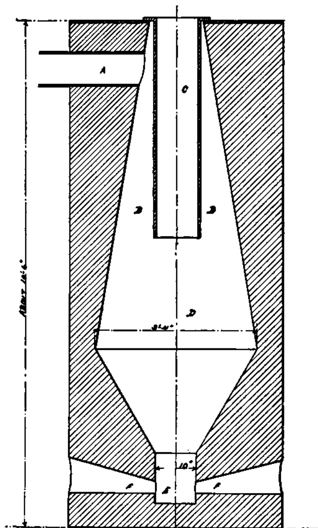
FIG. 13. — EBELMEN PRODUCER.
