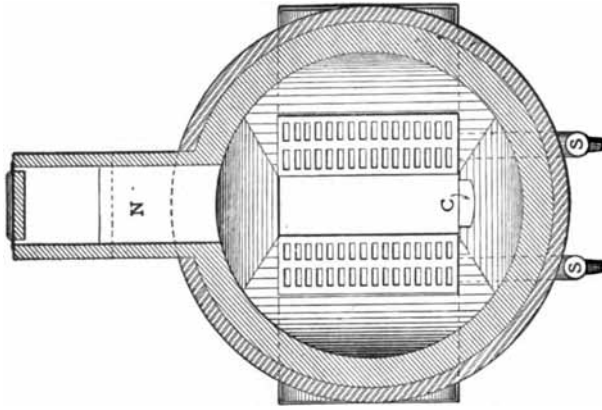
FIG. 28. — SWINDELL GAS-PRODUCER.
