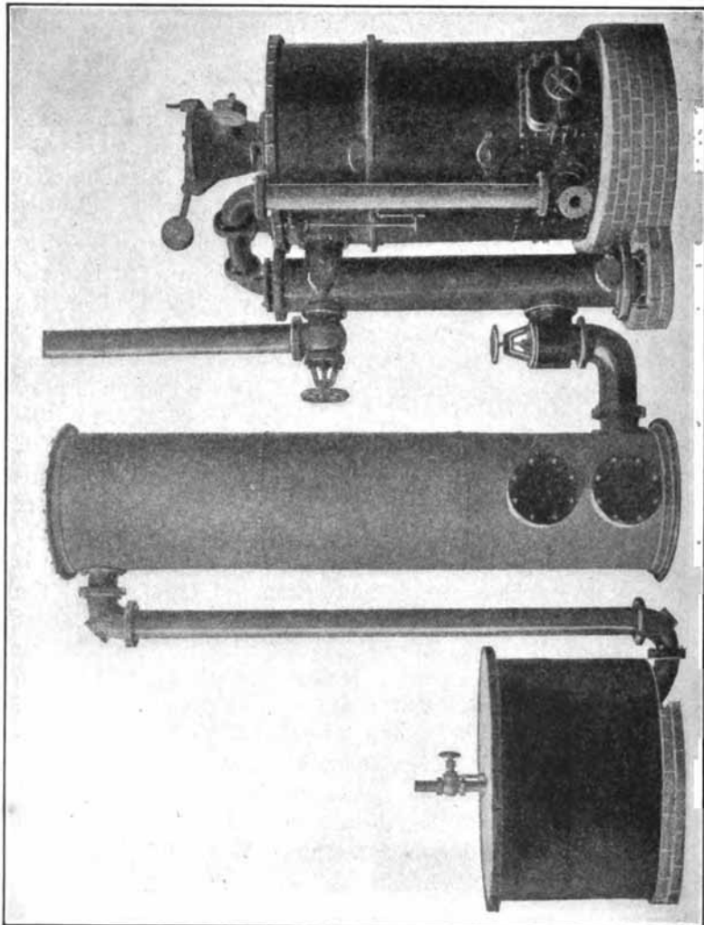
Producer. Vaporizer. Scrubber. Purifier. Fig. 51. — WOOD SUCTION GAS-PRODUCER.
