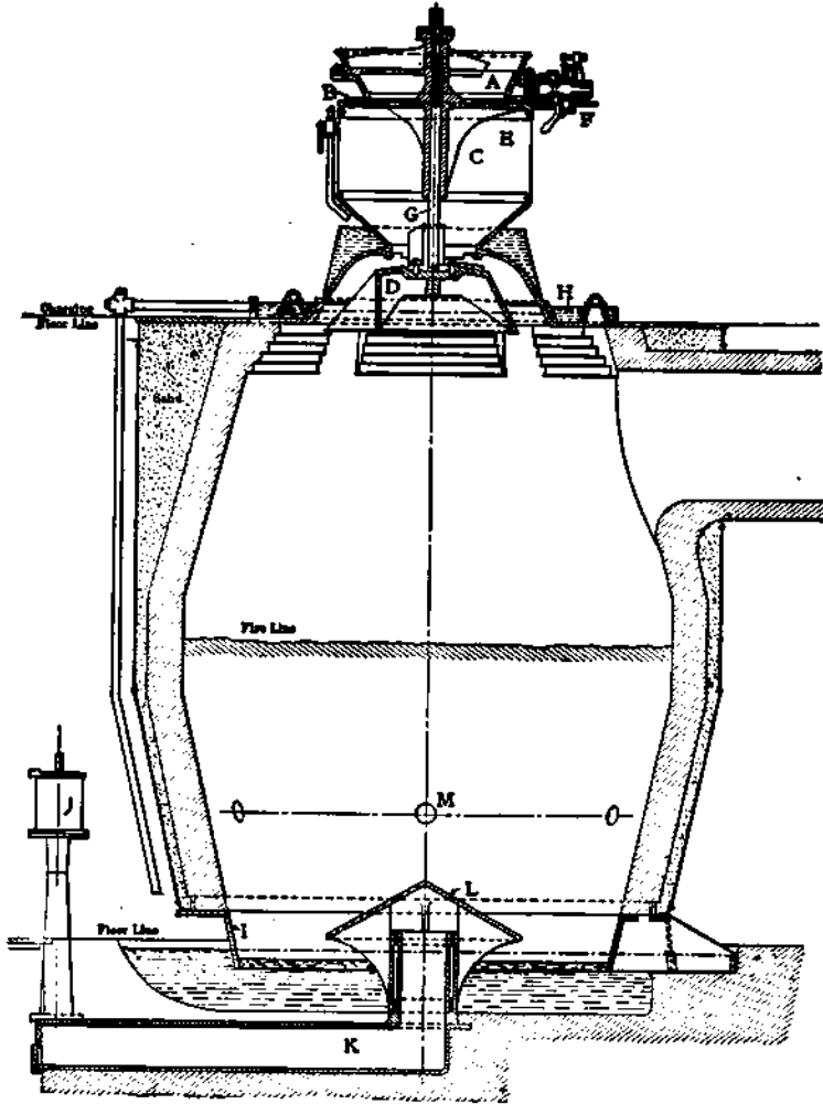
FIG. 44. — SECTION OF MORGAN GAS-PRODUCER EQUIPPED WITH BILTZ AUTOMATIC FEED.
