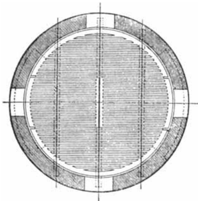
FIG. 39. — SECTION OF WOOD FLAT-GRATE GAS-PRODUCER.
