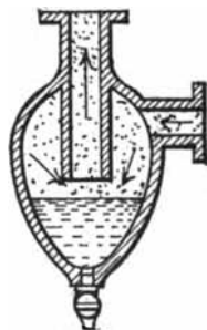
FIG. 74. — MOISTURE COLLECTOR.
