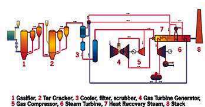
Figure 8. TPS Termiska Flow Sheet
