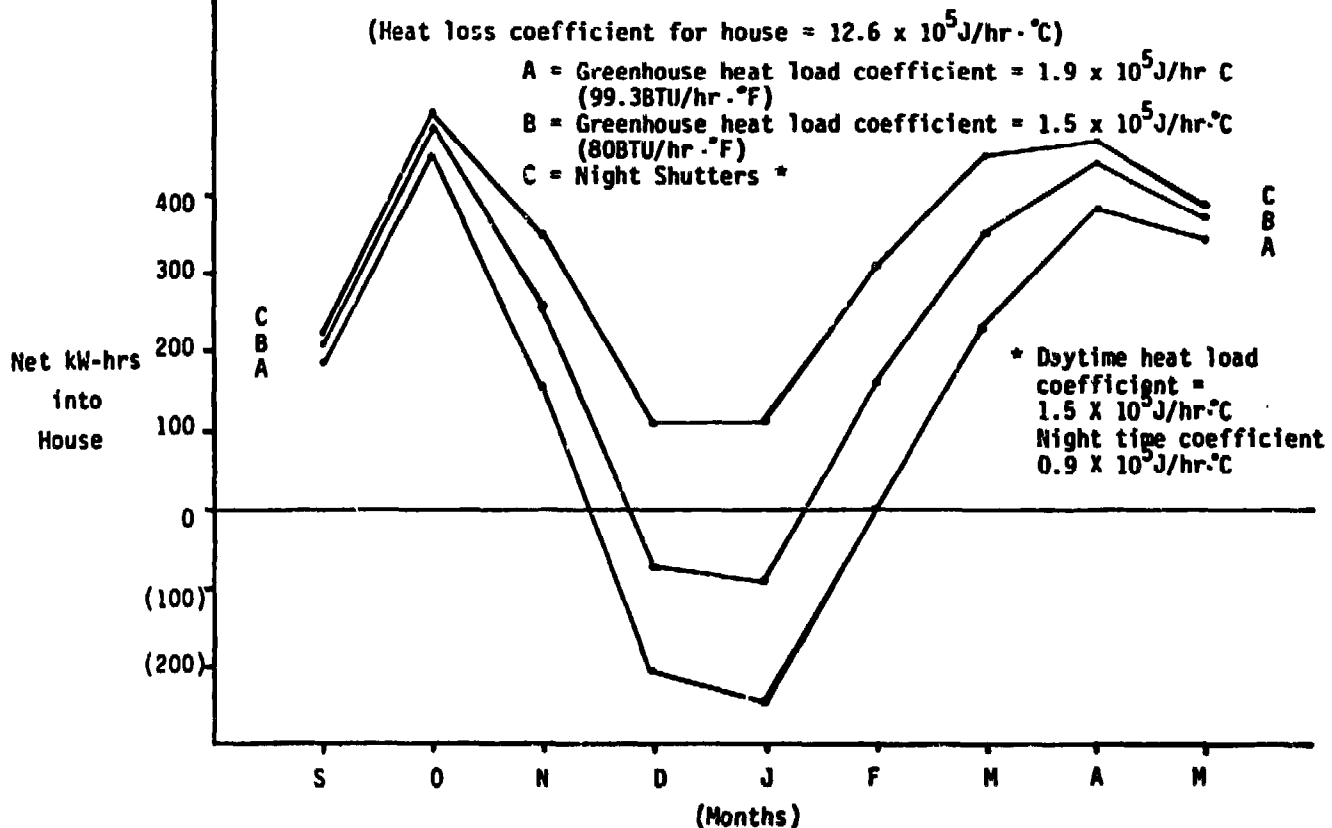
Figure 3 SIMULATED MONTHLY PERFORMANCE OF A PROTOTYPE GREENHOUSE IN BURLINGTON, VT., USED TO HEAT A HOUSE
