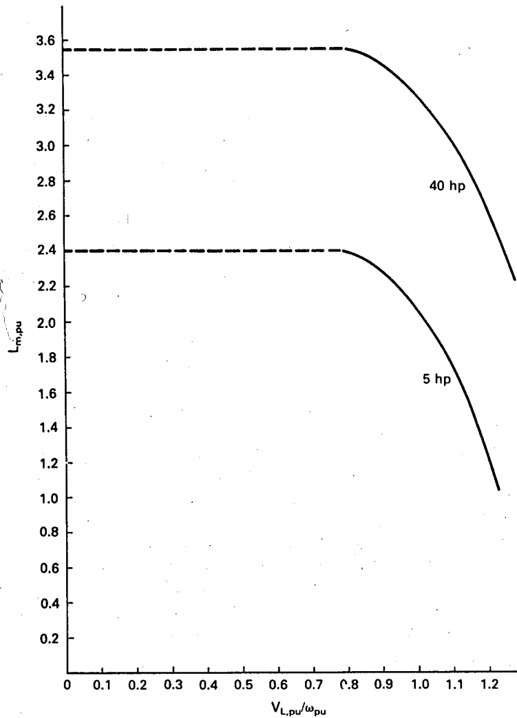
Figure 13: Per unit magnetizing inductance as a function of load voltage.
