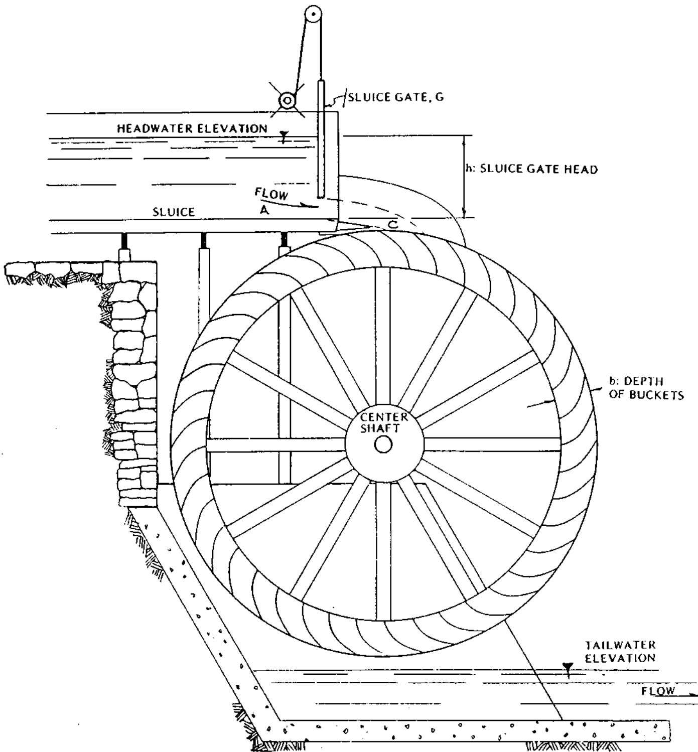
FIG. 11A OVERSHOT WHEEL
