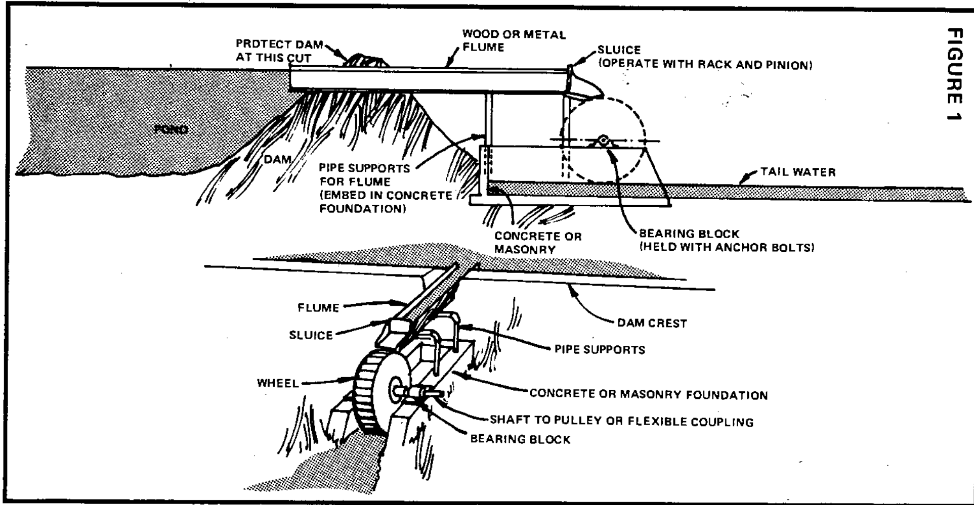
As the head of a water power system rises or falls, the sluice gate may be adjusted to meter the correct flow to the wheel.
