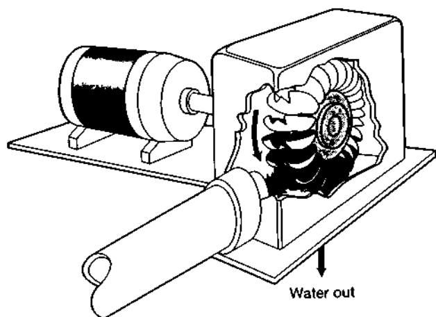
Figure 15. Single-jet Pelton turbine
