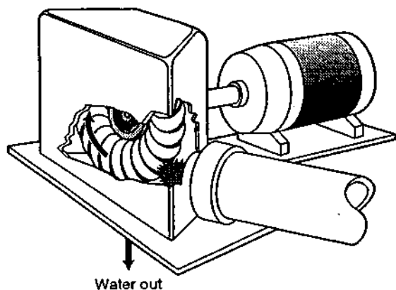
Figure 14. Turgo turbine
