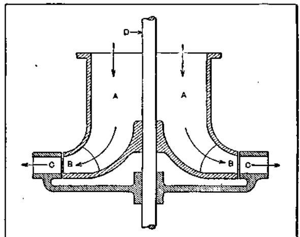
Fig. 13. Section of Fourneyron Reaction Turbine
