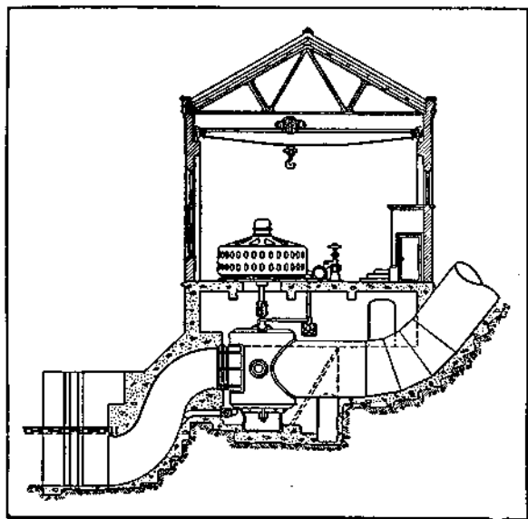
Fig. 32. High-head Vertical Turbine Installation
