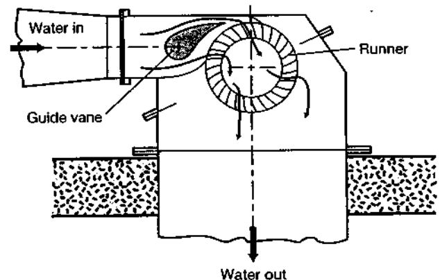
Figure 13. Crossflow turbine
