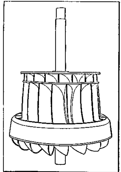
Fig. 12. Mixed-flow Turbine
