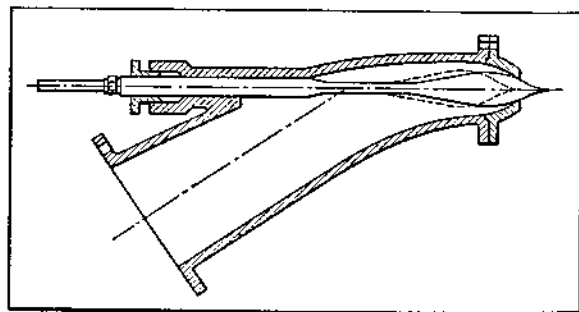
Fig. 20. Sectional View of Pelton-Doble Needle Nozzle
