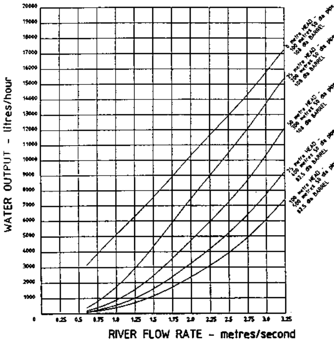
1.5m TYSON TURBINE - WATER OUPUT PREDICTIONS
