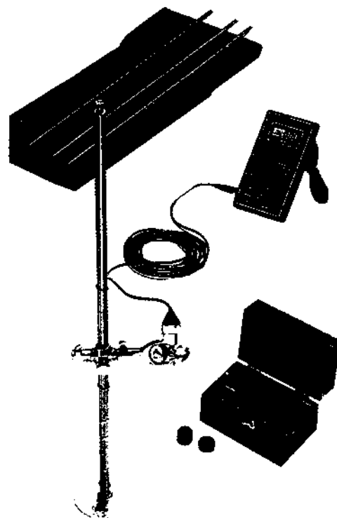
▲ PYGMY FLOW METER WITH DIGITAL FLOW INDICATOR
