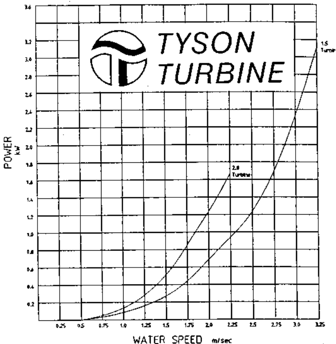
TYSON TURBINE ELECTRICAL PERFORMANCE PREDICTIONS
