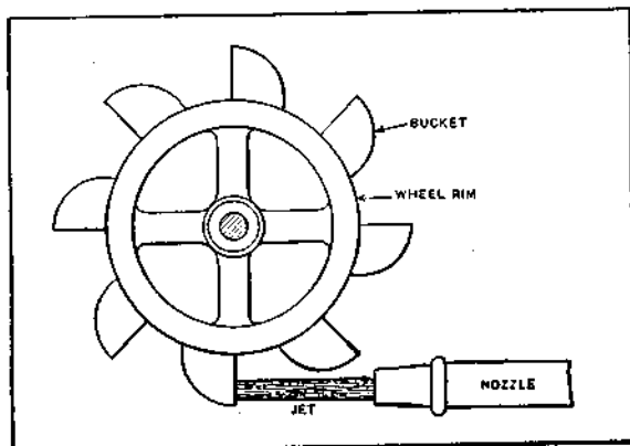
Fig. 7. Pelton Wheel
