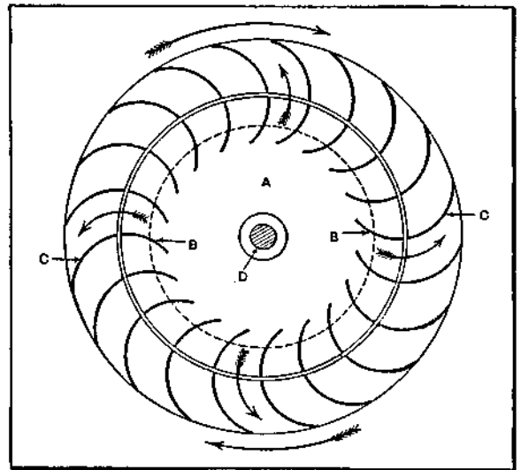
Fig. 11. Fourneyron Reaction Turbine
