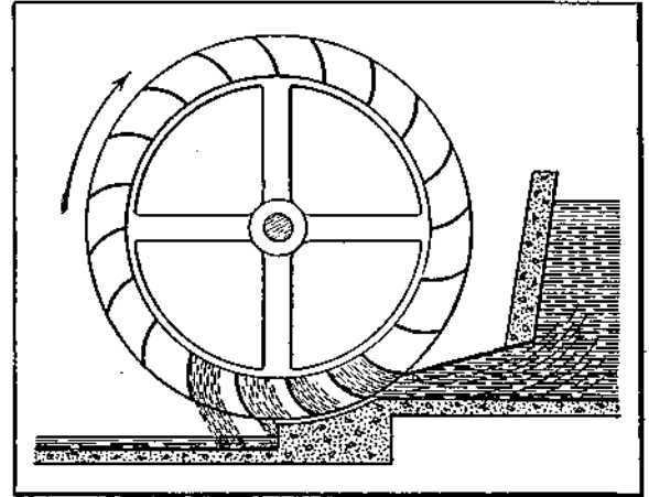
Fig. 4. Poncelet Water-wheel
