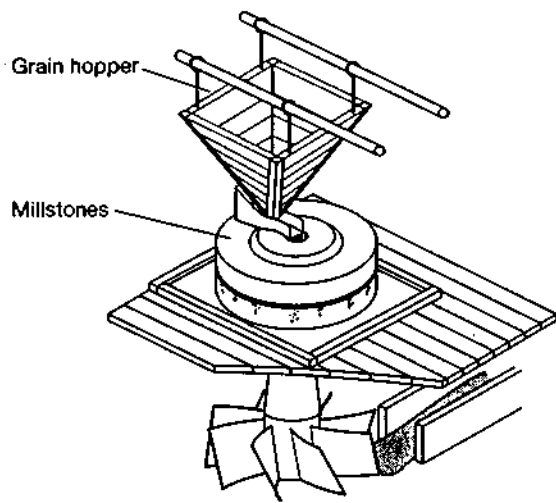
Figure 2. Norse wheel or ghatta, used for milling
