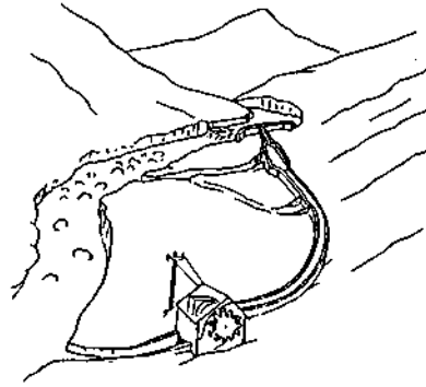
(c) Low head with channel
