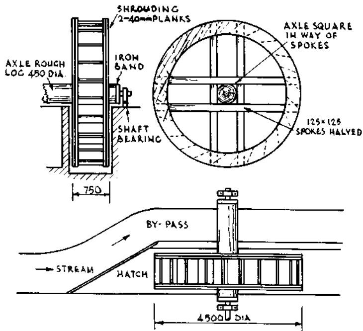
Figure 7.4 Undershot wheel.
