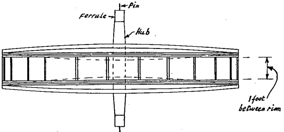
ELEVATION : scale \frac{1}{2}'' = 1'
