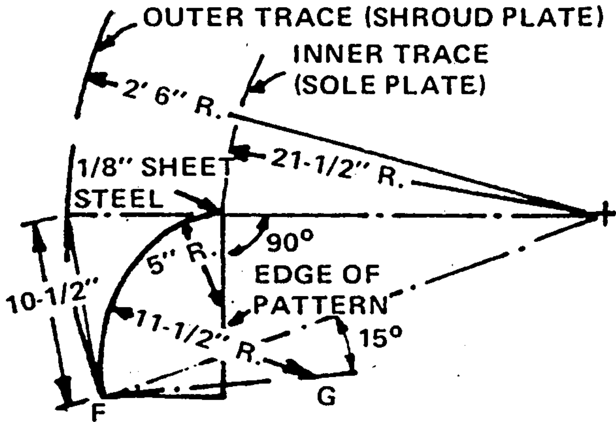
STEEL BUCKET LAYOUT 22 BUCKETS REQUIRED
