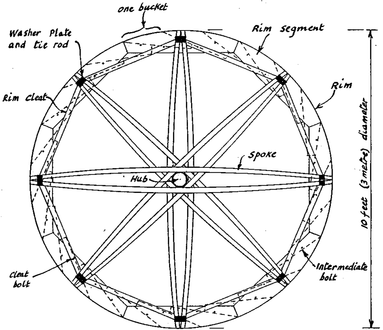
ELEVATION : scale \frac{1}{2}'' = 1'
