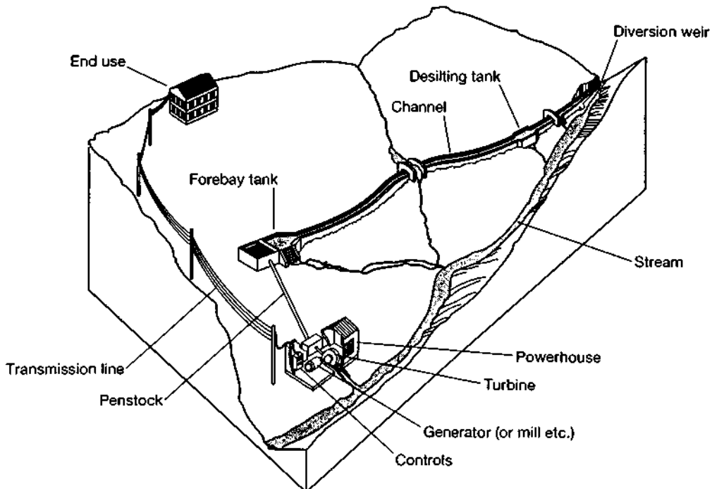
Figure 3. Components of a micro-hydro scheme
