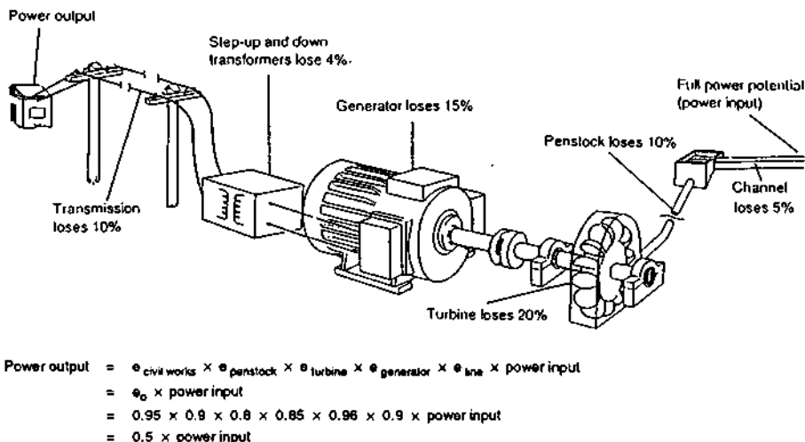
Figure 4. Typical efficiencies in a hydro system generating electricity (direct-drive mechanical applications have fewer inefficiencies)
