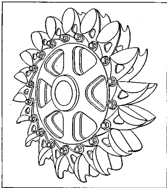
Fig. 16. Pelton Impulse Turbine Runner
