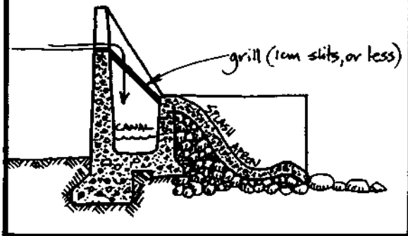
BARRIER DAM SECTION
