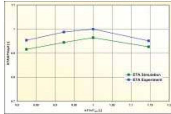
Fig. 4: Efficiency of a Pelton turbine: comparison of simulation and experiment.
