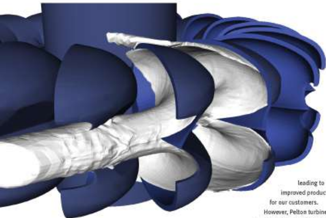
Fig. 2 (above): Free-surface water jet deformation as it interacts with three buckets, showing the water sheet leaving buckets.
