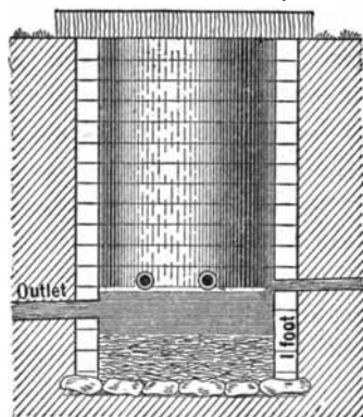
Fig. 14 - Silt Basin
