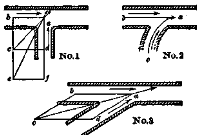
Fig. 20 - Junctions
