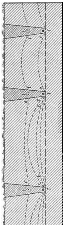
Fig. 15.—Cross-section showing the action of drains at different depths and distances apart upon retentive and unretentive soils.
