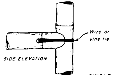
SINGLE BUTT JOINT
