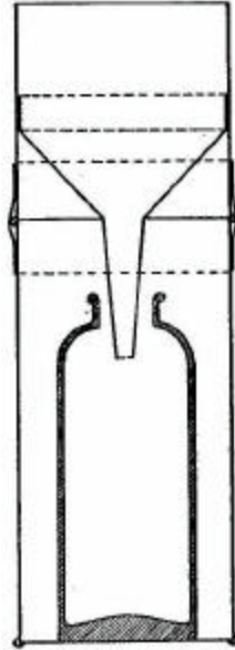
FIG. 152.—Section of home-made rain-gauge.
