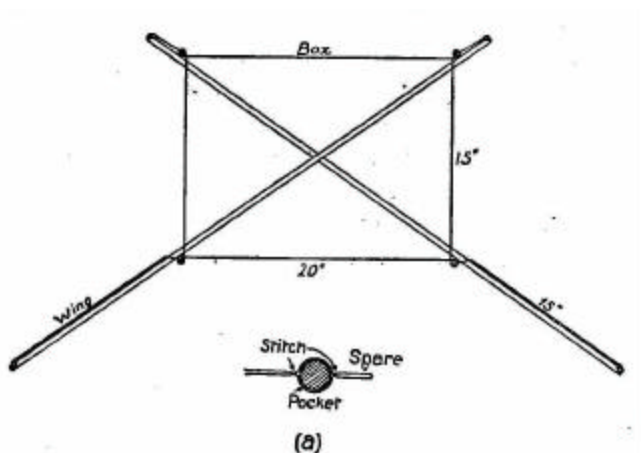
FIG. 119.—Plan of box kite with rear wings.
