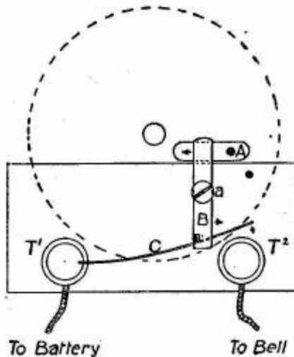
FIG. 89.—Plan of release gear of electric alarm, as attached to clock.
