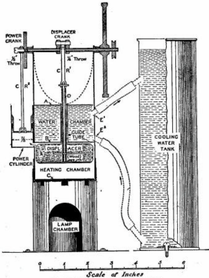
FIG. 97.—Vertical section of hot-air engine.
