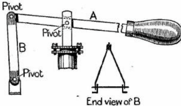
FIG. 111.—Details of lever for force pump.
