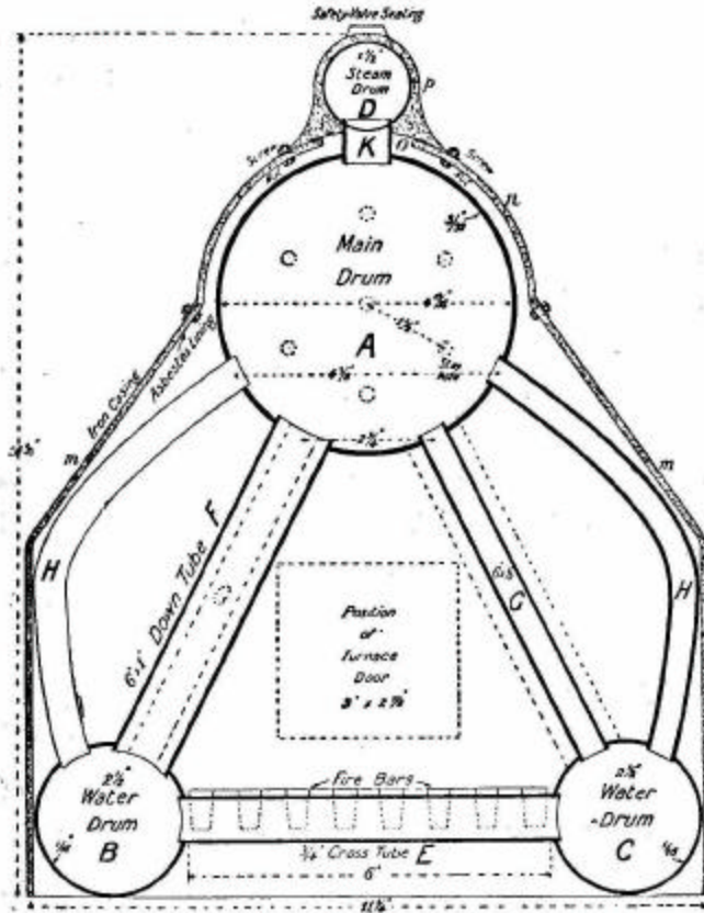
FIG. 86. -- Cross section of multitubular boiler.
