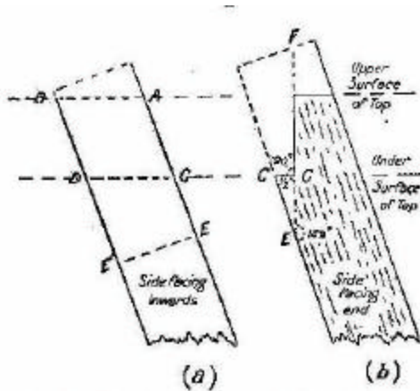
FIG. 2.—Showing how to cut sloping joint for trestle leg.
