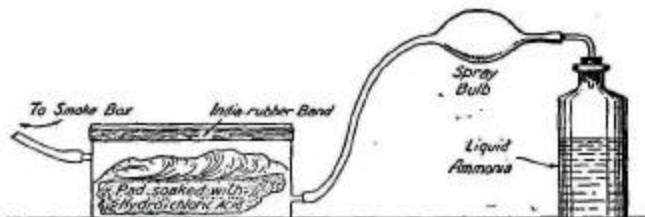
FIG. 150.—Smoke-making apparatus.
