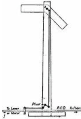
FIG. 46.—Double-armed signal, operated by points.
