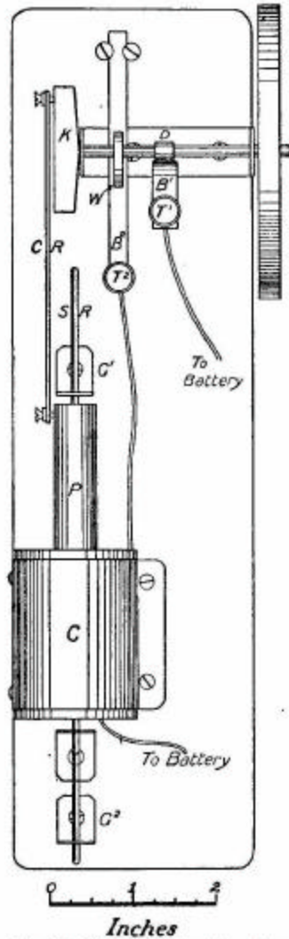
FIG. 38.—Plan of electric reciprocating engine.
