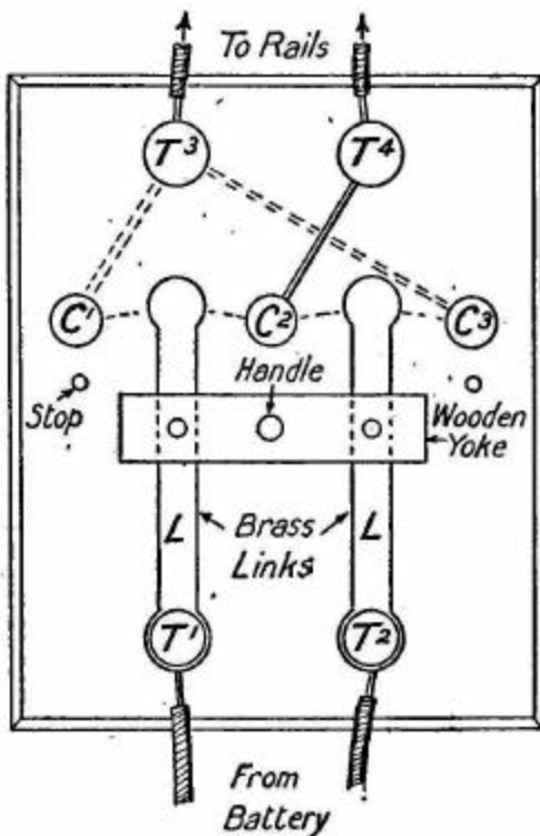
FIG. 48.—Reversing switch.
