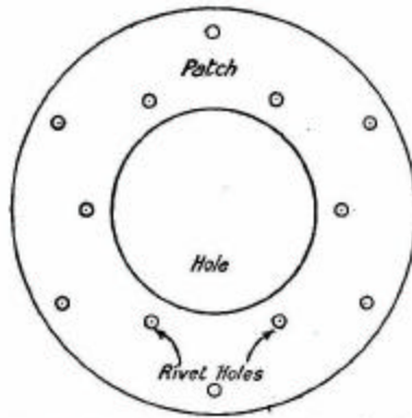
FIG. 85.—Showing how to mark out strengthening patch round steam dome hole.
