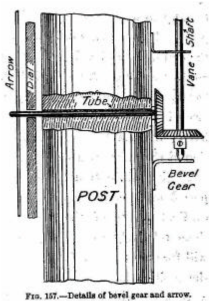
FIG. 157. -- Details of bevel gear and arrow.
