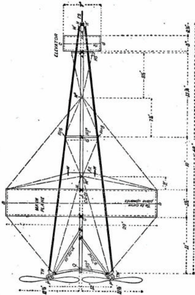
FIG. 133. -- Plan of model aeroplane.
