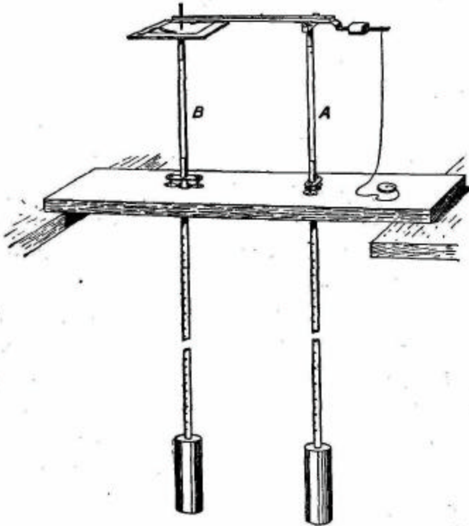
FIG. 168.—Simple Rectilinear Harmonograph.
