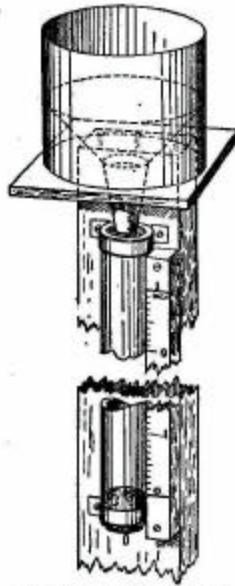
FIG. 153.—Self-measuring gauge.
