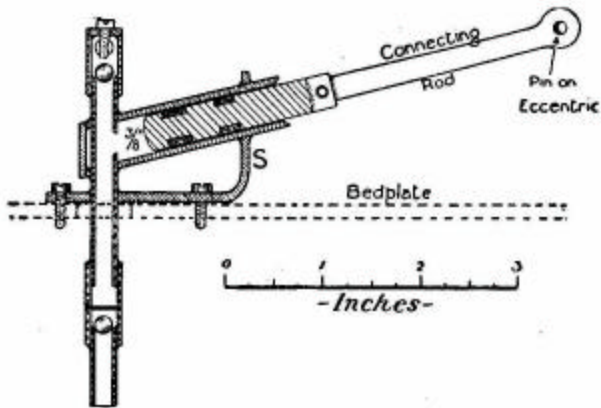
FIG. 66.—Vertical section of force pump driven by engine.
