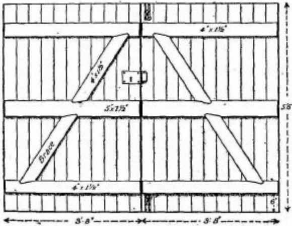
FIG. 22.—Doors of shed.
