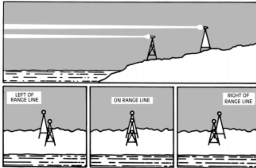
Figure 502. Range lights.
