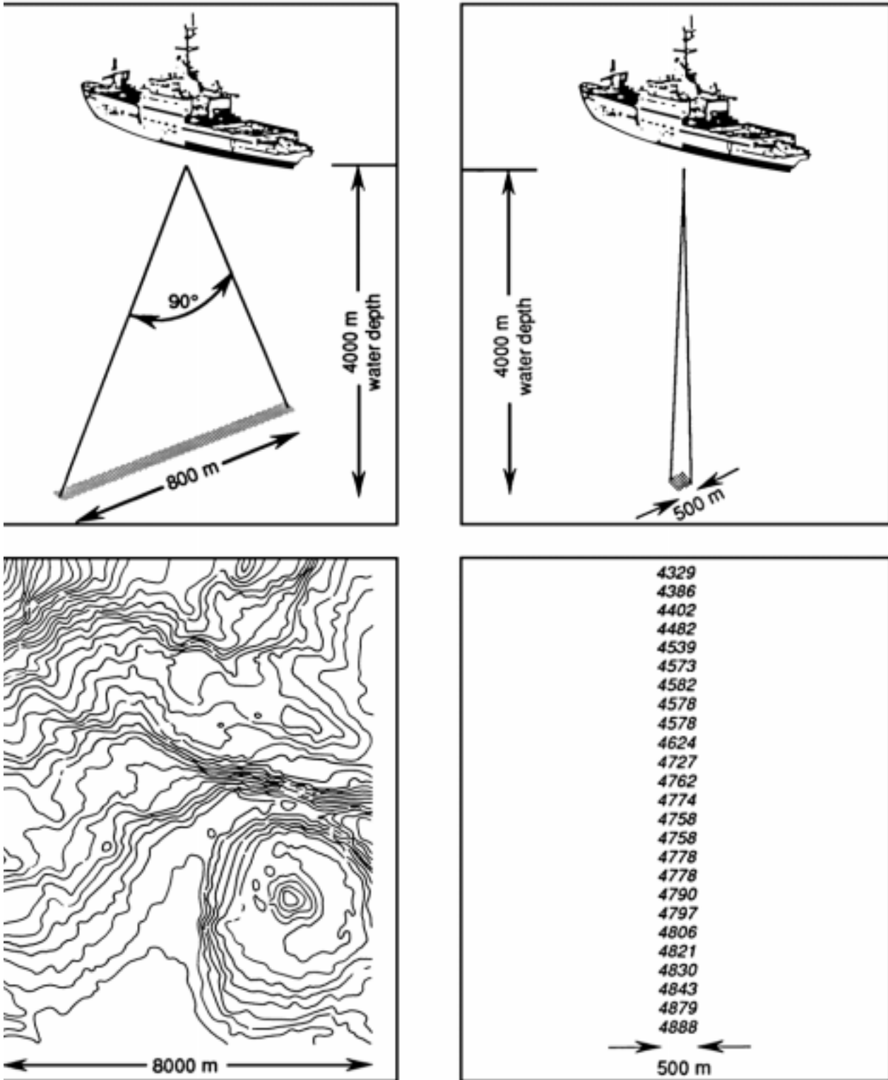
Figure 3005. Swath versus single-transducer surveys.
