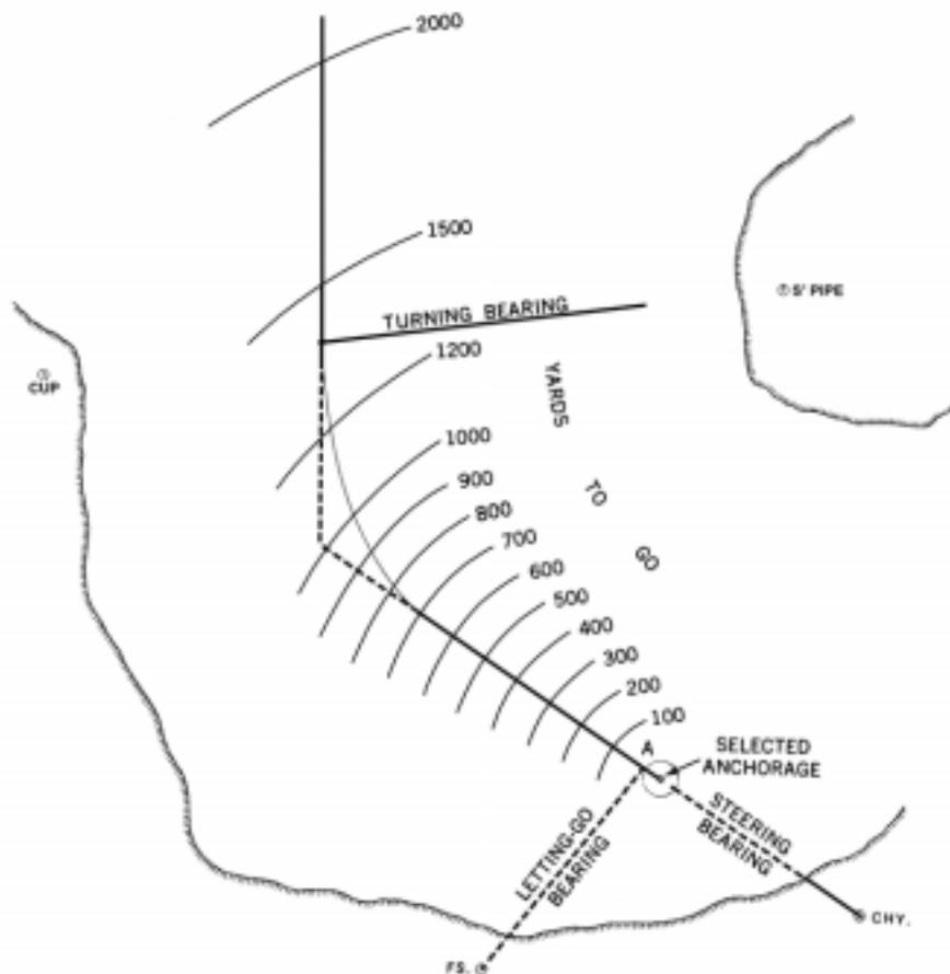
Figure 817. Anchoring.
