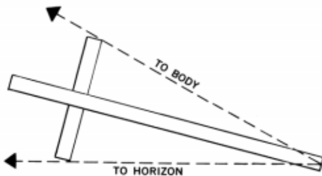
Figure 2608c. Improved cross-staff.
