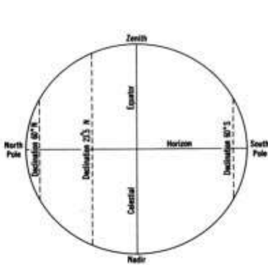
Figure 1516a. The right sphere.
