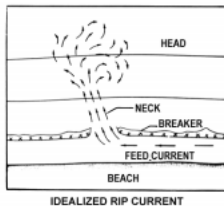
Figure 3319. A rip current (left) and a diagram of its parts (right). Courtesy of Robert L. Wiegell, Council on Wave Research, University of California.
