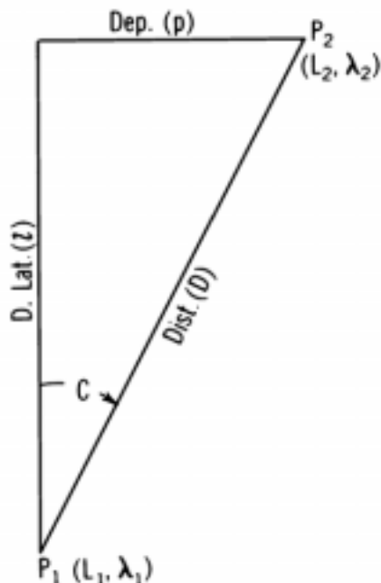
Figure 2206. The plane sailing triangle.
