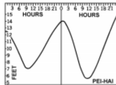
Figure 905b. Diurnal tide.
