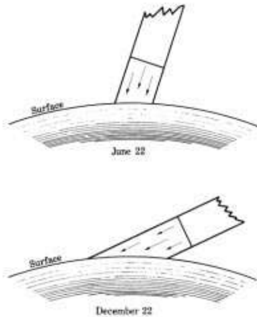
Figure 1519b. Sunlight in summer and winter. Compare the surface covered by the same amount of sunlight on the two dates.
