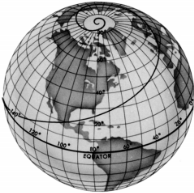
Figure 106. A loxodrome
