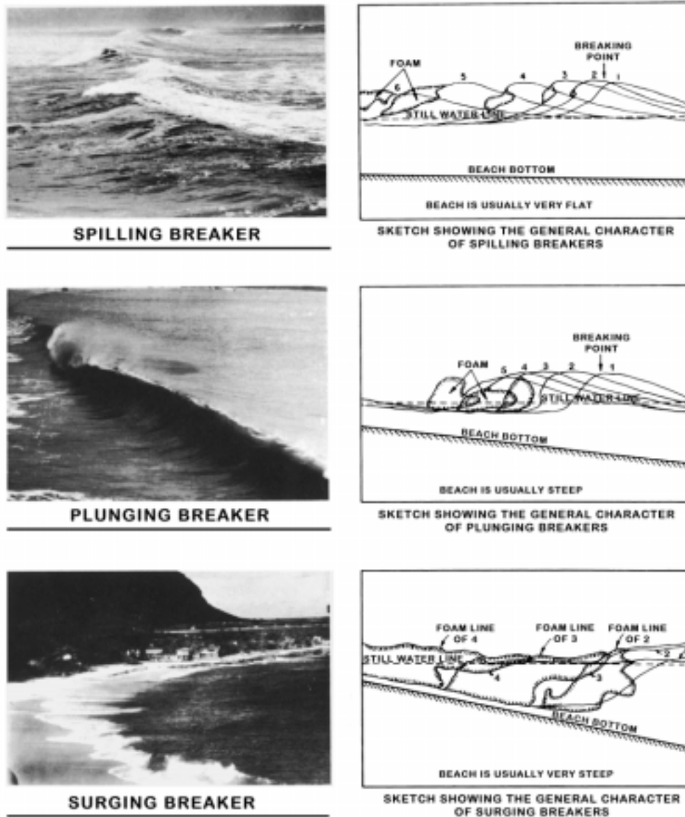
Figure 3317. The three types of breakers.
