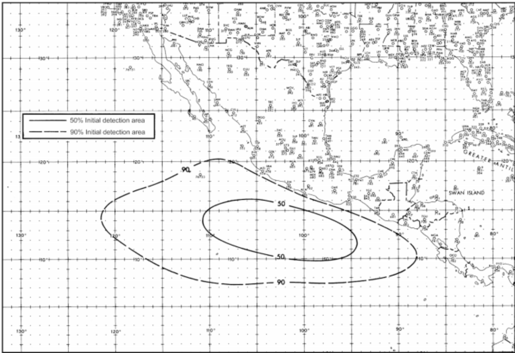
Figure 3804c. Area of initial detection of high percentage of tropical cyclones which later developed to tropical storm or hurricane intensity, 1957-1974.
