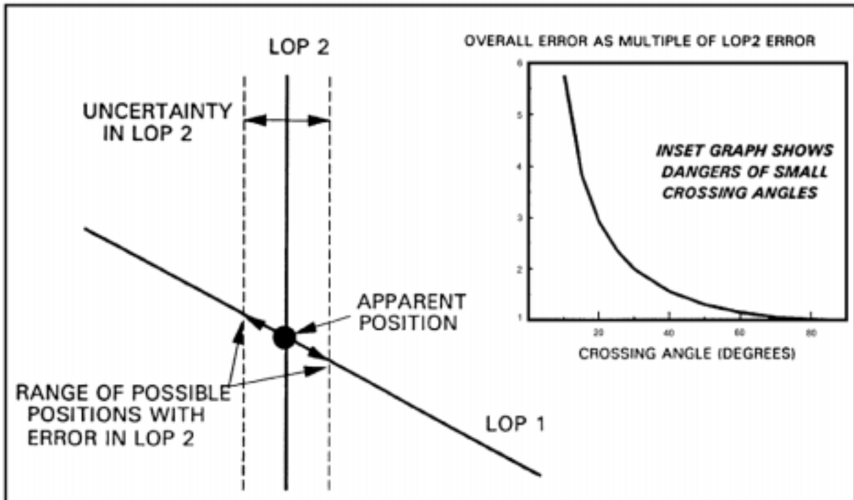
Figure 1206c. Error in Loran LOPs is magnified if the crossing angle is less than 90°.
