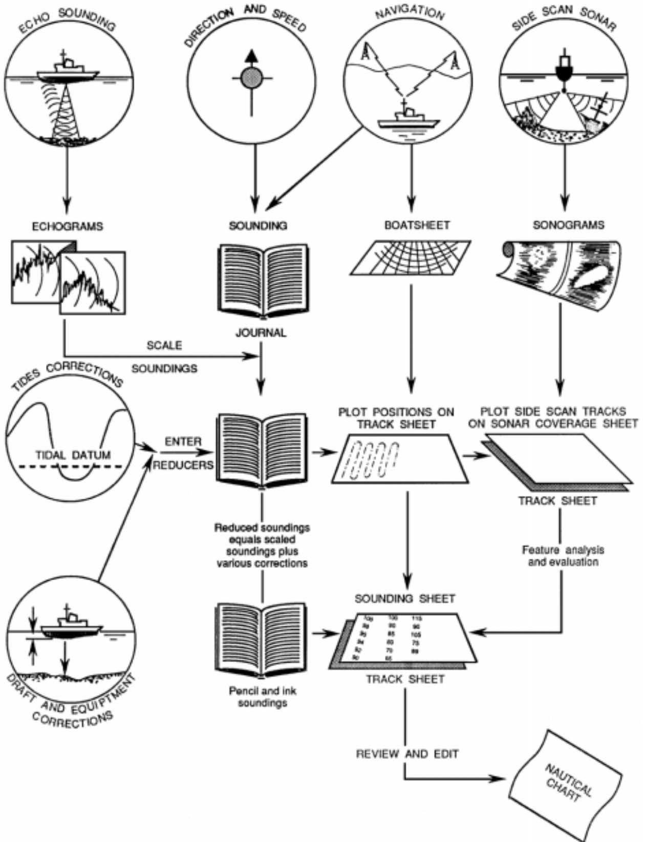
Figure 3004. The process of hydrographic surveying.
