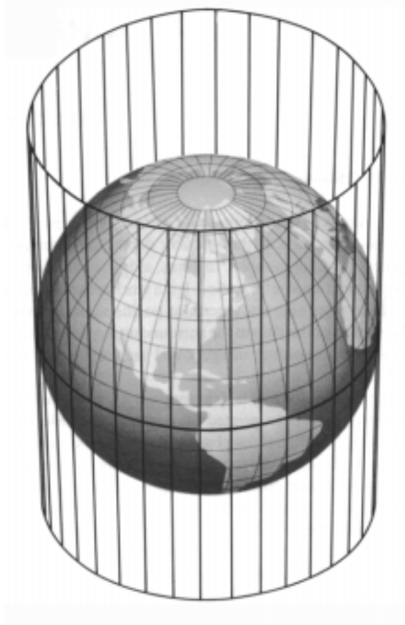
Figure 304. A cylindrical projection.
