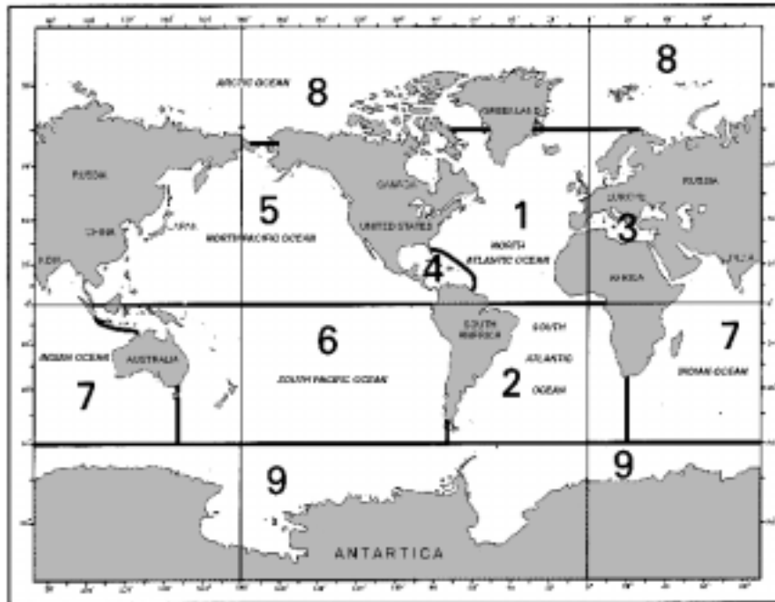
Figure 344a. Ocean basins with region numbers.
