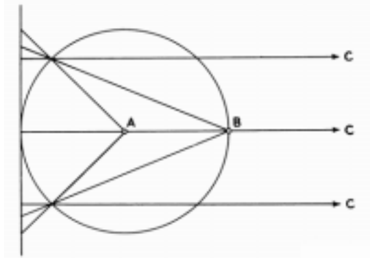
Figure 303. Azimuthal projections: A, gnomonic; B, stereographic; C, (at infinity) orthographic.
