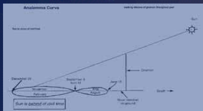
Figure #2, Building an analemma curve
