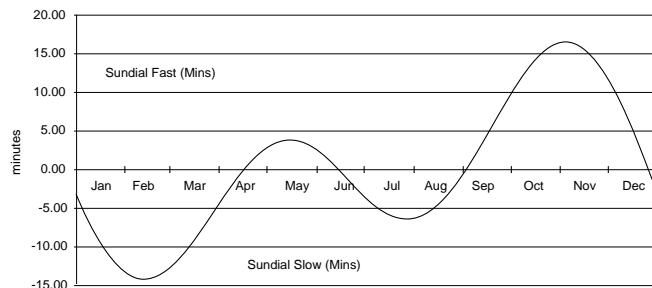
Correction for the "Equation of Time"
