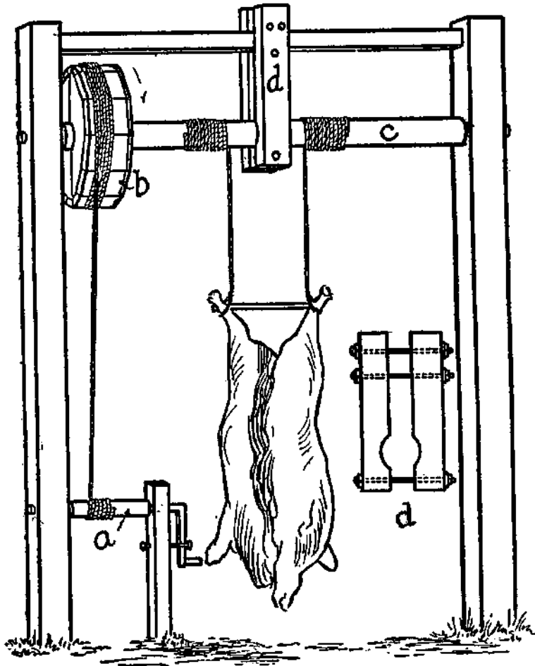
CARCASS DERRICK
