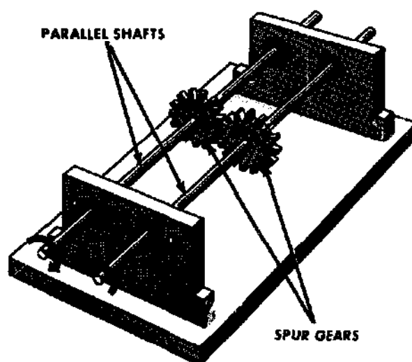
5.22.1 Figure 6-2.—Spur gears coupling two parallel shafts.
