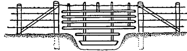
SUSPENDED GATE
