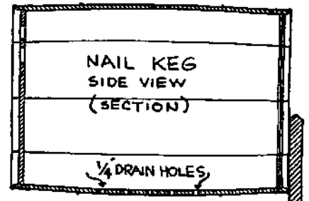
NEST BOX
