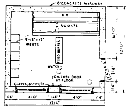
SHED TYPE POULTRY HOUSE CAPACITY 24 HENS
