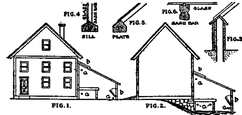
DETAILS FOR SMALL GREENHOUSES
