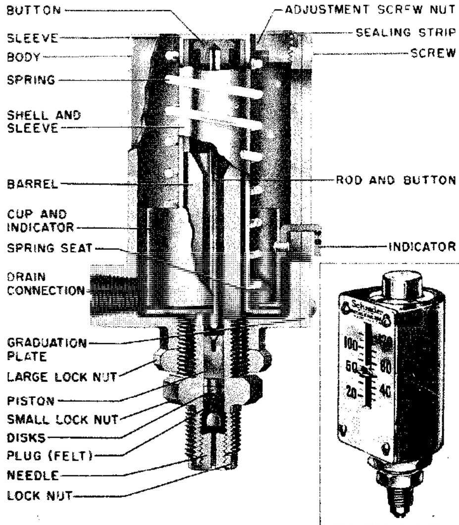
Figure 9-5.—The Schrader gage.
