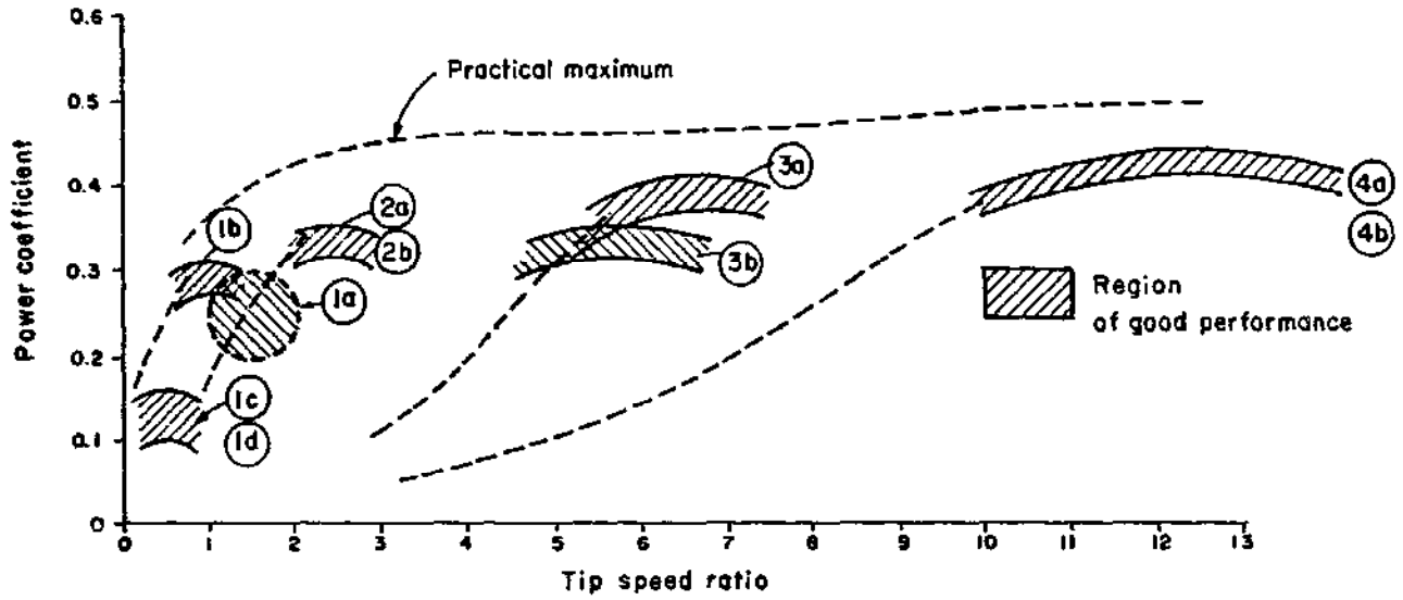
Figure 2. Power coefficient
