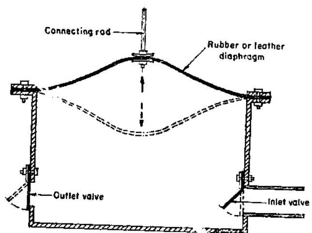
Figure 26. Diaphragm-type water pump
