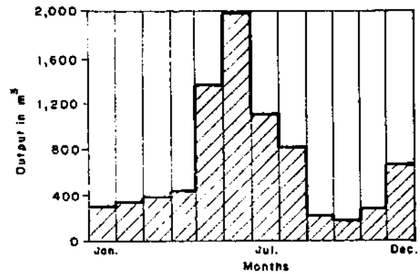
Figure 6. Monthly output of water per wind pump
