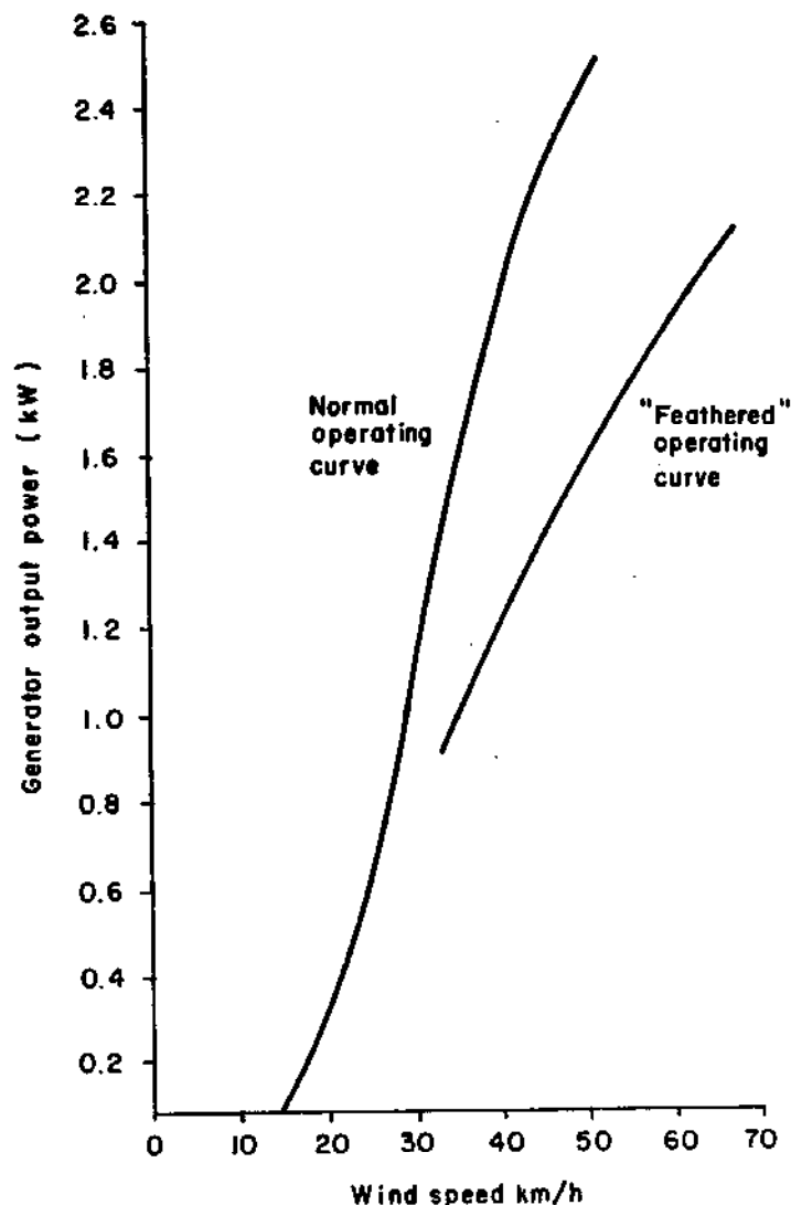
Figure 1. Characteristics of modified Dunlite generator
