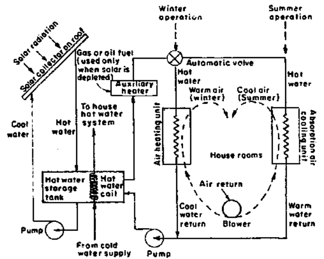
Figure 8. Residential heating and cooling
