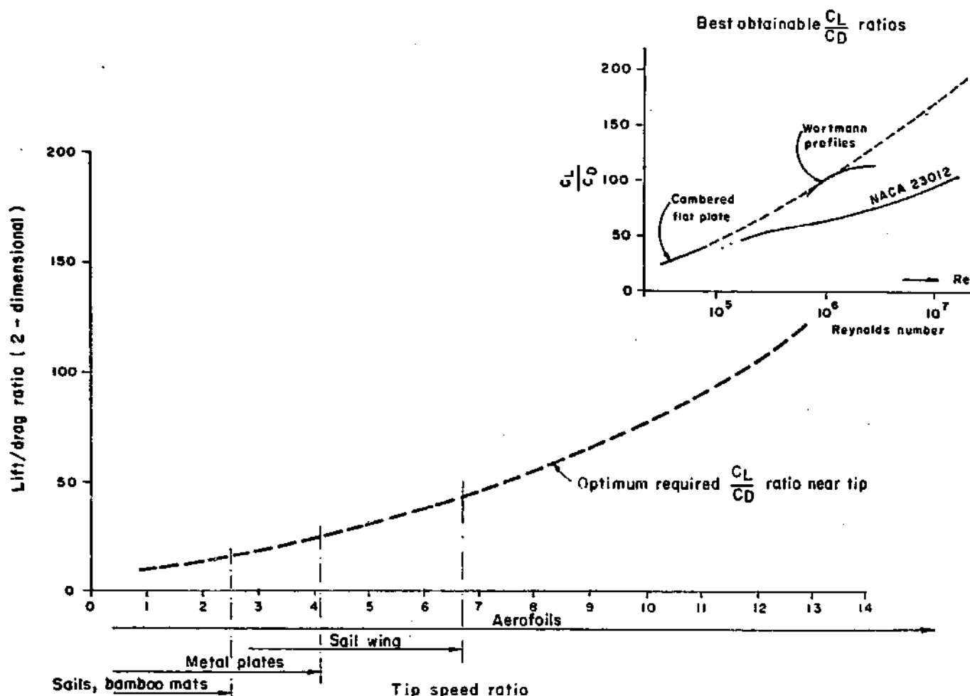
Figure 6. Lift/drag ratio
