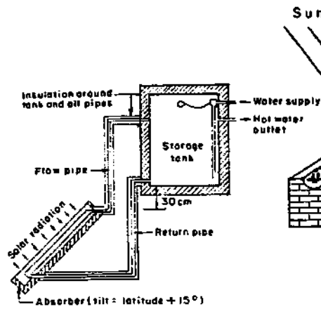
Figure 1. Domestic solar water heater
